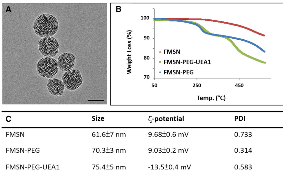
Figure 2. (A) TEM of FMSNs. Scale bar: 50 nm. (B) Thermogravimetric analysis of FMSN, FMSN-PEG and FMSN-PEG-UEA1. (C) Dynamic light scattering and zeta-potential measurements of pre/post UEA1-labeled FMSNs.
