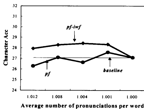
Fig.2 Character accuracy for count-based pruning with pf and pf-iwf ranking respectively.
