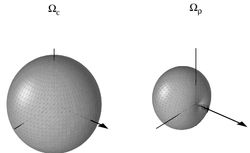
Figure 2. Perspective plots of the acoustic wave scattering coefficients \Omega_c (left) and \Omega_\rho (right). The orthonormal axes are centred upon the scatterer \mathbf{x} ; arrows denote the direction of the incoming wave vector \hat{\mathbf{k}}' .
