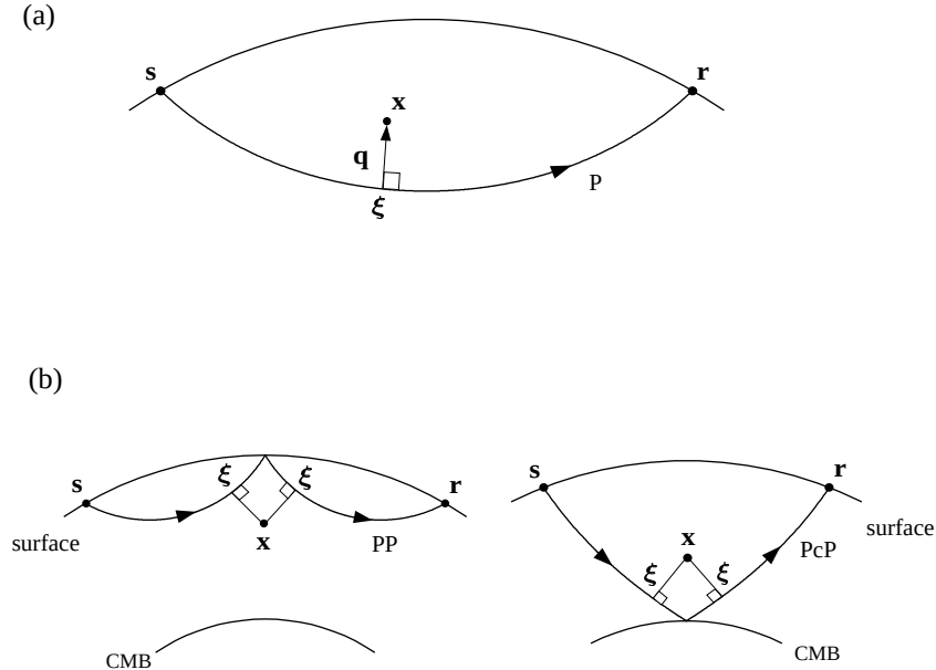
Figure 3. (a) In the paraxial approximation, every scatterer \mathbf{x} is perpendicularly projected onto the nearest point \xi on the central geometrical ray from the source \mathbf{s} to the receiver \mathbf{r} . The difference vector is \mathbf{q} = \mathbf{x} - \xi . (b) In many circumstances, including the two illustrated here, a scatterer can be projected onto more than one paraxial point \xi . (Left) A scatterer in the vicinity of the surface reflection point of a PP wave. (Right) A scatterer in the vicinity of the core–mantle boundary (CMB) reflection point of a PcP wave.
