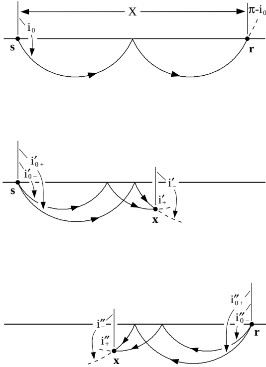
Figure A3. (Top) One-bounce PP ray between a surface source \mathbf{s} and receiver \mathbf{r} . The surface reflection occurs at the midpoint, \mathbf{x}_b = (X/2, 0, 0) . (Middle) Two PP rays' can propagate between a surface source \mathbf{s} and an arbitrary scatterer \mathbf{x} . The shallower of these, with take-off angle i'_{0-} and arrival angle i'_- , has passed through the PP caustic x^2 + y^2 - 8z(z+2h) = 0 on its second leg before arriving at \mathbf{x} , and has M' = 1 , whereas the steeper one, with take-off angle i'_{0+} and arrival angle i'_+ , has not yet passed through the caustic, and has M' = 0 . The two rays' merge and arrive with a downward incidence angle, given by \cos i' = \cos i'_0/3 in the case of a scatterer on the caustic. The \pm labels in the above discussion are the same as those in eqs (A33)–(A34). (Bottom) There are likewise two backward PP rays'', with take-off angles i''_{0\pm} and arrival angles i''_{\pm} , from the receiver \mathbf{r} to an arbitrary scatterer \mathbf{x} . The receiver-to-source caustic is given by (X-x)^2 + y^2 - 8z(z+2h) = 0 .
