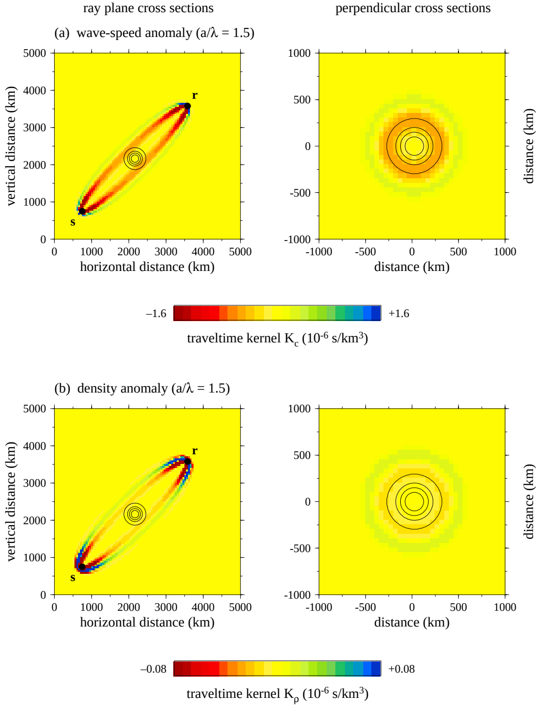
Figure 6. Cross-sections of the 3-D traveltime Fréchet kernels in a homogeneous background medium for a receiver at a distance \|\mathbf{r} - \mathbf{s}\| = 4000 km and an azimuth of 45^\circ . The characteristic period of the Gaussian-derivative wavelet \dot{m}(t) is \tau = 50 s. (a) Sensitivity K_c to a fractional change \delta c/c in wave speed. (b) Sensitivity K_\rho to a fractional change \delta \rho/\rho in density. Left panels show a ray-plane cross-section passing through the source \mathbf{s} and receiver \mathbf{r} ; right panels show a path-perpendicular cross-section, through the source–receiver midpoint. Circular contours show the location and size of a Case 1 or Case 4 anomaly. The outer circle, of radius a = 1.5 \lambda , is where the smooth, cosine-bell perturbation (36) or (37) vanishes.
