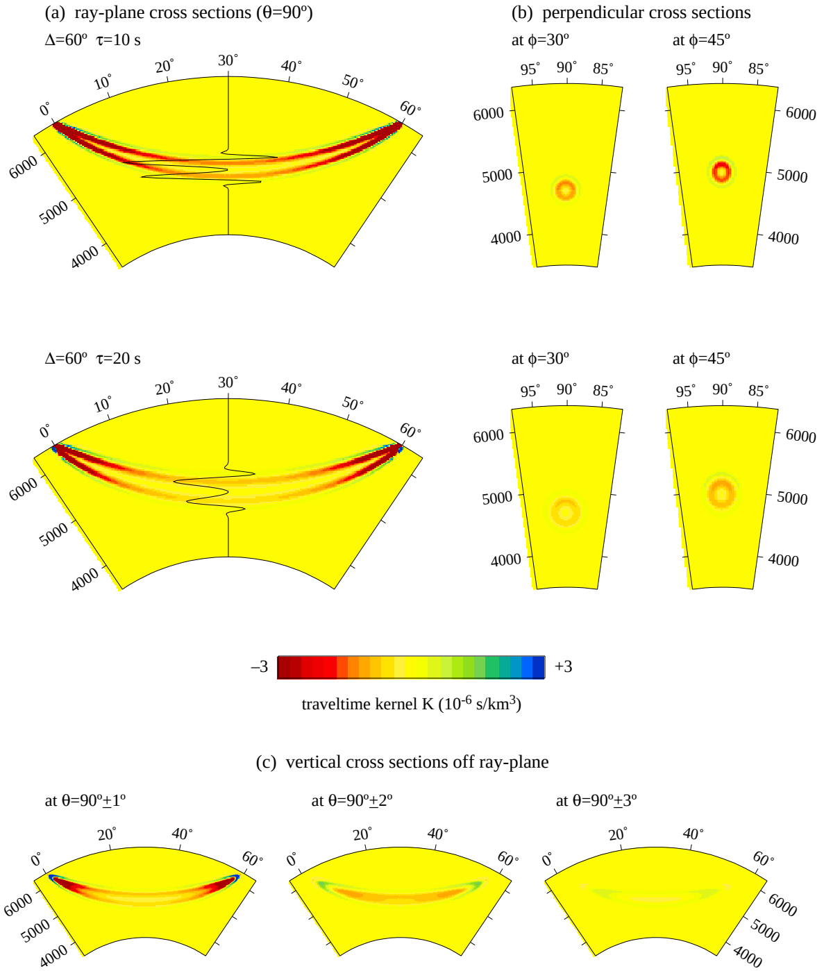
Figure 15. 2-D cross-sections through the 3-D paraxial Fréchet kernel K for a teleseismic P wave at an epicentral distance \Delta = 60^\circ . Compare with the corresponding views of the ‘exact’ kernel K_c in Fig. 12.
