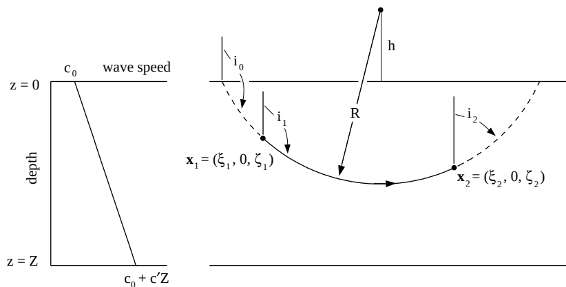
Figure A1. (Left) Flat-earth model with a constant-gradient wave speed c(z)=c_0+c'z in the depth interval 0 \leq z \leq Z . (Right) Every direct ray between two points \xi_1=(\xi_1, 0, \zeta_1) and \xi_2=(\xi_2, 0, \zeta_2) within such an earth model is a segment of a circle. The height h of the centre above the surface and the radius R are defined in the text.
