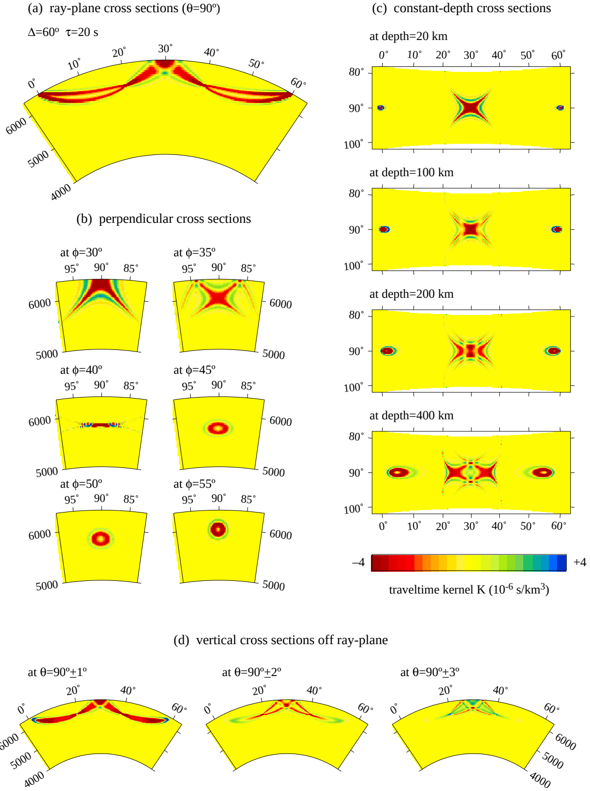
Figure 16. 2-D cross-sections through the 3-D paraxial Fréchet kernel K for a PP wave at an epicentral distance \Delta=60^\circ . Compare with the corresponding views of the ‘exact’ kernel K_e in Fig. 13.
