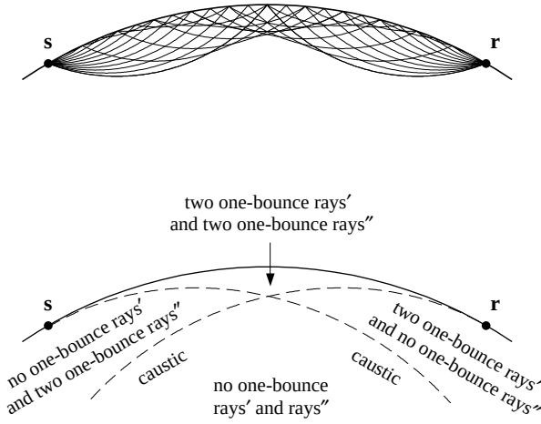
Figure 10. (Top) Family of PP rays shot from a surface source s and receiver r . The source-to-receiver and receiver-to-source caustics are the loci where adjacent rays cross. (Bottom) Dashed lines tangent to the surface of the earth at s and r denote these two bowl-shaped caustic surfaces. The caustics subdivide the space of single scatterers x into four regions, as shown.
