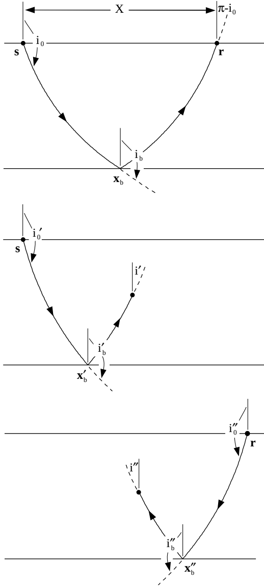
Figure A4. (Top) PcP ray between a surface source s and receiver r showing the take-off and arrival angles i_0 and \pi - i_0 and the incidence angle i_b upon reflection off the core–mantle boundary at \mathbf{x}_b = (X/2, 0, Z) . (Middle) Forward PcP ray' with one core–mantle boundary reflection between the source s and an arbitrary scatterer \mathbf{x} = (x, y, z) . (Bottom) Backward PcP ray'' between the receiver s and \mathbf{x} .
