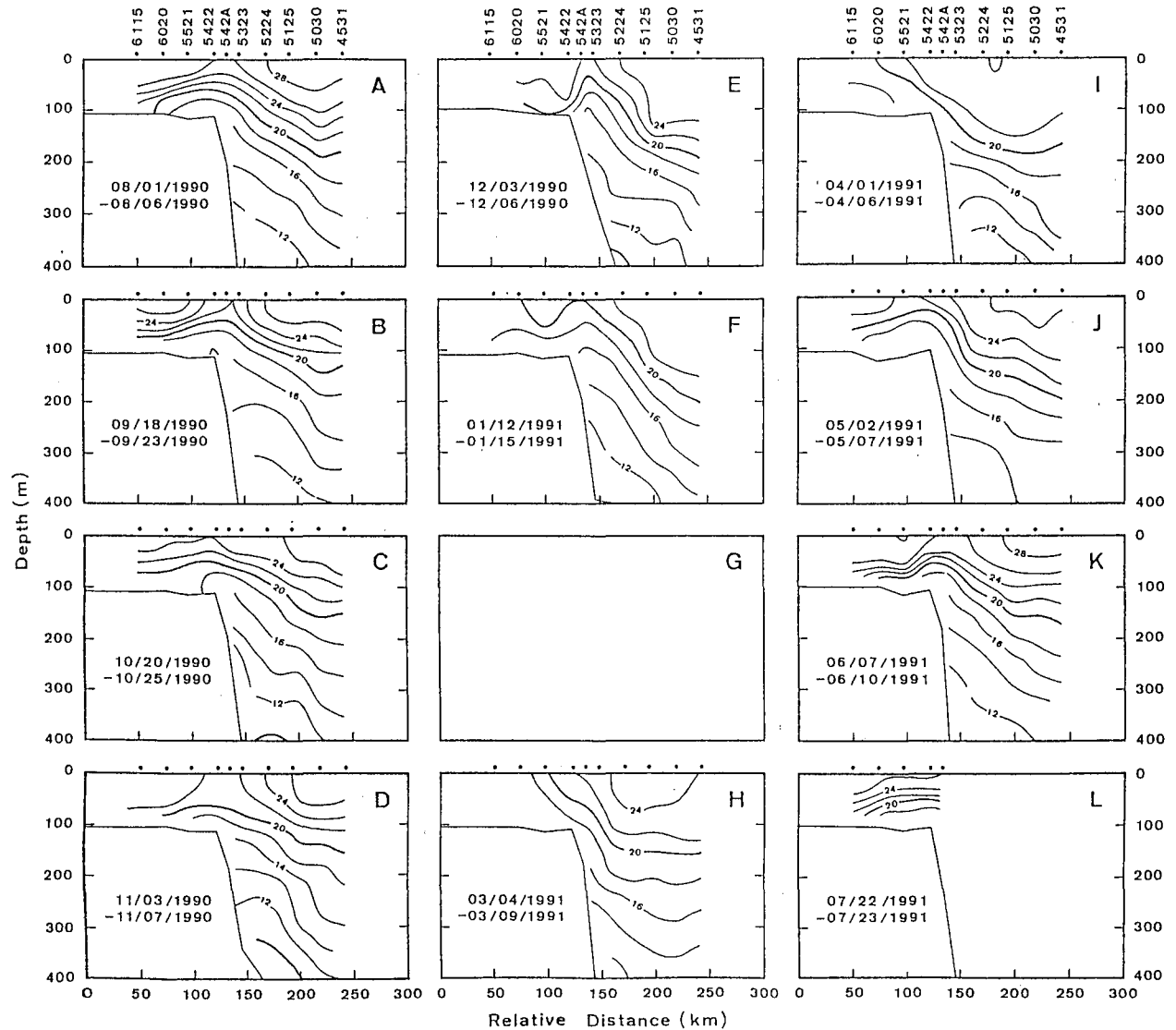
Fig. 2. The temperature sections along transect B (Fig. 1) during monthly cruises from August 1990 to July 1991.
