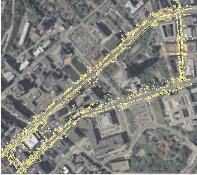
Fig. 36. The reconstructed map is overlaid on an aerial photo.
