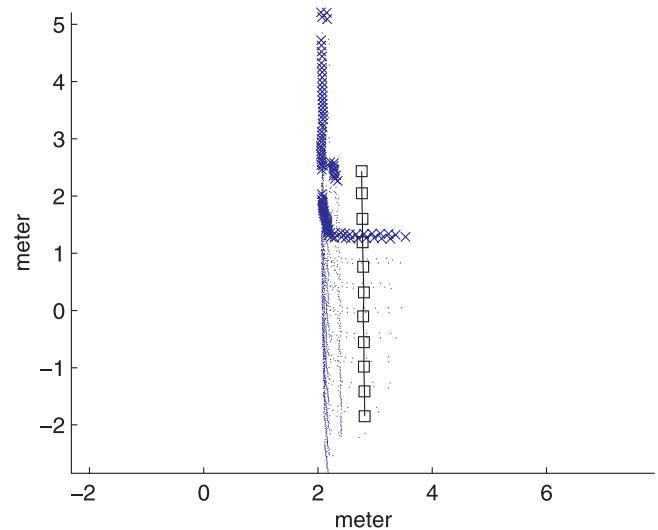
Fig. 16. Registration results of the example in Figure 15 using the SCRIM algorithm. The states are indicated by Box ( \square ), and the final scan points are indicated by \times .
