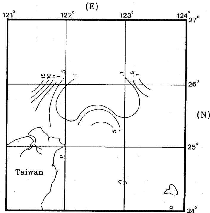
Fig. 5. Isoleth diagram of fish egg measured in \text{g}/1,000 \text{ m}^3 . A higher density contour toward the East China sea was found. In addition, A dilution effect of the Kuroshio was apparent around 26^\circ \text{ N}, 122^\circ 30' \text{ E} .
