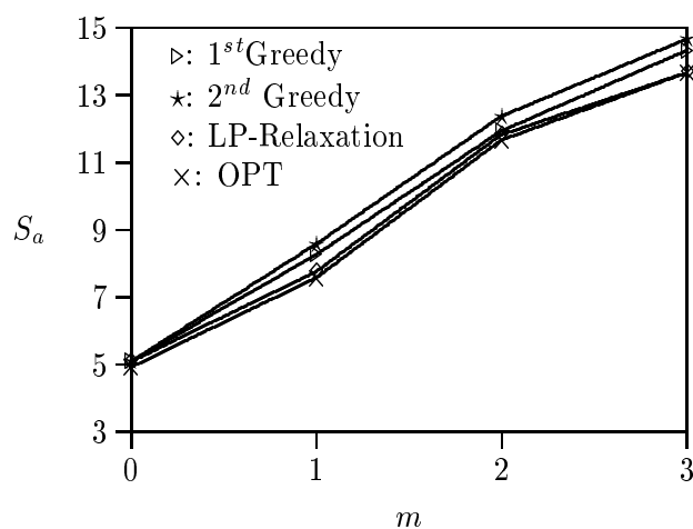
(c) Hudson's data (20 SNPs)
