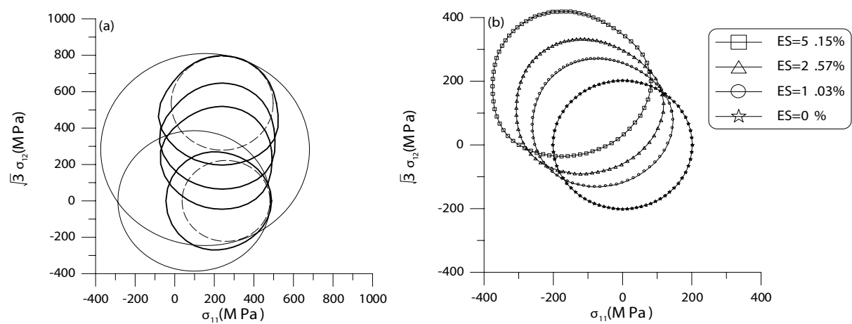
Figure 13. A theoretical prediction of yield surfaces with an equivalent strain offset with 0.001.
