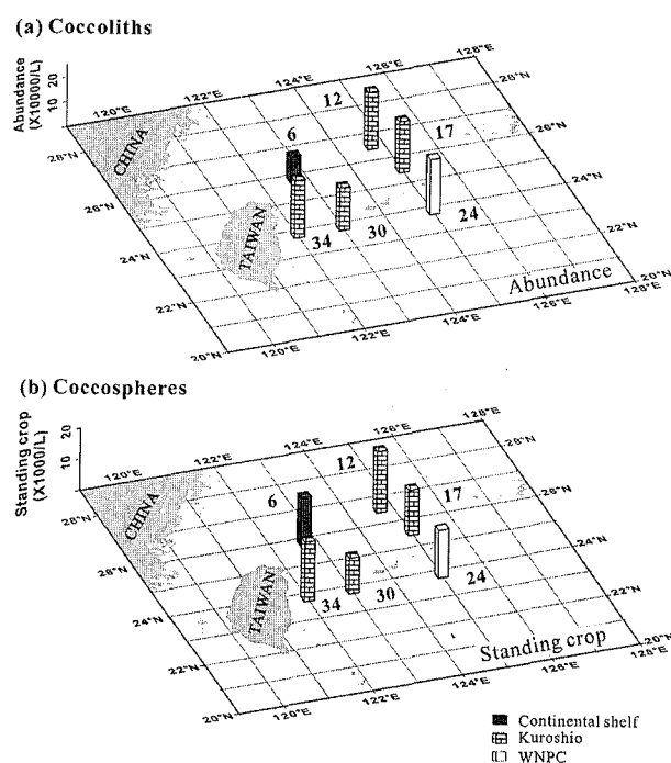
Figure 5. Geographic distribution of abundance of coccoliths (a), and standing crops of coccospheres (b). The Kuroshio path shows the highest abundance of coccoliths and coccospheres.
