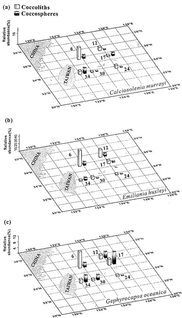
Figure 6. Geographic pattern of the relative abundances of Calciosolenia murrayi (a), Emiliania huxleyi (b) and Gephyrocapsa oceanica (c) in the studied area. These species distributed mainly on the continental shelf of the East China Sea.
