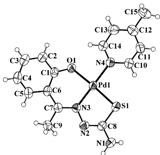
Fig. 3 Structure of the [\text{Pd}(\text{L}^2)(\text{pic})] complex drawn at the 50% probability level.
