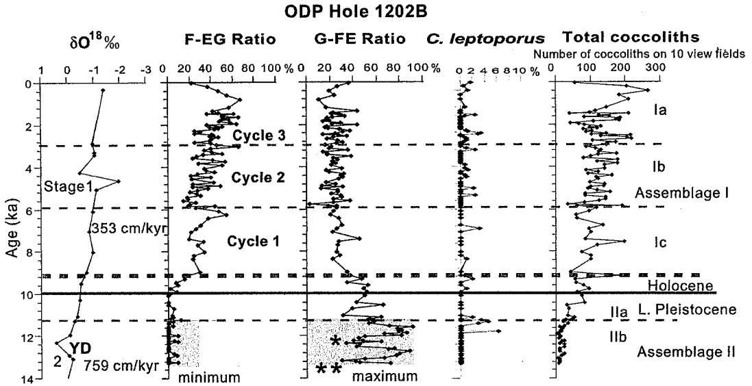
Fig. 6. Down-hole variation of the F-EG ratio, G-FE ratio and \delta^{18}\text{O} of N. dutertrei at ODP Hole 1202B plotted against age. In addition, relative abundance of a warm water species, C. leptoporus , and total coccoliths were plotted. The star symbols mark two low values of G-FE ratio (See explanation in the text). 353 \text{ cm ky}^{-1} and 759 \text{ cm ky}^{-1} are sedimentation rates for the Holocene and the Upper Pleistocene interval studied.
