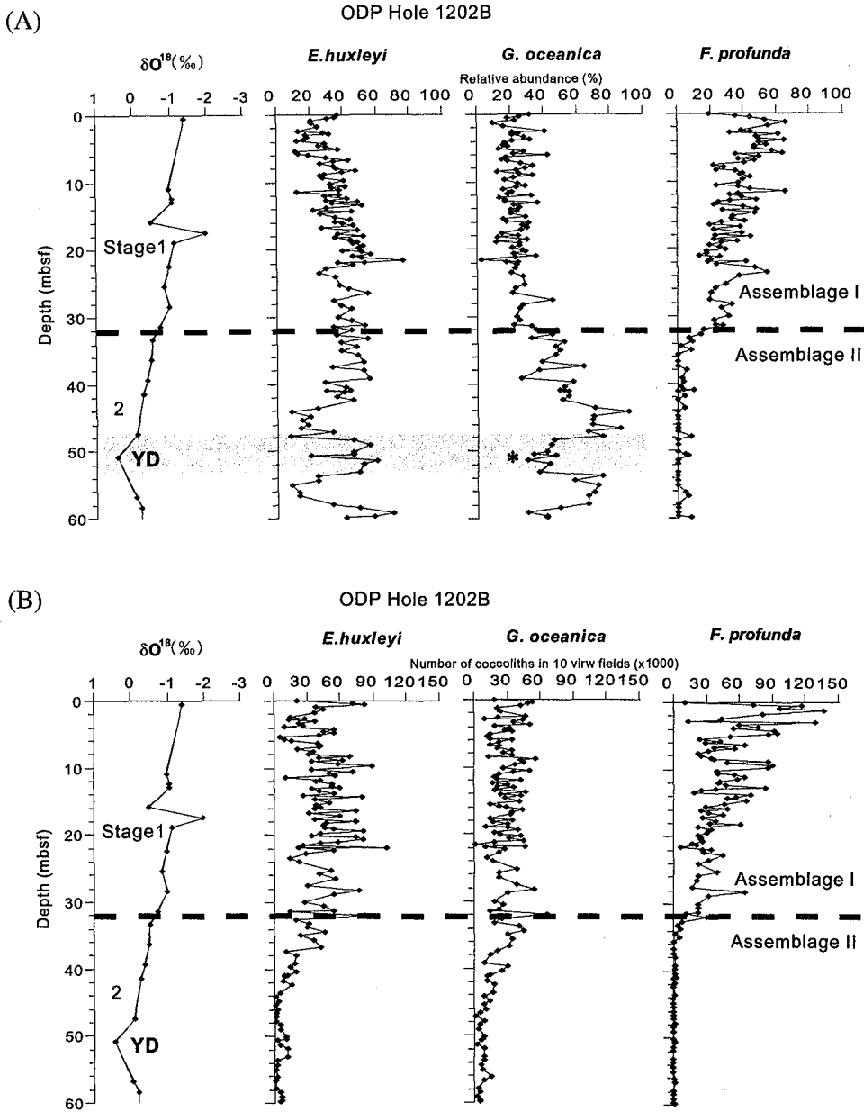
Fig. 5. Down-hole variations of relative abundance (A) and absolute abundance (B) of 3 dominant species and \delta^{18}\text{O} of N. dutertrei at ODP Hole 1202B plotted against depths. YD represents the Younger Dryas event. The star symbol in (A) shows the warm water G. oceanica reduces production during the cold Younger Dryas event (See text).
