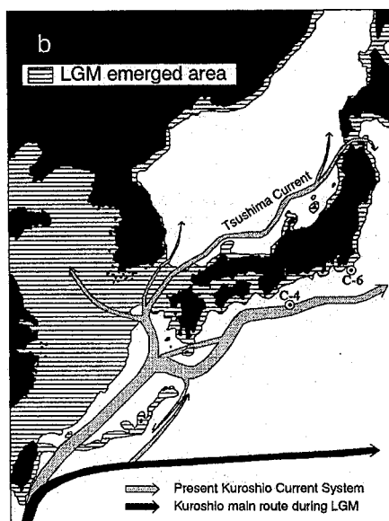
Fig. 2. Main route positions of the Kuroshio Current at the present and during the last glacial maximum suggested by Ujiie and Ujiie (1999).
