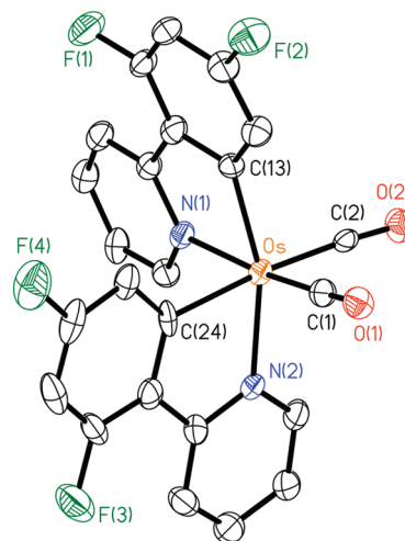
Figure 2. ORTEP drawing of complex 2b with thermal ellipsoids shown at the 50% probability level. Selected distances (Å): Os–C(1) = 1.865(11), Os–C(2) = 1.940(12), Os–C(13) = 2.078(9), Os–C(24) = 2.129(9), Os–N(1) = 2.142(7), Os–N(2) = 2.159(8), O(1)–C(1) = 1.155(11), O(2)–C(2) = 1.137(11).
