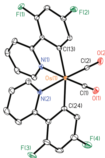
Figure 1. ORTEP drawing of complex 2a with thermal ellipsoids shown at the 50% probability level. Selected distances (Å): Os(1)–C(1) = 1.864(4), Os(1)–C(2) = 1.859(4), Os(1)–C(13) = 2.116(3), Os(1)–C(24) = 2.110(3), Os(1)–N(1) = 2.145(3), Os(1)–N(2) = 2.146(3), O(1)–C(1) = 1.145(4), O(2)–C(2) = 1.158(4).
