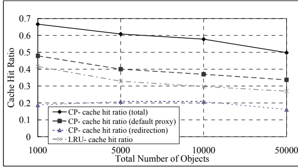
Figure 4. Total Number of Objects vs. Cache Hit Ratio (Cluster Size = 6, Cache Size Per Proxy = 50)
