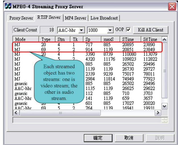
Figure 2. A snapshot of MPEG-4 streaming services.
