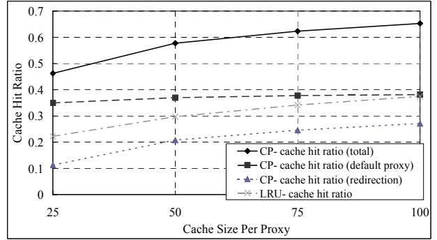
Figure 6. Cache Size Per Proxy vs. Cache Hit Ratio (Total Number of Objects = 10000, Cluster Size = 6)
