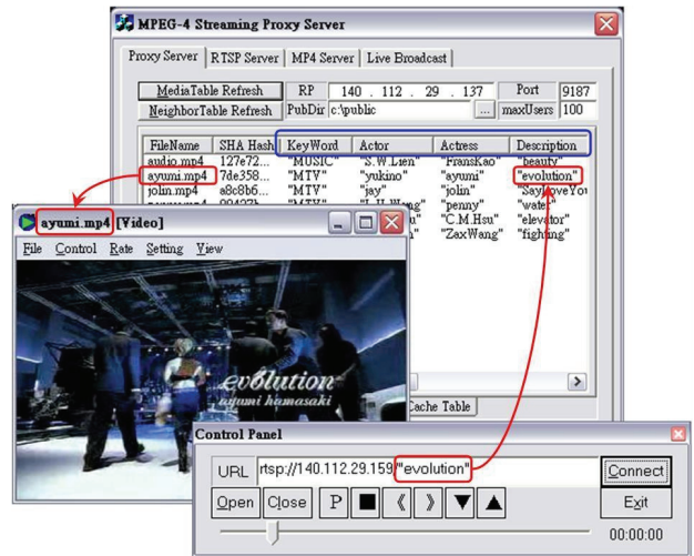
Figure 3. An example of request by using MPEG-7 content description is shown. Information items enclosed by the blue line are MPEG-7 content descriptions of a multimedia object.
