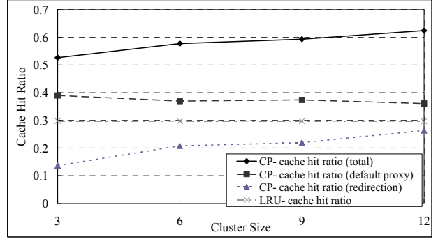
Figure 5. Cluster Size vs. Cache Hit Ratio (Total Number of Objects = 10000, Cache Size Per Proxy = 50 objects)
