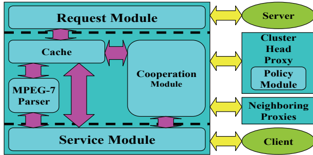
Figure 1. The working modules in our streaming proxies: the internal interactions between these modules and the external interactions with servers, clients, neighboring proxies and the cluster head proxy.
