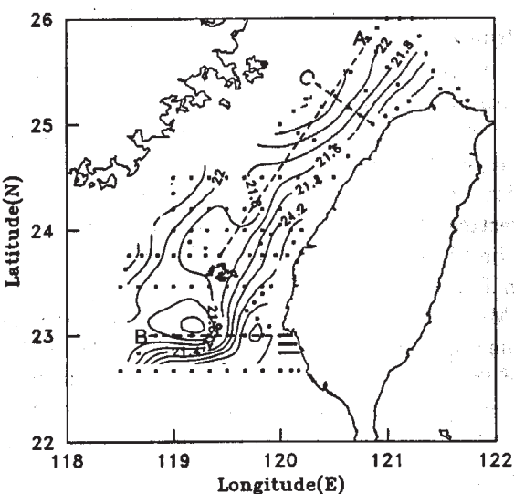
(a) 1988/9/1-6 Sigma- t at 10m depth
