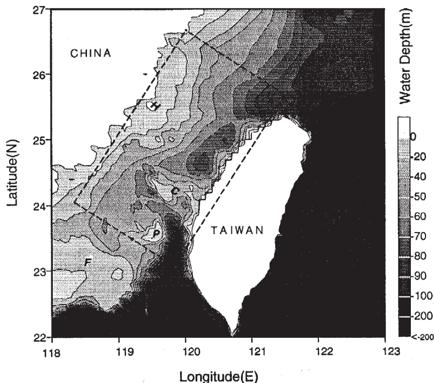
Fig. 1. Bottom topography of the Taiwan Strait, in which F is the Formosa Banks, P is the Peng-hu Islands, PHC is the Peng-hu Channel, C is the Chang-yuen ridge and H is Hai-tang Island. The dashed rectangle is the computation domain.
