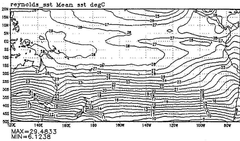
Fig-A2: Distribution of the Isotherm in 1983.
