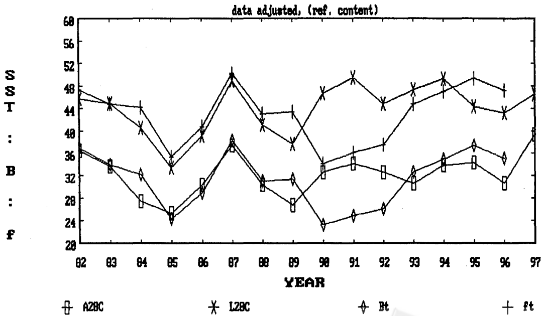
Fig. 5. SST index and Bt, ft.
