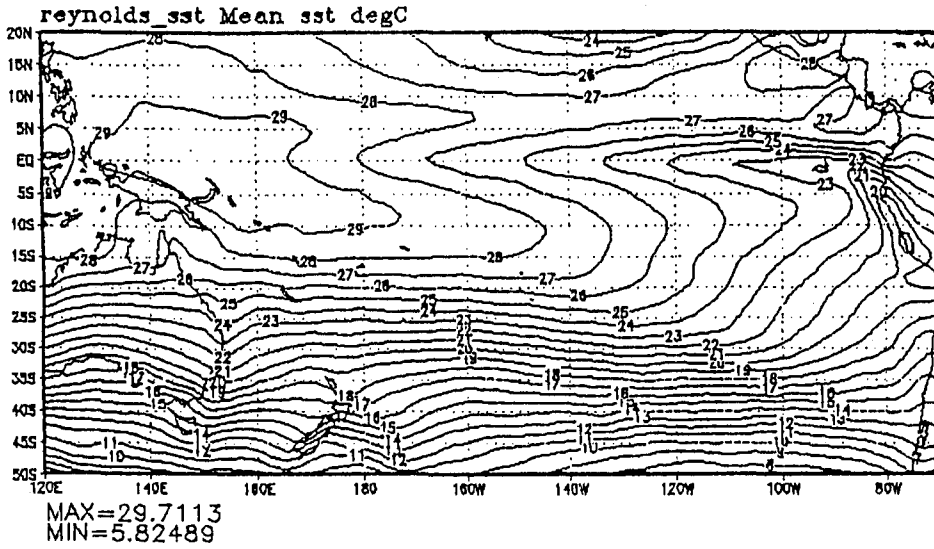
Fig-A4: Distribution of the Isotherm in 1985.
