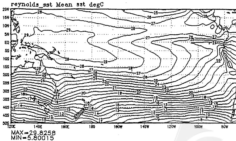
Fig-A5: Distribution of the Isotherm in 1986.
