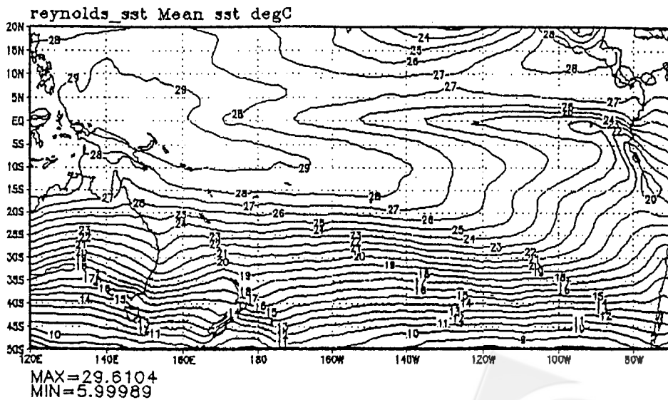
Fig-A3: Distribution of the Isotherm in 1984.
