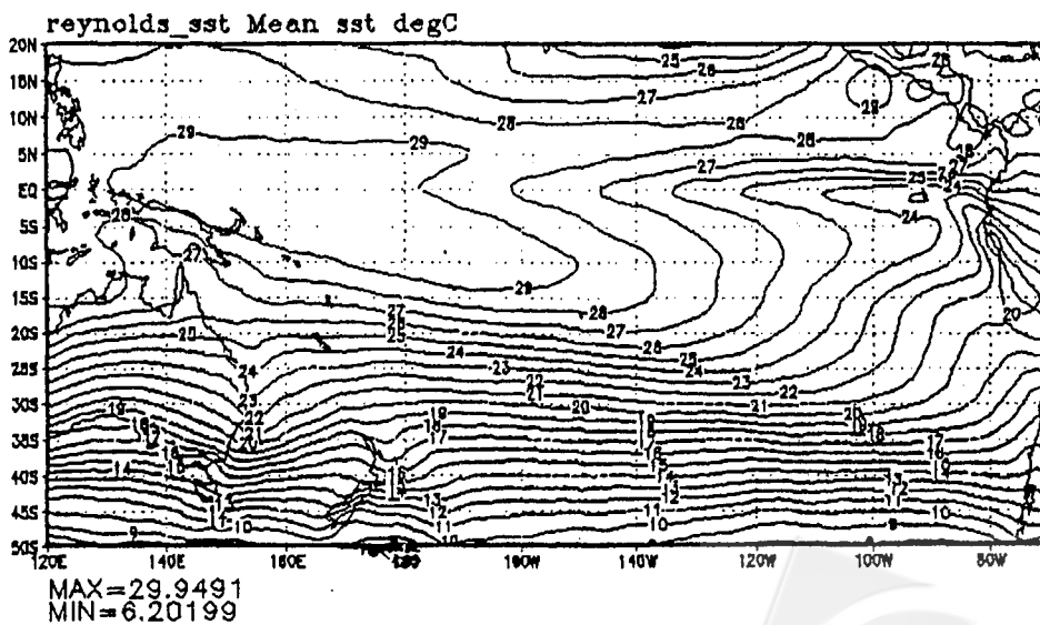
Fig-A13: Distribution of the Isotherm in 1994.
