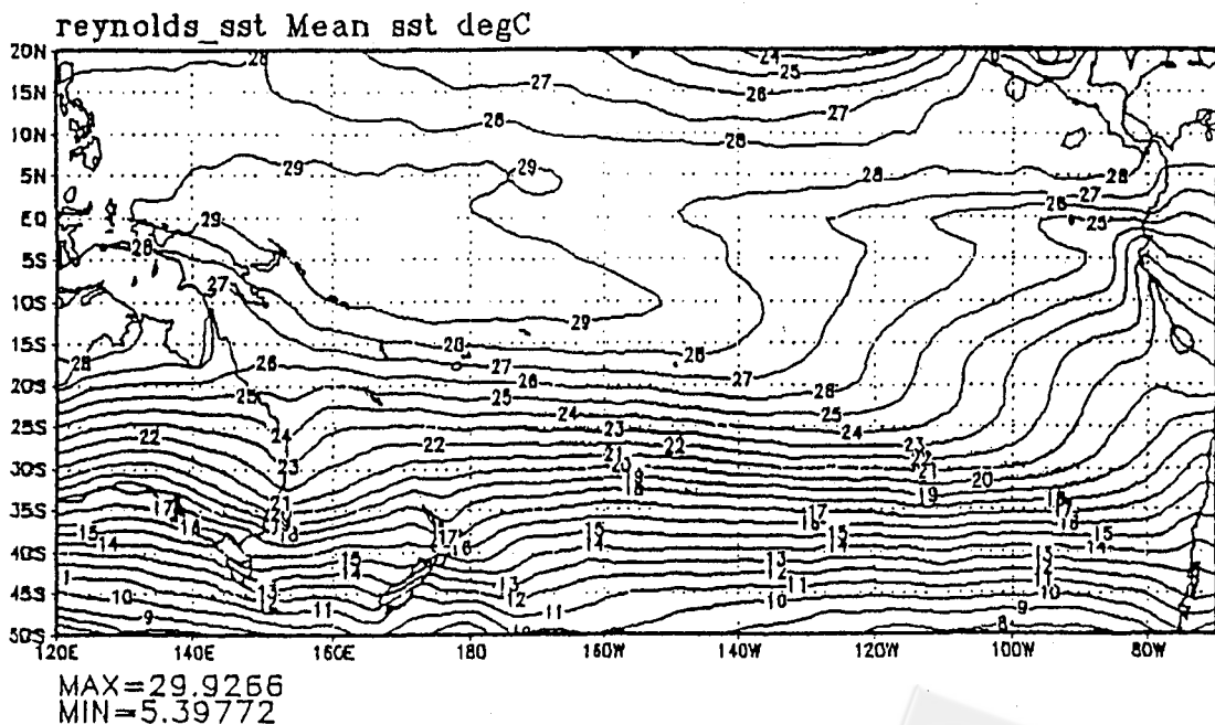
Fig-A1: Distribution of the Isotherm in 1982.
