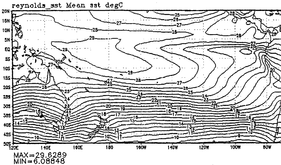
Fig-A12: Distribution of the Isotherm in 1993.
