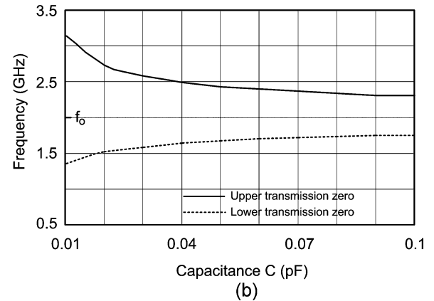
Fig. 6. (a) Simulated responses of the filter circuit model (Fig. 2) for various values of C . (b) Curves to relate the cross-coupled-induced transmission-zero frequencies to the values of C . ( \theta_1 = 51.8^\circ , \theta_2 = 35^\circ , \theta_3 = 61.8^\circ , \theta_4 = 25^\circ , L = 0.22 nH, Z_{oe1} = 69 \Omega , Z_{oo1} = 39 \Omega , Z_{oe3} = 66.3 \Omega , Z_{oo3} = 39.8 \Omega .)
