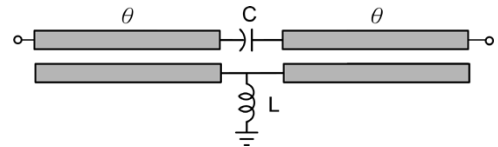
Fig. 1. Circuit model of second-order coupled-line filter in [14]–[16].
