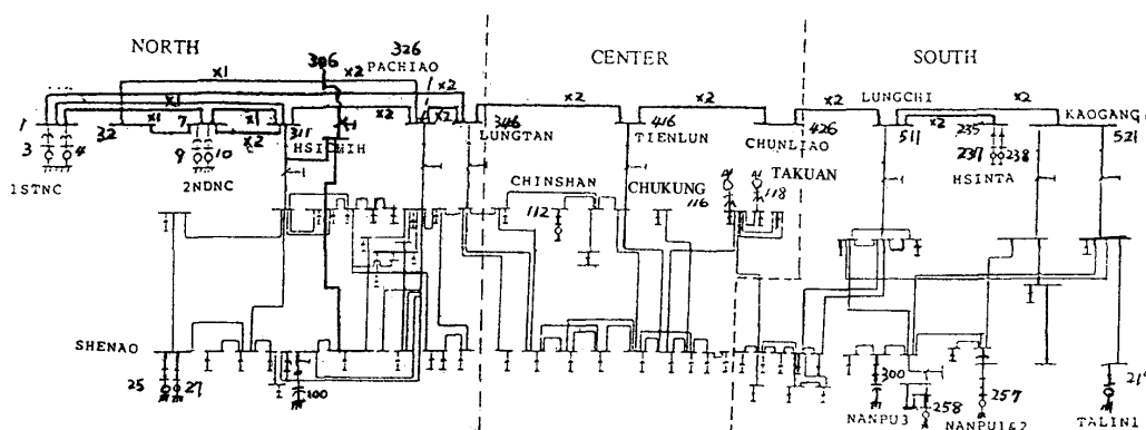
Fig. 2 One-line diagram of Taiwan power system
