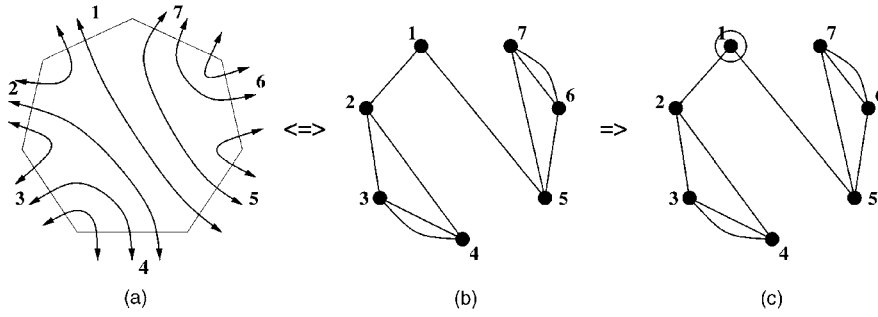
Fig. 1. Example of RRV, (7, 3)-GR and (7, 3)-PBGR. (a) Diagram of V_0 . (b) Graph representation of global routing of V_0 . (c) Corresponding (7, 3)-PBGR GR_0 .
