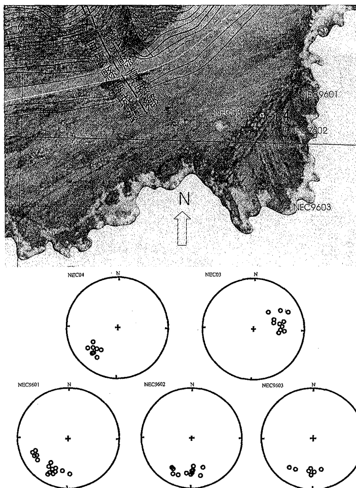
Fig. 4. The air-photograph at the 122 km area of the northeastern cross highway showing sampling site localities and stereo-net plot showing the tilt-corrected paleomagnetic results of the studied sites. Open circle in the stereo-net plot represents the negative inclination.
