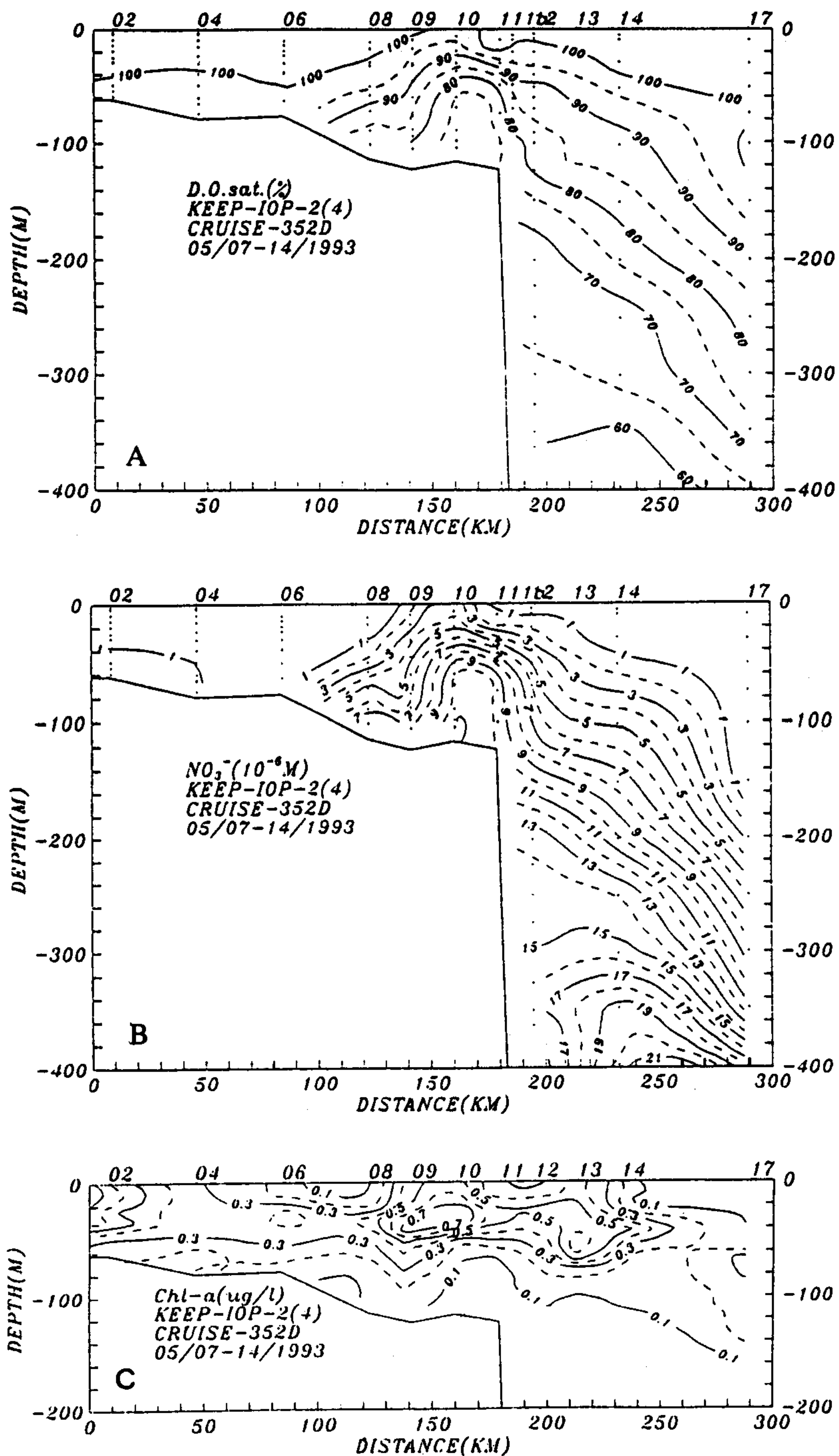
Fig. 4. Vertical distribution of some chemical parameters along the long transect observed on Cruise 352D. (A) Degree of oxygen saturation (%), (B) Nitrate ( \mu\text{M} ), and (C) Chlorophyll a ( \mu\text{g/L} ).
