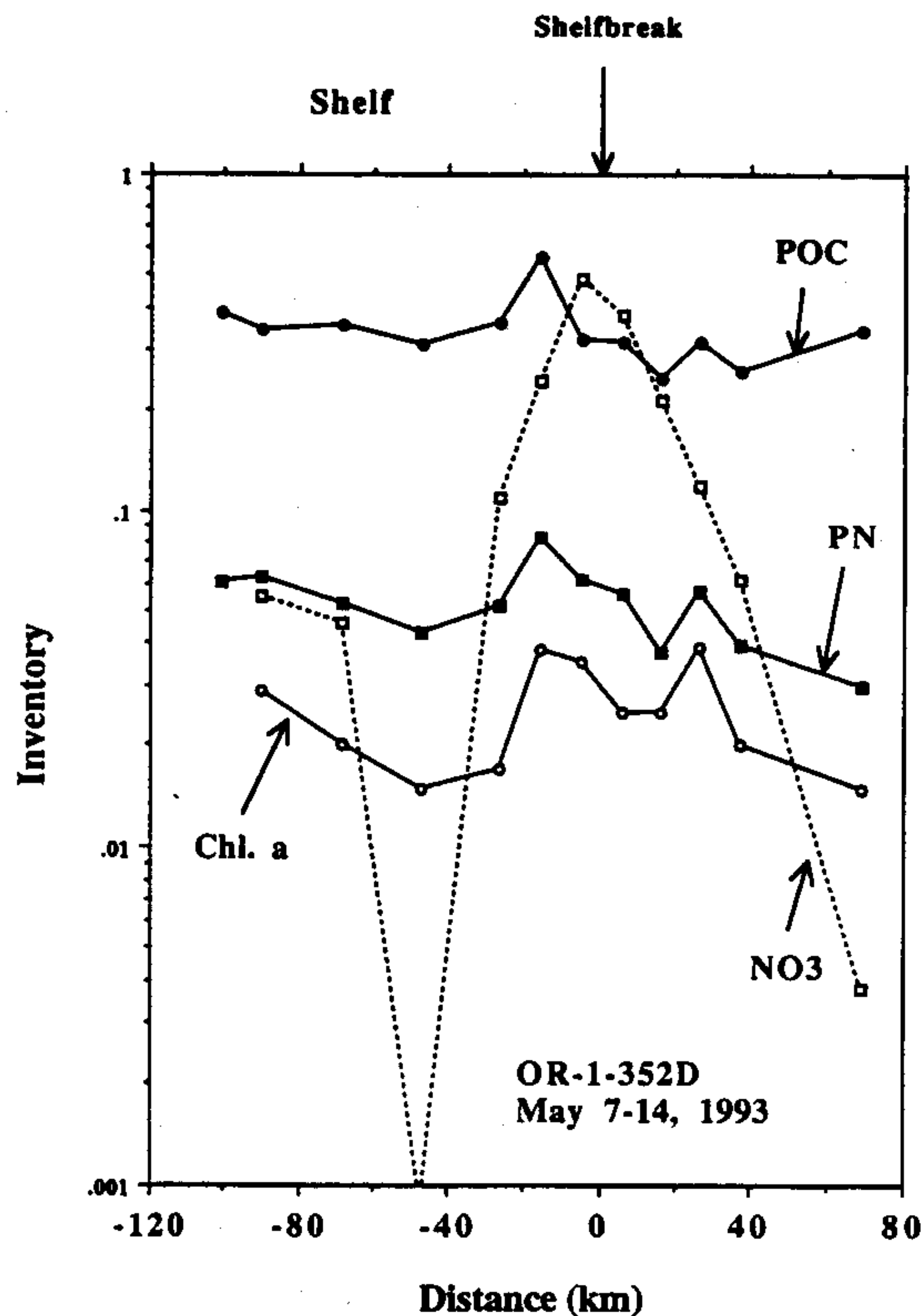
Fig. 12. The variation of chemical inventories, i.e., integrated quantities in the upper 70 m, along the long transect of Cruise 352D. The distance was measured with the shelf break set to zero. Dots and solid squares represent POC and PN, respectively. Open squares and circles represent nitrate and chlorophyll a , respectively. The units are in mole/m 2 except for chlorophyll a which is in g/m 2 .
