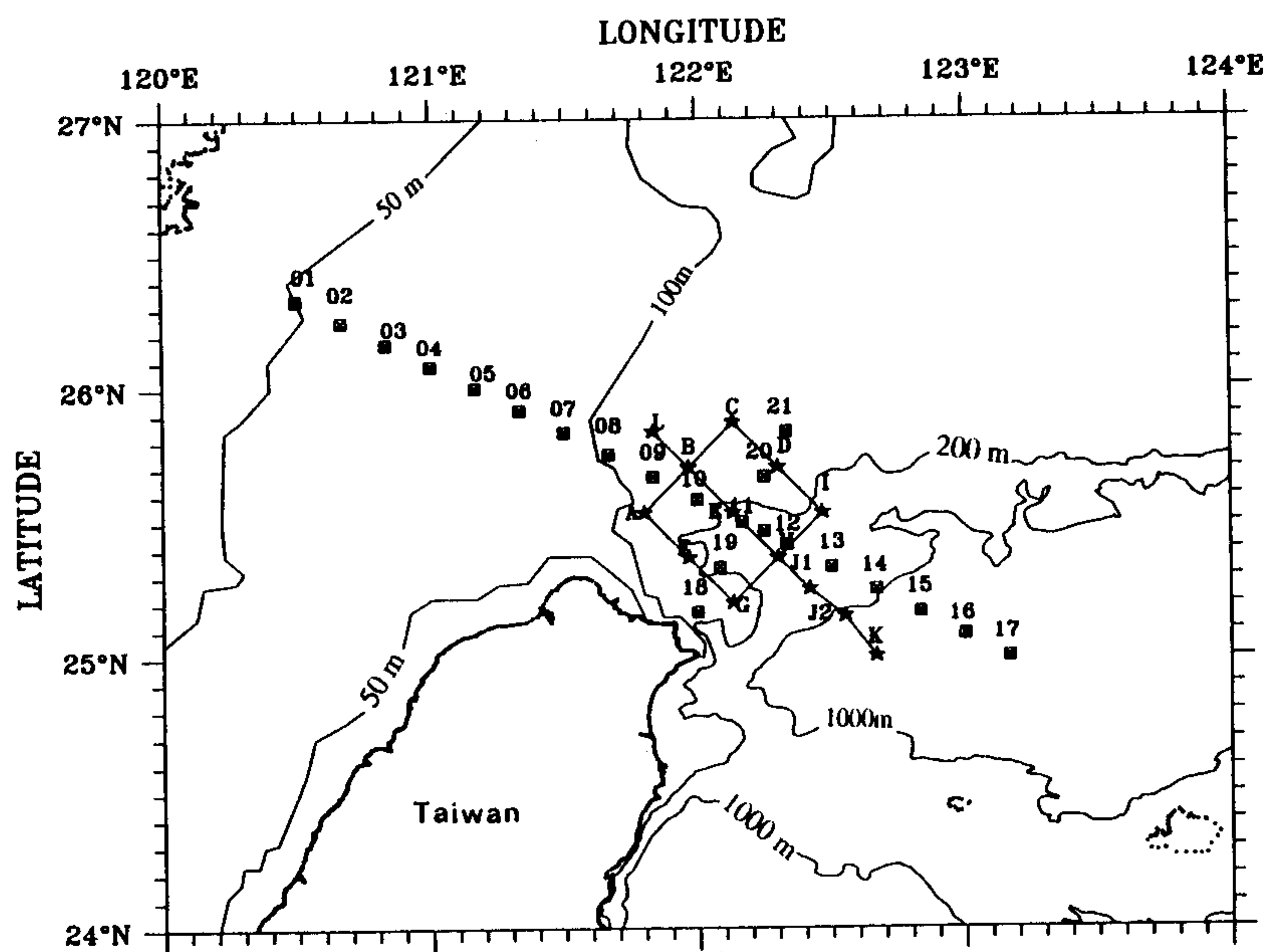
Fig. 1. The sampling stations in this study. Stations from Cruise 331B on Ocean Researcher I during October 4-9, 1992 are indicated by stars, and those from Cruise 352D during May 5-9, 1993 are indicated by squares. Station 11A, which is located midway between Stations 11 and 12, is not labeled to avoid an overlapping of labels.
