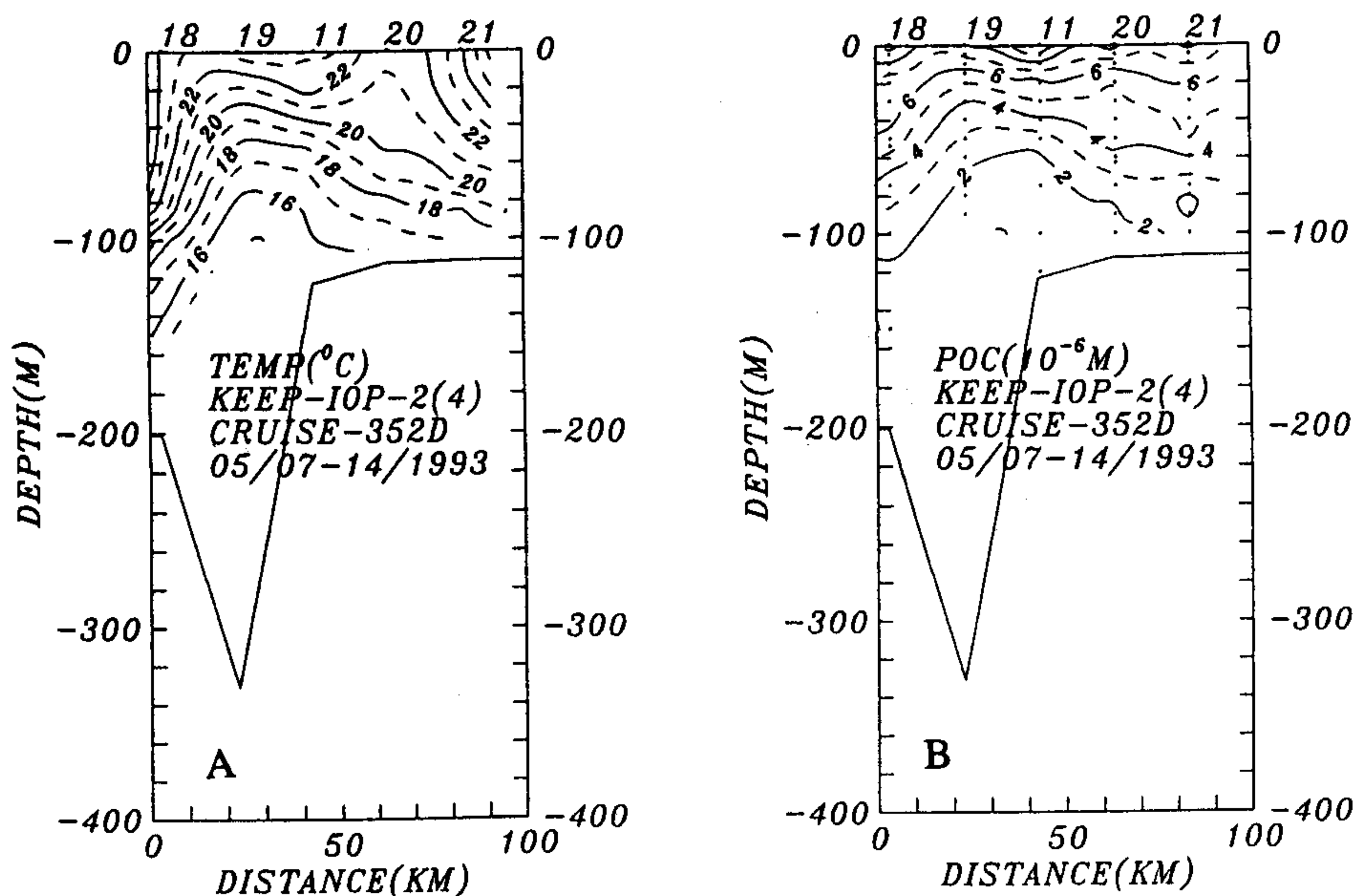
Fig. 6. Section contours for temperature (A) and POC (B) along the short transect of Cruise 352D.
