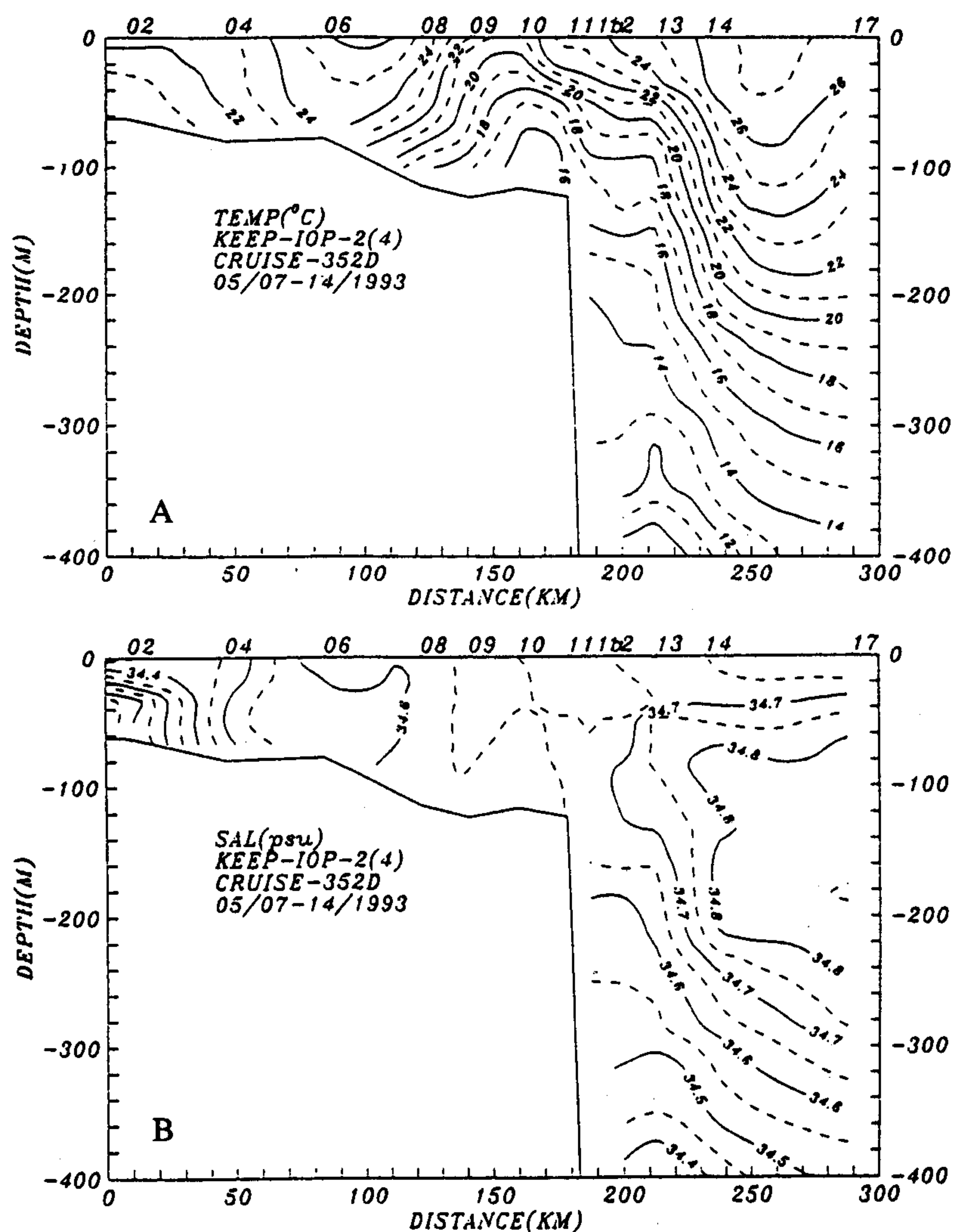
Fig. 2. The hydrographic sections for the upper 400 m obtained with CTD along the long transect on Cruise 352D. The localities of the stations are shown on top of the plots. (A) Temperature ( ^{\circ}\text{C} ), (B) Salinity (psu).
