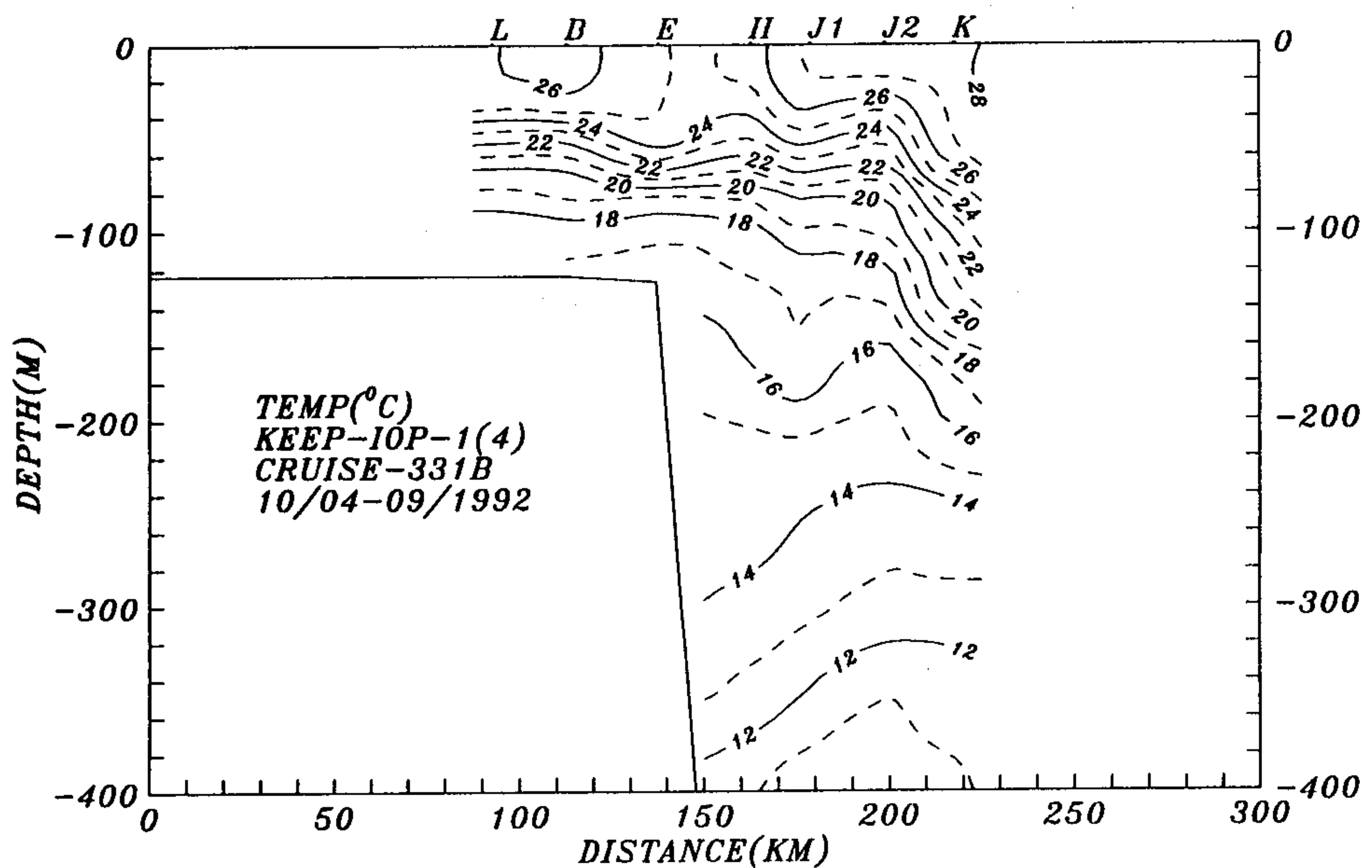
Fig. 7. The temperature section for the upper 400 m along the long transect of Cruise 331B.
