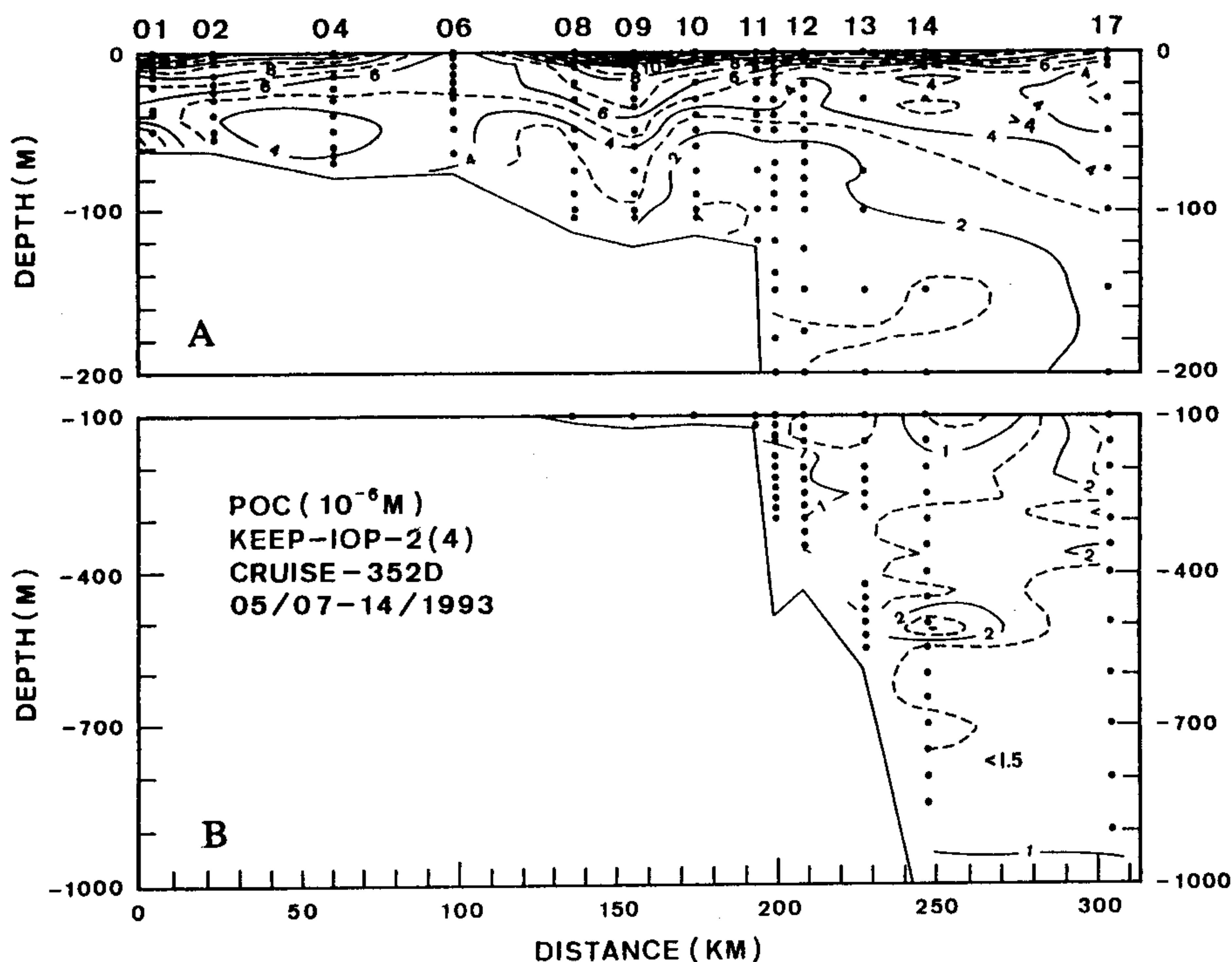
Fig. 5. The vertical distribution of POC along the long transect of Cruise 352D. (A) Section for the upper 200 m. The contour interval is 1 \mu\text{M} . (B) Section for depths from 100 to 1000 m. The contour interval is 0.5 \mu\text{M} .
