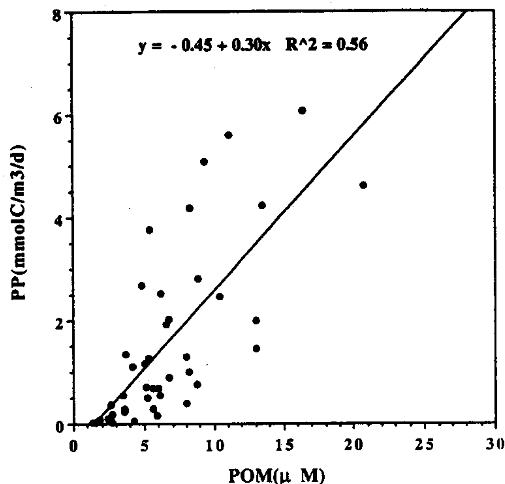
Fig. 11. The primary production versus POC concentration in the upwelling region.
