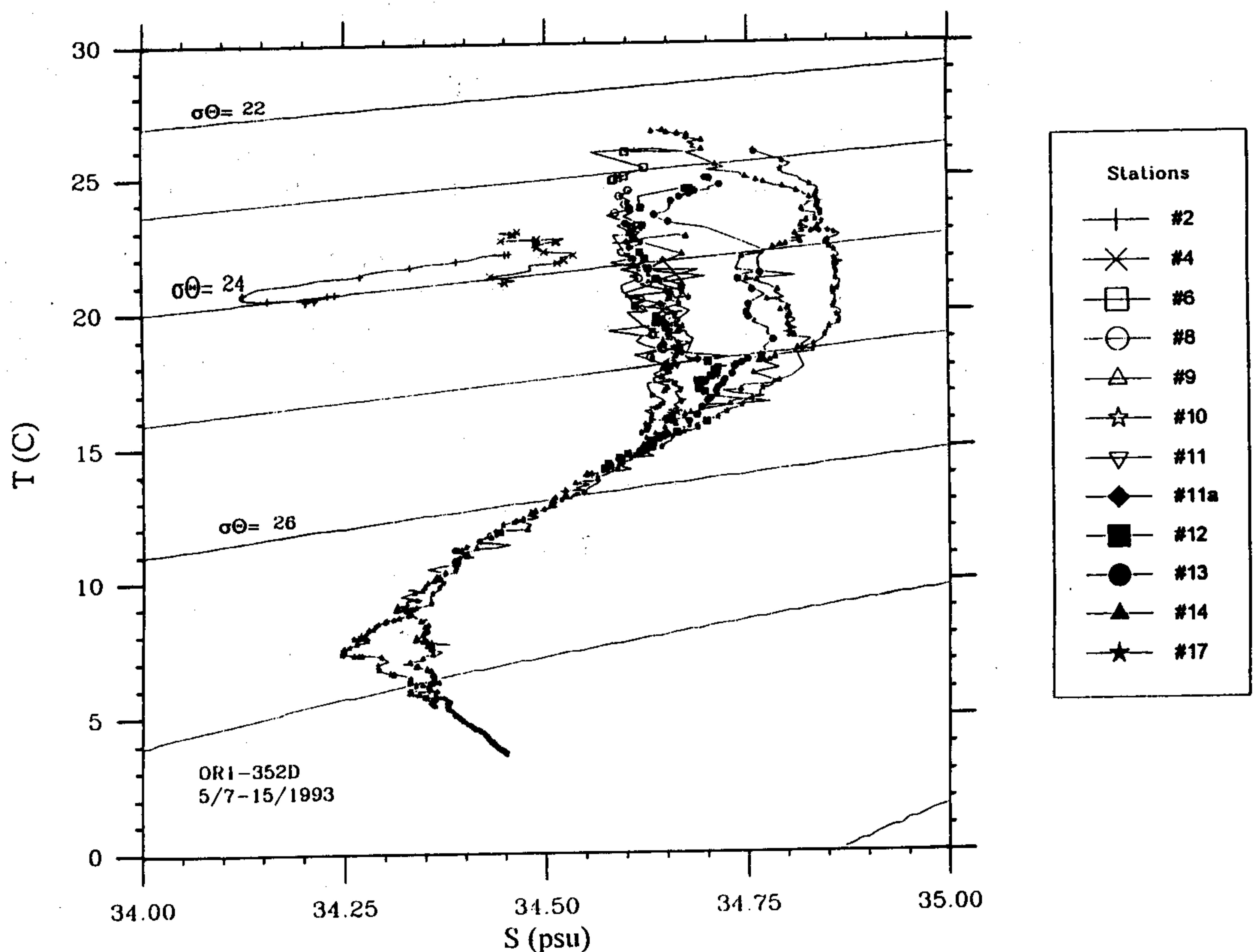
Fig. 3. The T-S diagram for Stations 2-17 on Cruise 352D.
