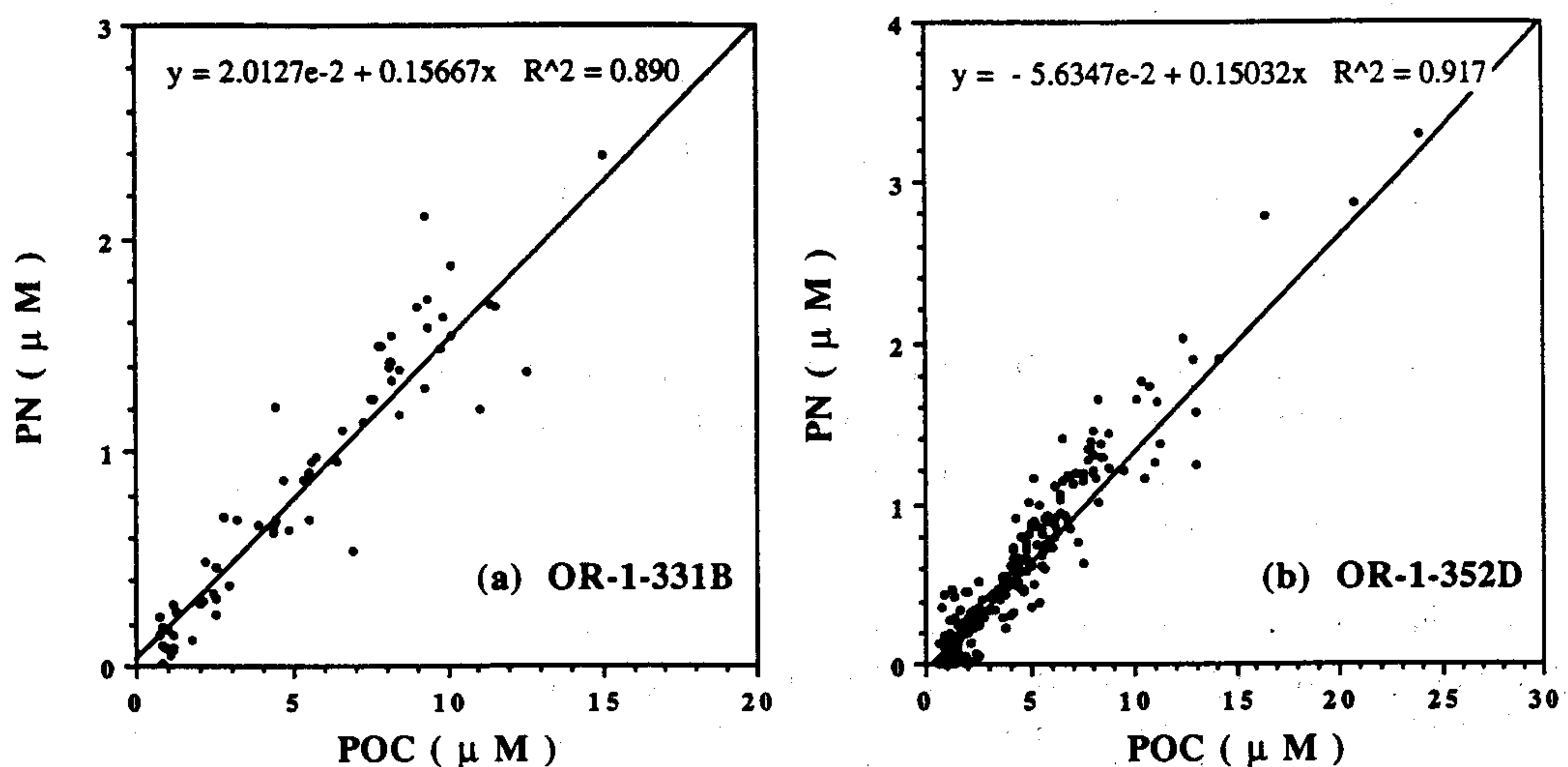
Fig. 9. The relationship between POC and PN. (a) Cruise 331B, (b) Cruise 352D.
