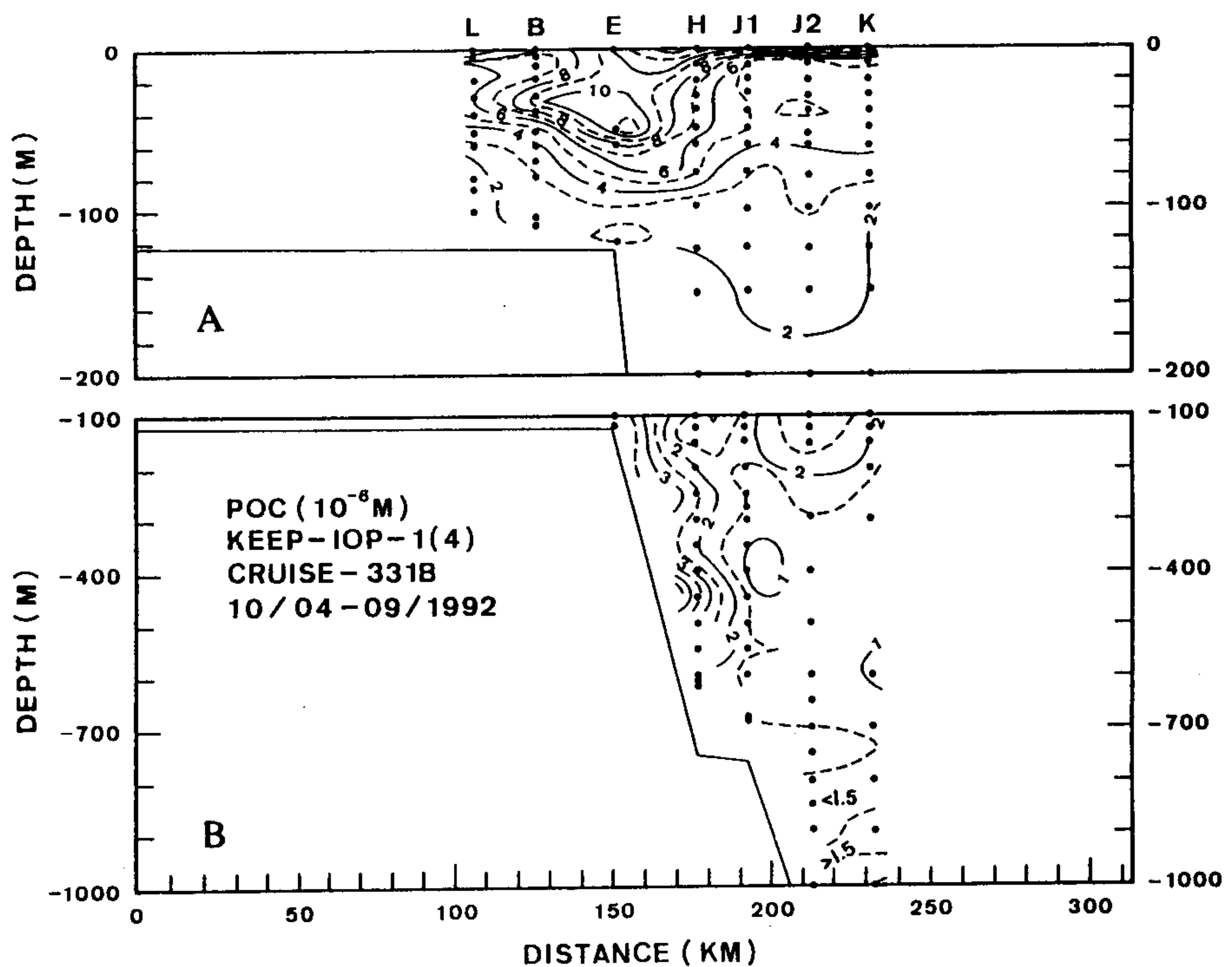
Fig. 8. The same as Fig. 5 except for Cruise 331B.
