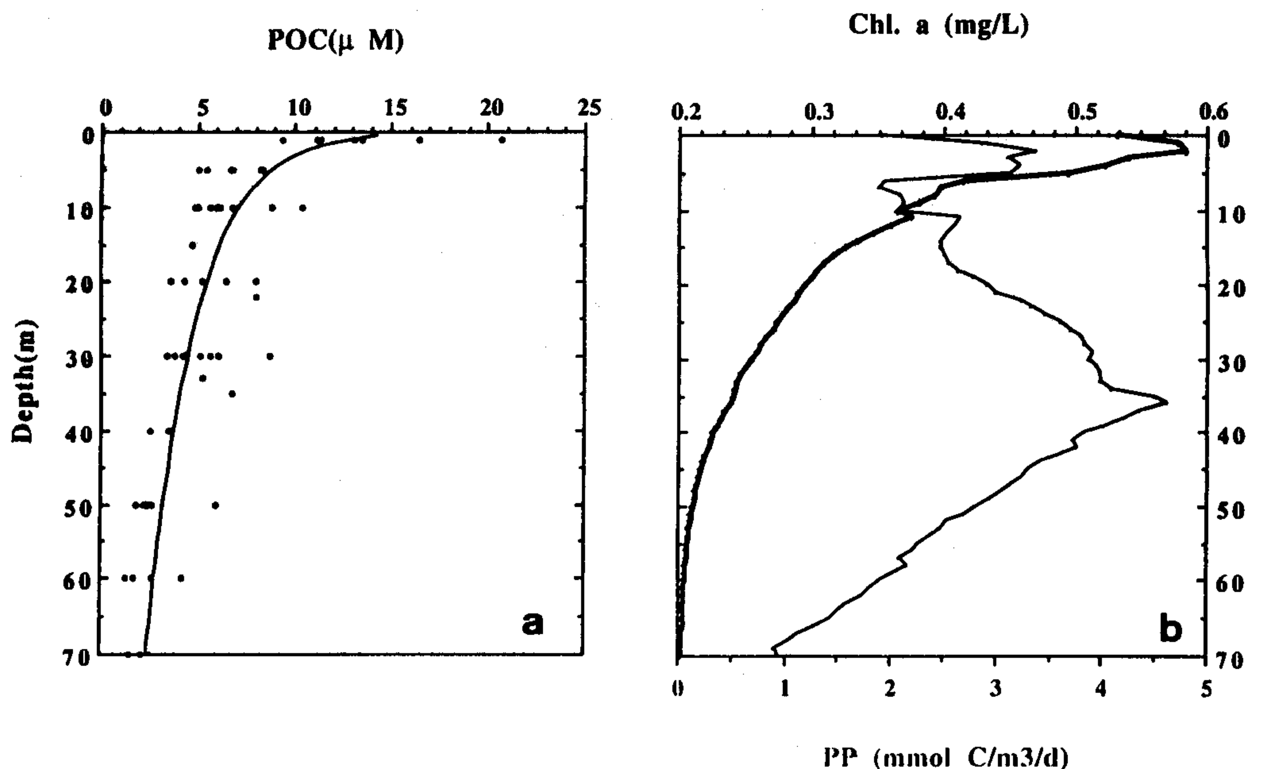
Fig. 10. (a) Left panel: The vertical distribution of POC in the upwelling area during Cruise 352D. (b) Right panel: The mean vertical distribution of chlorophyll a and primary production in the upwelling area during the same cruise.
