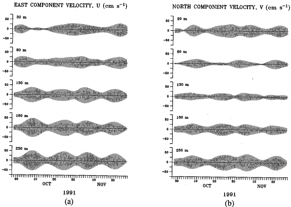
Fig. 3. (a) The band-pass filtered east component velocity ( U ) time series. The uppermost to the bottom panels show the U at 30 m, 80 m, 130 m, 180 m and 230 m, respectively. (b) The band-pass filtered north component velocity ( V ) time series. The uppermost to the bottom panels show the V at 30 m, 80 m, 130 m, 180 m and 230 m, respectively.
