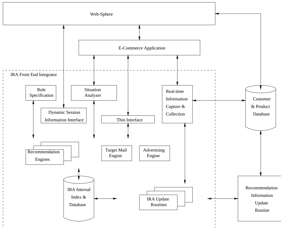
Figure 1: IRA architecture.
