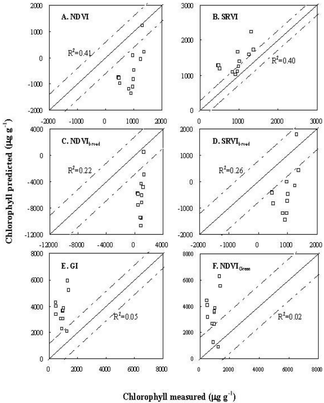
Fig. 5. The results of validation of vegetation indices by independent data sets in which samples containing anthocyanin. R^2 was the determination coefficient between the predicted and the measured Chl contents. The solid line represents the equation \text{Chlorophyll}_{\text{pred}} = \text{Chlorophyll}_{\text{meas}} . The dotted lines represent error of pigment prediction.
