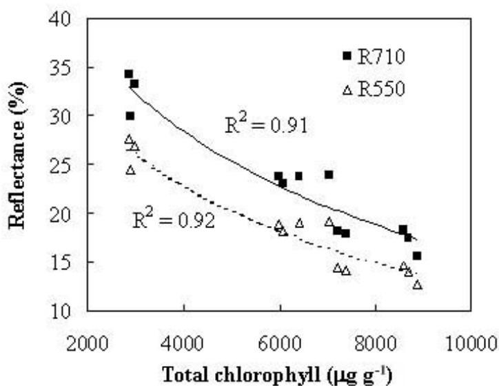
Fig. 3. The reflectance at the wavelengths 710 nm (■) and 550 nm (△) versus total Chl content in sugarcane leaves.
