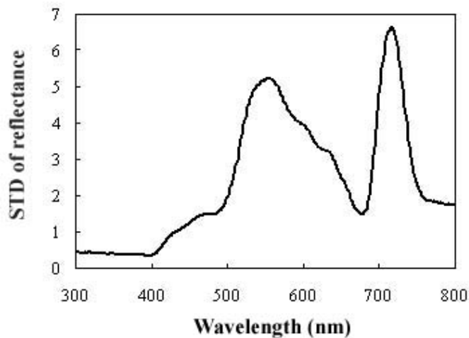
Fig. 2. Standard deviation (STD) of spectral reflectance obtained from sugarcane leaves.
