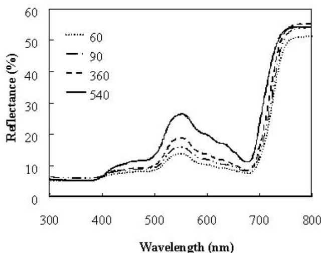
Fig. 1. Reflectance spectra of sugarcane leaves at 60, 90, 360, 540 days after planting.
