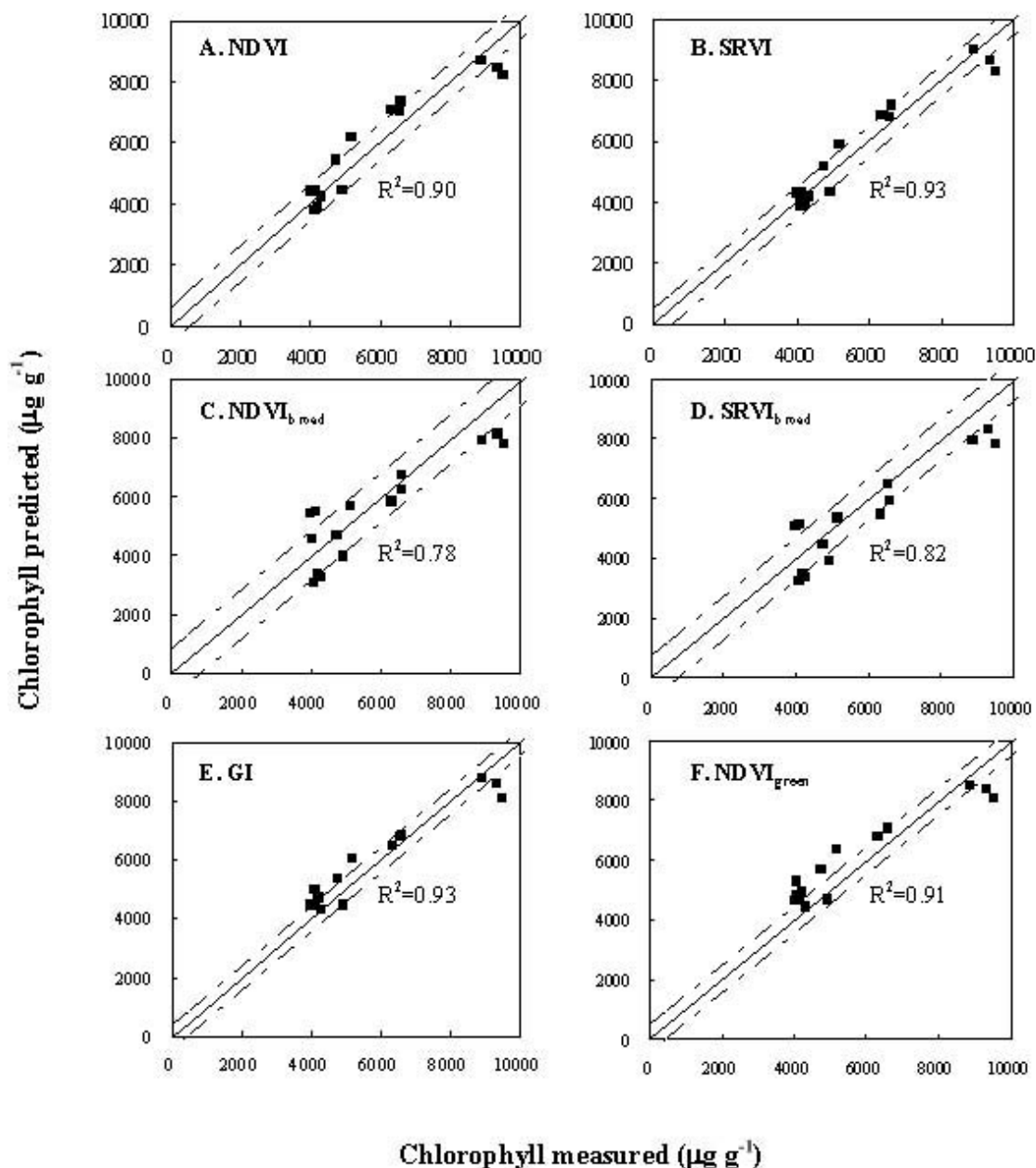
Fig. 4. The results of validation of vegetation indices by independent data sets in which samples containing no anthocyanin. R^2 was the determination coefficient between the predicted and the measured Chl contents. The solid line represents the equation \text{Chlorophyll}_{pred} = \text{Chlorophyll}_{meas} . The dotted lines represent error of Chl prediction.
