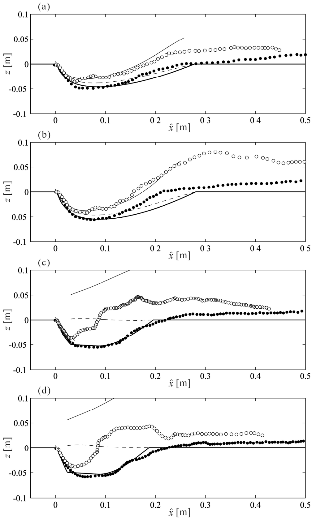
Figure 7. Sample results from our study of moving transverse jets: lines = computational results; dots and circles = laboratory measurements.
