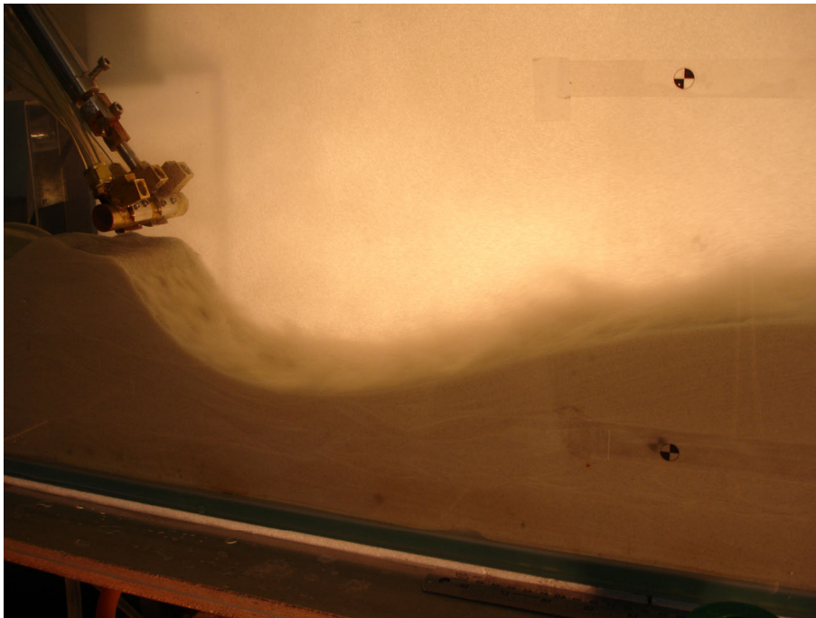
Figure 1. Underwater trench erosion and turbidity current induced by a moving transverse plane jet, in a parallel walled channel, leading to an effectively 2D flow.
