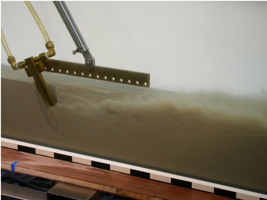
Figure 2. More realistic trenching jets, mounted on an upright sword that moves into the sea bed close to a transparent flume wall, yielding a 3D trench shape and flow pattern.
