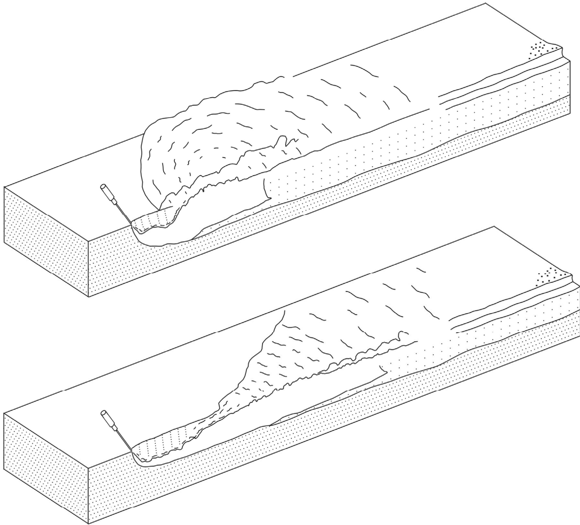
Figure 7. Three-dimensional reconstructions of the patterns of water and sediment motion induced by point jets travelling along erodible sand beds at slow (top) and fast speeds of advance (bottom).
