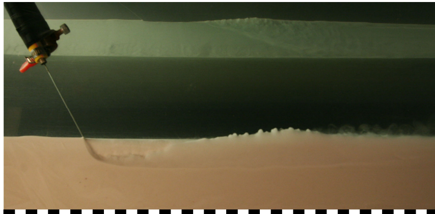
Figure 3. Time-lapse photographs of the flow pattern generated by a rapidly advancing jet ( U = 3.2 cm/s) operating at low power ( Q = 175 ml/min). The mirror shown in Fig. 1d is used to produce the top views observed in the background. The marks on the scale bars are 1 cm long.
