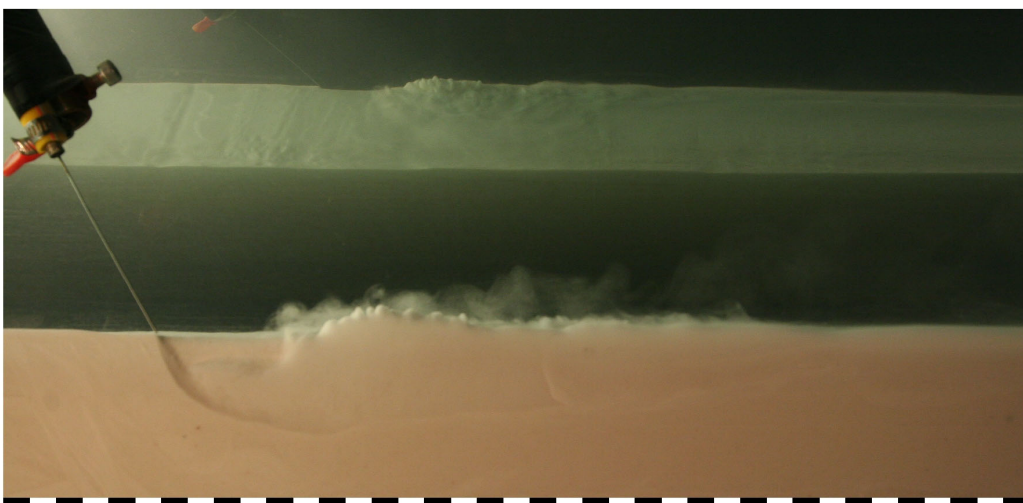
Figure 5. Time lapse images of a small-scale jet trenching flow, seen through the side wall and reflected in an oblique mirror in the background to obtain a top view as well.
