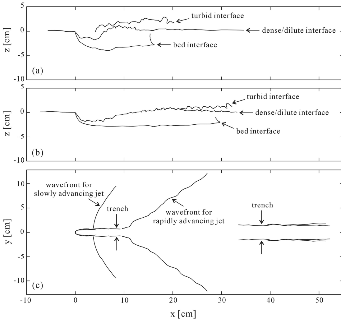
Figure 4. Profiles extracted from side and top views of the jet-induced flows under the lower flowrate Q = 175 ml/min: (a) side view interfaces for a slowly moving jet ( U = 1.9 cm/s); (b) side view interfaces for a jet travelling more rapidly ( U = 3.2 cm/s); (c) top view profiles for both speeds.
