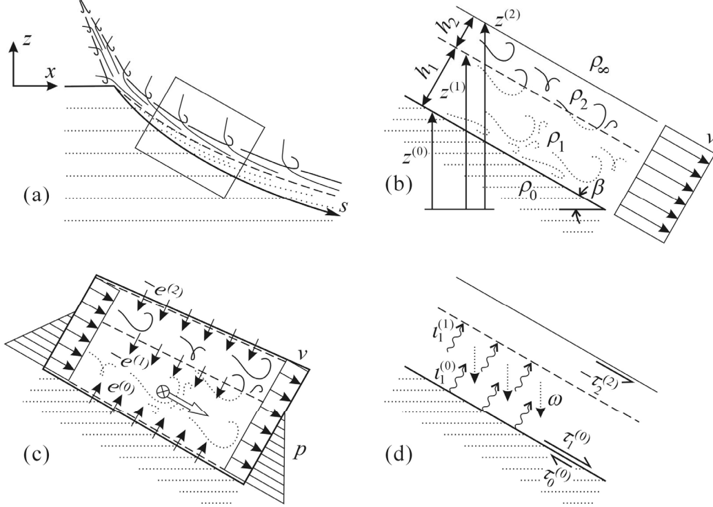
Figure 6. Definition sketch and conceptual view for jet-induced shallow eroding and entraining bed currents.
