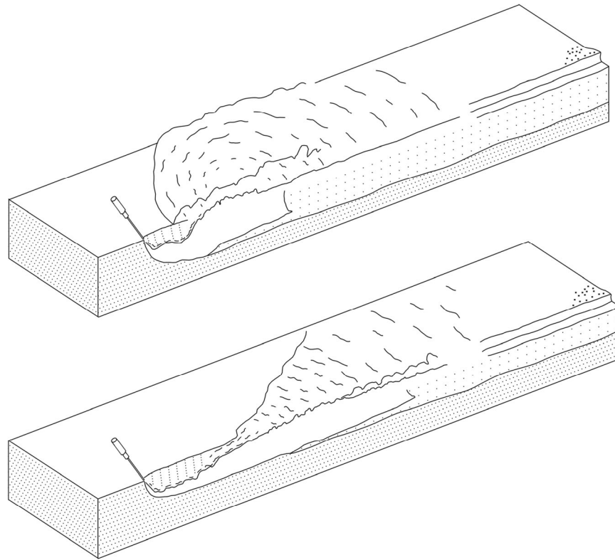
Figure 8. Three-dimensional flow patterns induced along an erodible underwater sand bed by slowly (top) and rapidly moving point jets (bottom).
