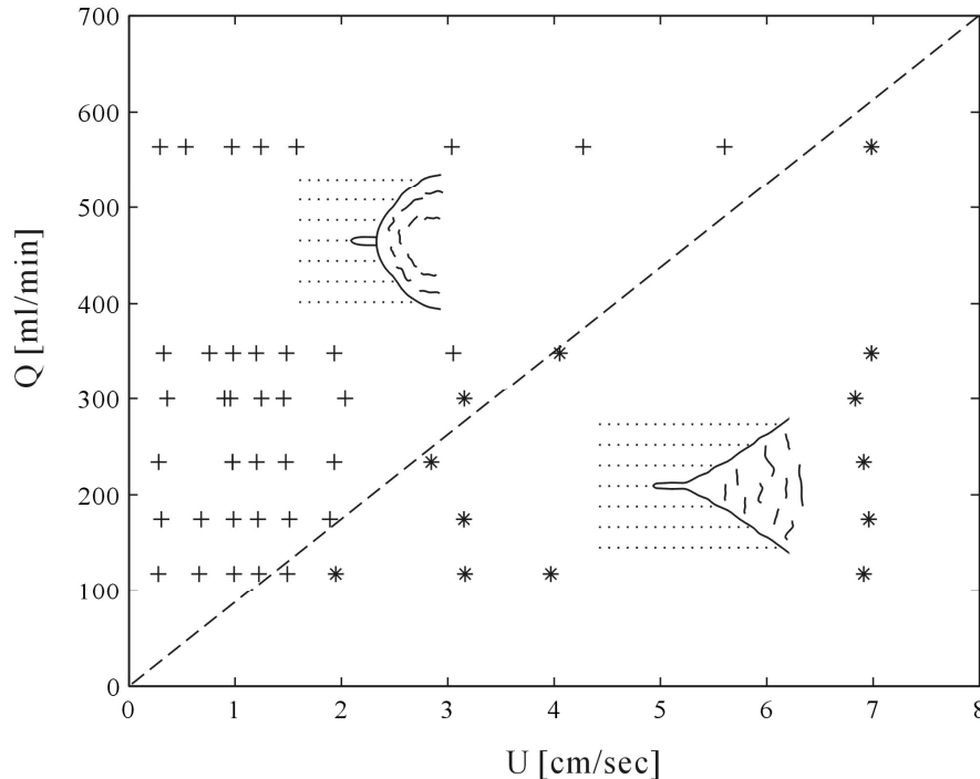
Figure 6. Phase diagram showing experiments in which U-shaped (crosses) and V-shaped overspill patterns (stars) are observed, respectively. The dashed line is a tentative boundary between the regions of occurrence of these two patterns.
