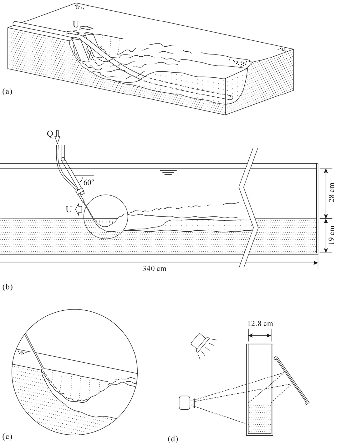
Figure 1. Jet trenching configurations used in the field and in our small-scale laboratory experiments: (a) actual jet trencher vehicles are typically equipped with a pair of jetting swords, placed on both sides of the product (cable or pipeline) to be buried. The pipeline sinks into the seabed thanks to the temporary open trench eroded by the jets, and is then buried by the sediment settling out of the turbid plume further away from the advancing trencher; (b) simplified configuration used for the small-scale experiments, featuring a needle jet moving along the transparent sidewall of the tank to facilitate observation; (c) detail of the needle tip and front region of the jet-incised trench; (d) arrangement of the camera and mirror used to simultaneously acquire side and top views of the jet-induced flow pattern.
