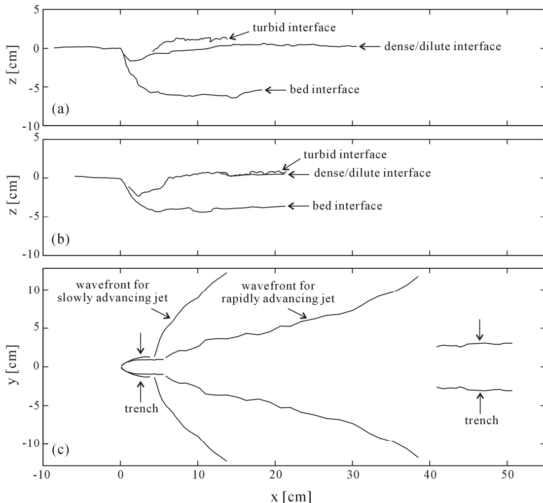
Figure 5. Profiles extracted from side and top views of the jet-induced flows under the higher flowrate Q = 350 ml/min: (a) side view interfaces for a slowly moving jet ( U = 3.1 cm/s); (b) side view interfaces for a jet travelling more rapidly ( U = 7.0 cm/s); (c) top view profiles for both speeds.
