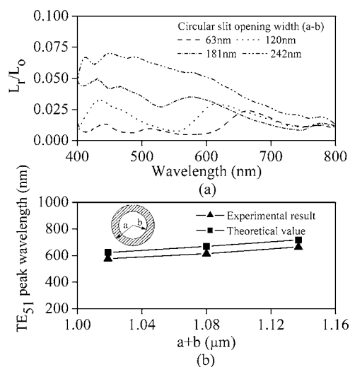
FIG. 1. Optical transmission of a single metallic ring: (a) L_o is the intensity of the halogen lamp light source (outer radius a is fixed at 0.6 \mu\text{m} , and the various line types correspond to the different circular slit opening widths and where Ag film thickness was 235 nm), and (b) comparison of the experimental results with the theoretical values ( TE_{51} ).
