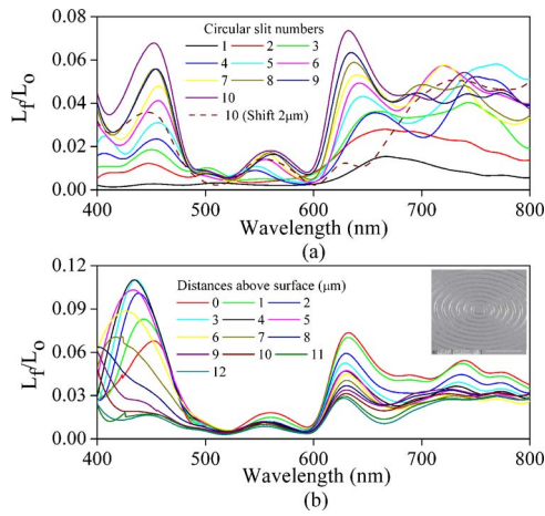
FIG. 2. (Color online) Optical transmission of a circular grating: (a) Ag thickness was 245 nm, with a circular slit width opening of 65 nm at a period of 600 nm and outer radius of first circular slit at 0.6 \mu\text{m} . The various colors represent the various circular slit numbers. The dashed line indicates the transmission spectrum as obtained by shifting the measuring point 2 \mu\text{m} from the center of the grating. (b) The circular grating has ten circular slits (the opening width of the circular slit was 65 nm and Ag film thickness on a glass substrate was 245 nm). The various colors represent the various distances above the metal surface along with the scanning electron microscopy micrograph of the circular grating.
