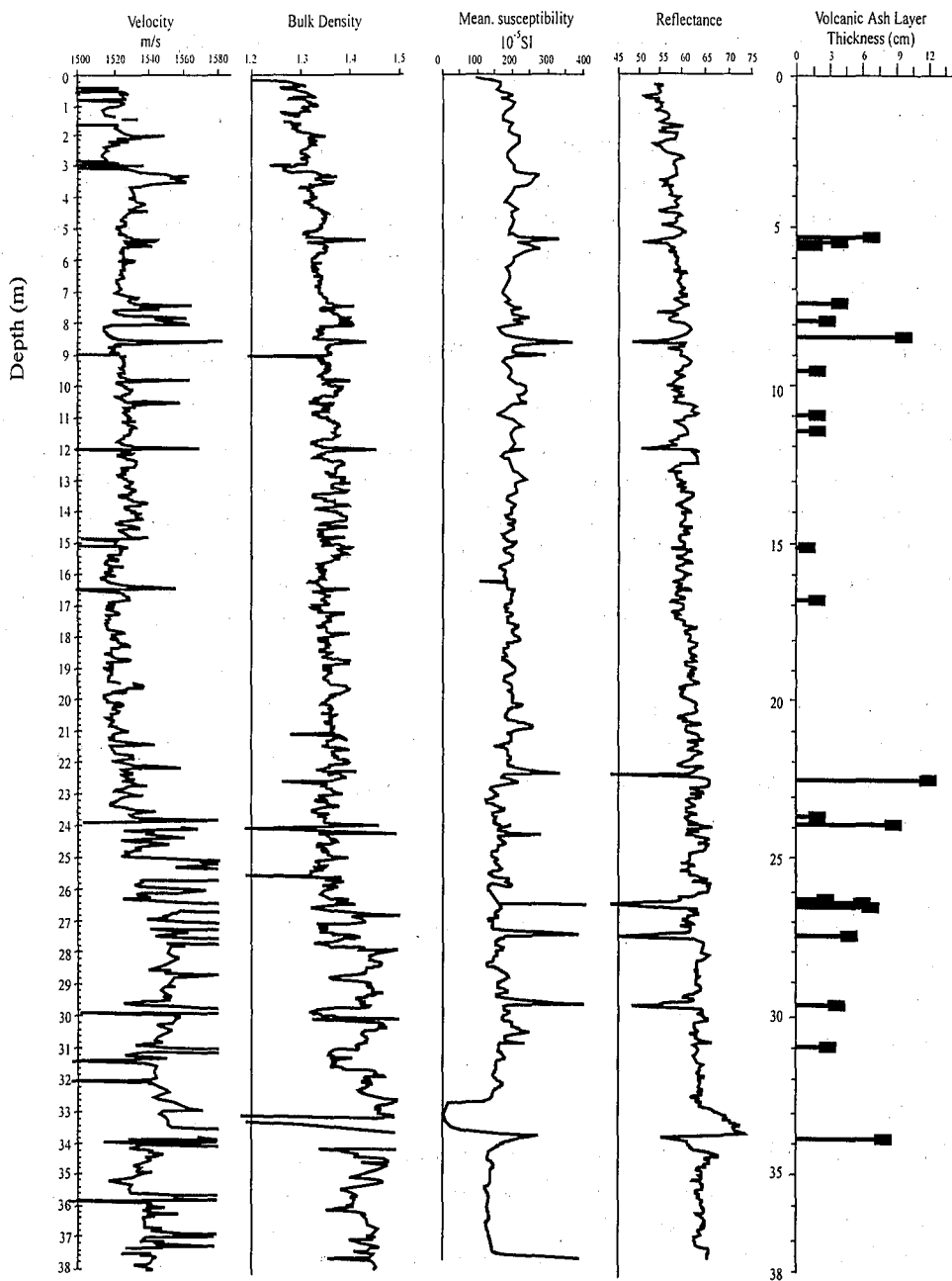
Fig. 3. Time-series of various physical properties including P-wave velocity, bulk density, magnetic susceptibility and reflectance of Core MD 972143. The thickness of volcanic ash layers is also shown in the column on the far right.
