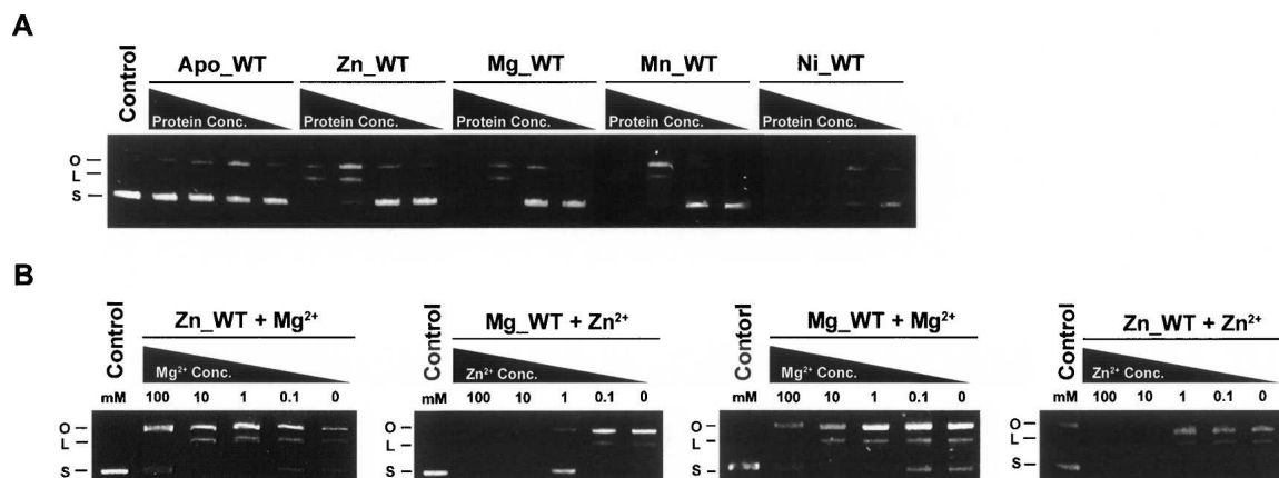
Figure 2. The metal-dependent endonuclease activity of N-Cole7 (the nuclease domain of Cole7). (A) The endonuclease activity of N-Cole7 was analyzed by plasmid digestion assays using pQE-70 as the substrate (see Control lane). Various amounts of apo-N-Cole7 (0.05, 0.27, 1.33, and 6.67 \mu M), did not cleave plasmids (100 ng). However, the endonuclease activity of apo-N-Cole7 was reactivated by the presence of one of the metal ions, Ni 2+ , Mn 2+ , Mg 2+ , and Zn 2+ . Ni-N-Cole7 cleaved plasmids at 0.05 \mu M; Mn- and Mg-N-Cole7 cleaved plasmids at 0.27 \mu M; and Zn-N-Cole7 cleaved plasmids at \sim 1.33 \mu M. (B) Different concentrations of Zn 2+ and Mg 2+ (0, 0.1, 1.0, 10.0, 100.0 mM, as indicated in the figure) were added to Zn-bound and Mg-bound N-Cole7. Both Mg 2+ (0.1 to 10 mM) and Zn 2+ (0.1 to 100 mM) enhanced Cole7 endonuclease activity, but 100 mM of Mg 2+ inhibited enzyme activity. (O) Open, (L) linear, and (S) supercoiled DNA.
