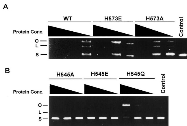
Figure 3. The endonuclease activities of N-ColE7 mutants analyzed by plasmid digestion assays. (A) Various amounts (0.01, 0.05, and 0.27 \mu M) of zinc-bound wild-type and mutated N-ColE7 were incubated with pQE-70 plasmids (100 ng) in 10 mM Tris-HCl (pH 8.0) for 20 min at 37°C. The digested DNA was resolved on 1% agarose gels. The wild-type N-ColE7 started to digest plasmids at 0.01 \mu M. The H573E and H573A N-ColE7 mutants showed reduced endonuclease activities, only starting to cleave DNA at \sim 0.05 \mu M. (B) The H545A and H545E mutants of N-ColE7 had no endonuclease activity when the enzyme concentration was increased from 0.01 to 0.27 \mu M. But H545Q mutant had residual endonuclease activity, cleaving DNA at \sim 0.27 \mu M. (O) Open, (L) linear, and (S) supercoiled DNA.
