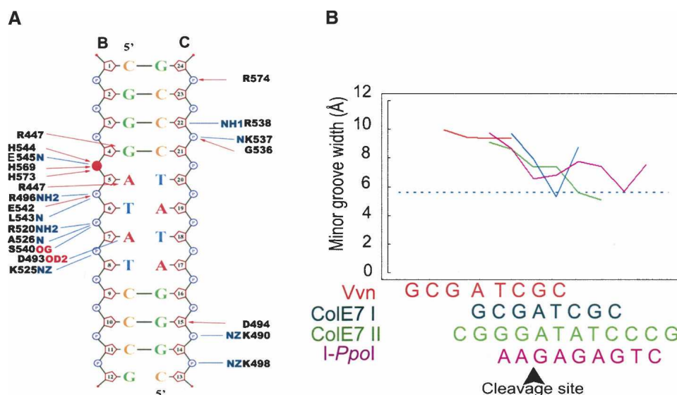
Figure 6. Schematic presentations of the interactions between N-ColE7 and DNA. (A) The solid blue lines indicate hydrogen bonds or salt bridges ( < 3.50 \text{ \AA} ) and the red arrows show van der Waals contacts ( < 3.35 \text{ \AA} ) between N-ColE7 and DNA. Most of the interactions are between proteins side chains and DNA phosphate backbones. (B) DNA groove widths were plotted for each base step in H545E/12-mer DNA complex (this study), N-ColE7/8-mer DNA complex (PDB entry 1PT3), Vvn/DNA (PDB entry 1OUP), and I-PpoI/DNA (PDB entry 1A74). The DNA cleavage sites are aligned and marked by a solid arrow, shown at the bottom of the figure. The minor groove widths are widened to \sim 9 \text{ \AA} at the region bound to \beta\beta\alpha -metal motif in all complexes. DNA is cleaved right at the 3'-side of the widened minor groove.
