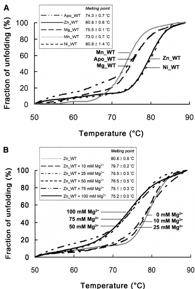
Figure 1. Measurements of the melting points for apo- and metal-bound N-ColE7 by circular dichroism. (A) The melting points of the apo- and each metal-bound N-ColE7 were measured by circular dichroism at a wavelength of 222 nm. The protein concentration used for all measurements was 0.1 mg/mL in 10 mM Tris-HCl (pH 8.0). The melting points were 74.3 \pm 0.7^\circ\text{C} for apo-N-ColE7, 75.5 \pm 0.1^\circ\text{C} for Mg-bound, 73.1 \pm 0.8^\circ\text{C} for Mn-bound, 80.8 \pm 0.8^\circ\text{C} for Zn-bound, and 80.8 \pm 1.4^\circ\text{C} for Ni-bound N-ColE7. (B) The zinc-bound N-ColE7 was mixed with buffers containing 10–100 mM \text{MgCl}_2 . The melting points of N-ColE7 in 10 and 25 mM \text{Mg}^{2+} buffers were \sim 80^\circ\text{C} , close to that of the Zn-bound enzyme, indicating that zinc was still bound in N-ColE7. However, the melting points of N-ColE7 in 50, 75, and 100 mM \text{Mg}^{2+} buffers were shifted to \sim 75^\circ\text{C} , indicating that \text{Zn}^{2+} was not bound to N-ColE7 when \text{Mg}^{2+} concentrations were > 50 mM.
