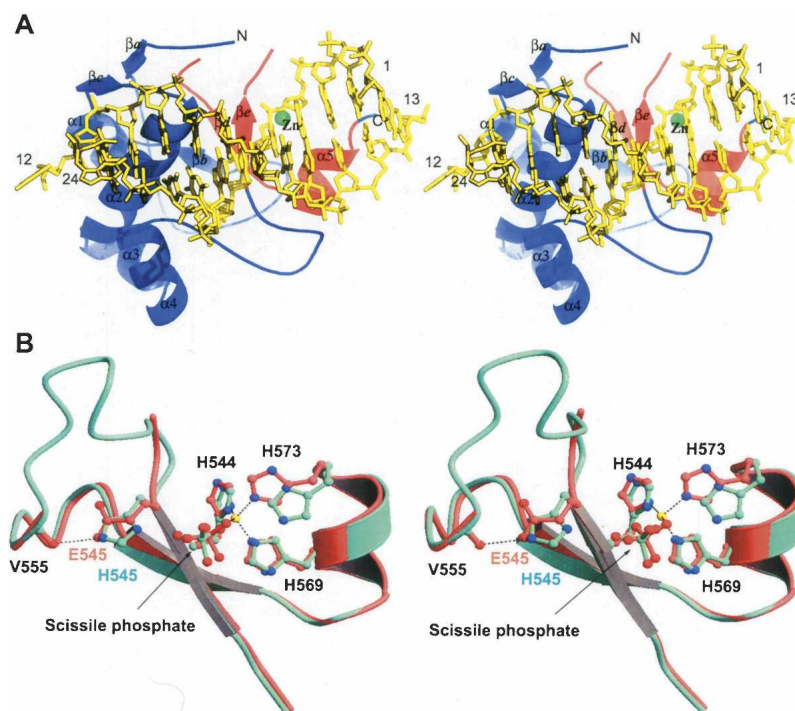
Figure 5. Stereo view of the H545E/DNA/ \text{Zn}^{2+} crystal structure. (A) The H-N-H motif (red) of N-Cole7 (blue and red ribbon) is bound at the minor groove of DNA 12-mer (yellow). DNA is bent \sim 20^\circ (calculated by Curve [Lavery and Sklenar 1988]) away from N-Cole7. The zinc ion (displayed as a green ball) is located closely to one of the phosphates in the DNA backbone. (B) The zinc-bound active site in the N-Cole7/12-mer DNA complex (red) was superimposed with the metal-free active site (green) in the N-Cole7/8-mer DNA complex (PDB entry 1PT3). The two structures fitted well with an average RMS difference of 0.34 Å for 18 \text{C}_\alpha atoms located in \beta -strand or \alpha -helix regions used for superimposition. In the zinc-bound active site, the zinc ion is coordinated to the side chains of H544, H569, and H573 and the scissile phosphate in a tetrahedral geometry. In the zinc-free active site, only H573 shifted away slightly. The loop between residues 548 to 554 was disordered and not modeled in the H545E/DNA/Zn complex.
