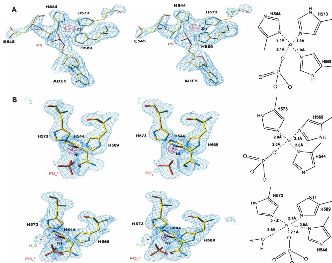
Figure 4. The omit electron density maps of Zn-bound and Ni-bound endonuclease active sites in H545E/DNA/ \text{Zn}^{2+} and N-ColE7/Im7/ \text{Ni}^{2+} complexes, respectively. (A) Stereo view of the omit difference maps ( F_o - F_c ) contoured at 2.5 \sigma (blue) and 12.0 \sigma (red) shows that the DNA scissile phosphate (P5) is bound directly to the zinc ion. The tetrahedral geometry and bond distances around the Zn atom are schematically shown in the right panel. (B) Stereo views of the omit difference maps contoured at 2.5 \sigma (blue) and 18.0 \sigma (red) around the Ni-binding site in the two noncrystallographic-symmetry related molecules in N-ColE7/Im7/ \text{Ni}^{2+} complex structure. In molecule A, \text{Ni}^{2+} is bound to three histidines and a phosphate in a tetrahedral geometry. In molecule B, \text{Ni}^{2+} is bound to three histidines, a phosphate, and a water molecule in a distorted trigonal bi-pyramidal geometry.
