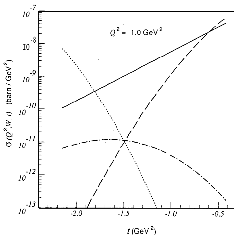
FIG. 5. The t -dependence of the virtual photoproduction cross section \sigma(Q^2, W, t) with W=2.1 GeV and Q^2 = 1.0 GeV 2 in RHOM. Notation is the same as in Fig. 4.
