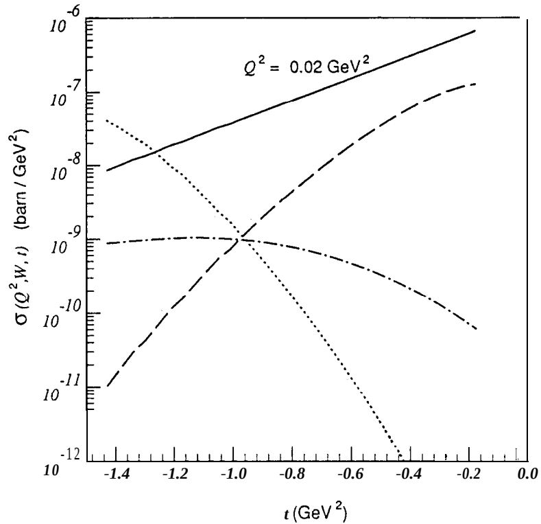
FIG. 4. The t -dependence of the virtual photoproduction cross section \sigma(Q^2, W, t) with W=2.1 GeV and Q^2 = 0.02 GeV 2 in RHOM. The curves are as follows. The diffractive cross section – solid line; s\bar{s} knockout – dashed line; uud knockout – dotted line; interference term – dash-dotted line.
