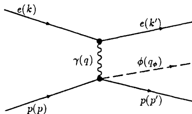
FIG. 1. Feynman diagram for the one-photon exchange electroproduction of \phi meson from the proton.
