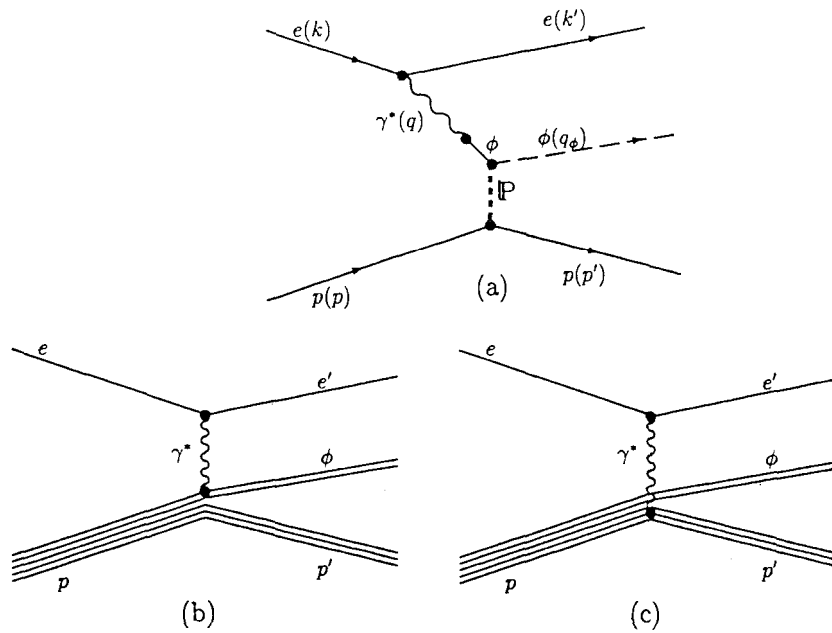
FIG. 2. (a) Diffractive \phi -meson production within vector meson dominance model by means of the Pomeron exchange; (b) s\bar{s} -knockout contribution to the electroproduction of \phi meson; (c) uud -knockout contribution.
