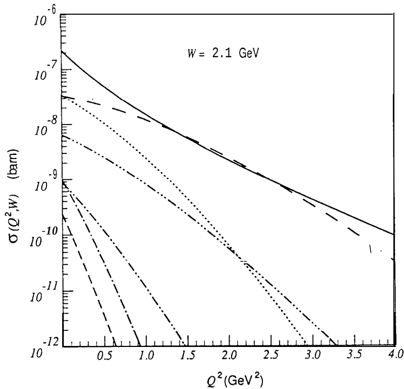
FIG. 3. The Q^2 -dependence of the virtual photoproduction cross section, \sigma(Q^2, W) with W=2.1 GeV in RHOM and in NRQM. The curves are as follows. The diffractive cross section – solid line; RHOM: s\bar{s} knockout cross section – long dashed line, u\bar{u} knockout – dash-dotted-dotted line, interference term – dash-dotted line; NRQM: s\bar{s} knockout cross section – dotted line, u\bar{u} knockout – dashed line, interference term – dash-dotted line.
