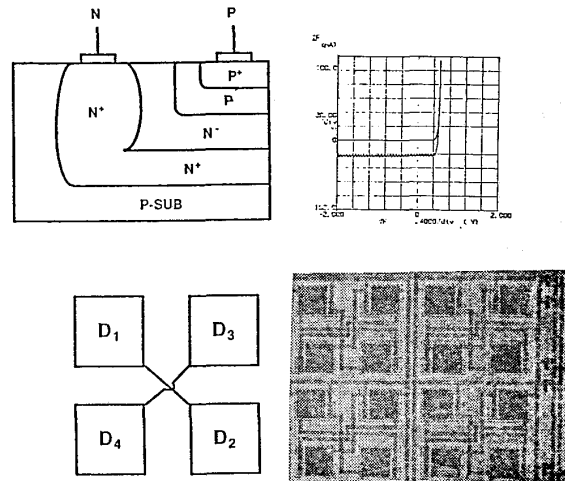
Fig. 1. (a) The photodiode structure. (b) IV characteristics of the photodiode. (c) Low cross-coupled pairs of back-to-back-connected photodiodes in each pixel area.
