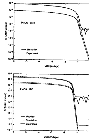
Fig. 3. IV characteristics of the NMOS and PMOS devices at 298K and 77K.
