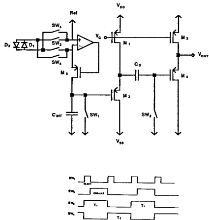
Fig. 2. The readout circuit.
