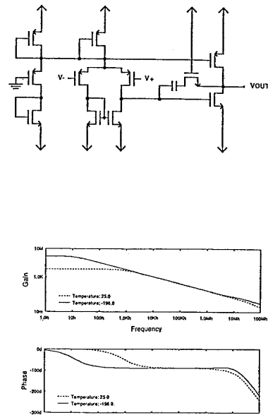
Fig. 4. The CMOS op amp operating at 77K.
