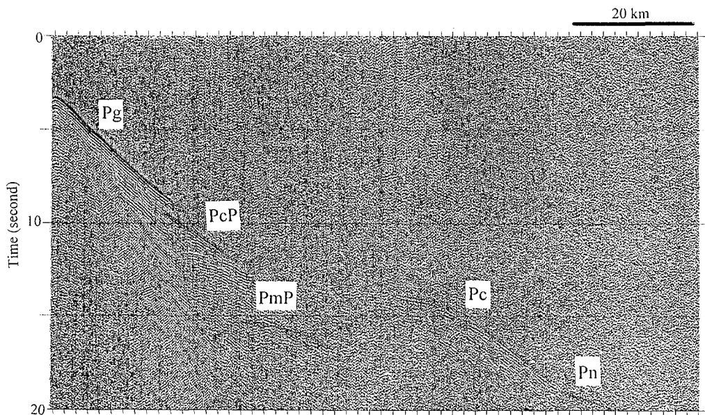
Fig. 5. Receiver gathering at station 28 in middle of the south-link highway by Reftek recorder. In profile, R/V Maurice Ewing was firing shots from Pacific and cruising westward to Taiwan. Total recording time for each trace was 20 seconds with 10 ms sampling interval. Trace spacing is about 50 m. In this figure, clear events of Pg, PcP, PmP, Pc, and Pn may be seen.
