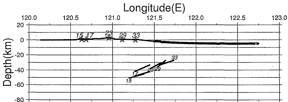
Fig. 7. Final interpreted image of deep crustal structure along southern cross-island highway profile. Image was interpreted using stacked data from stations 15, 17, 23, 29, and 33.
