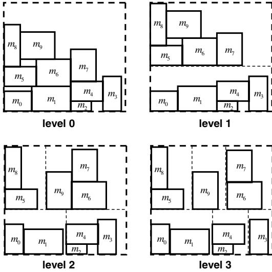
Fig. 7. Illustration of the interactive global optimization and partitioning steps ( q = 2 ).
