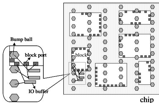
Fig. 1. Example layout of the flip chip.
