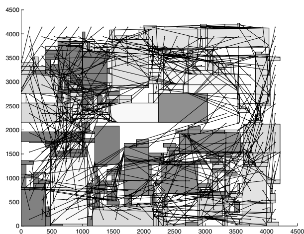
Fig. 13. The floorplanning result of fc3.
