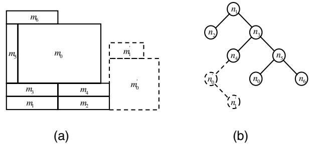
Fig. 9. The blocks of solid lines belong to a clustered block m_i , and the blocks of dotted lines belong to another clustered block m_l . m_l is the left child of m_i . (a) m_i and m_l after declustering. (b) The corresponding tree topology after declustering. (Here, m_4 is the tail block on the last contour.)
