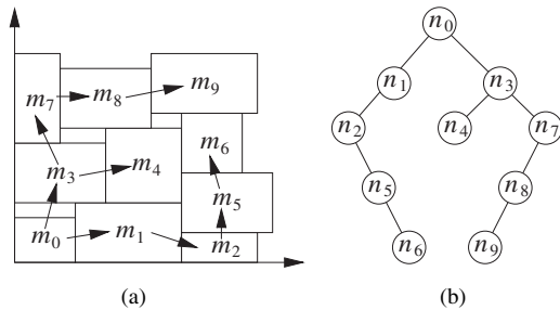
Fig. 4. (a) An admissible placement. (b) The corresponding B*-tree.
