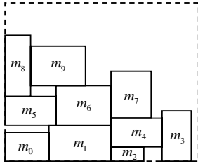
Fig. 3. The B*-tree based floorplanner always packs blocks to the left and to the bottom.
