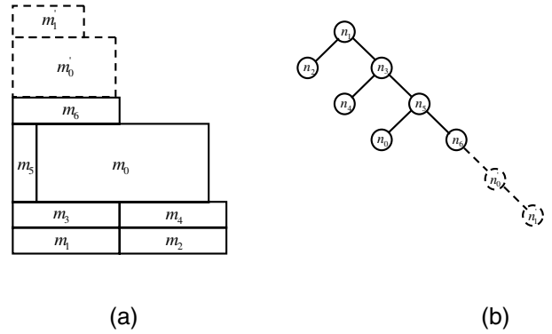
Fig. 10. The blocks of dotted lines belong to the clustered block m_r . m_r is the right child of m_i . (a) m_i and m_r after declustering. (b) The corresponding tree topology after declustering.
