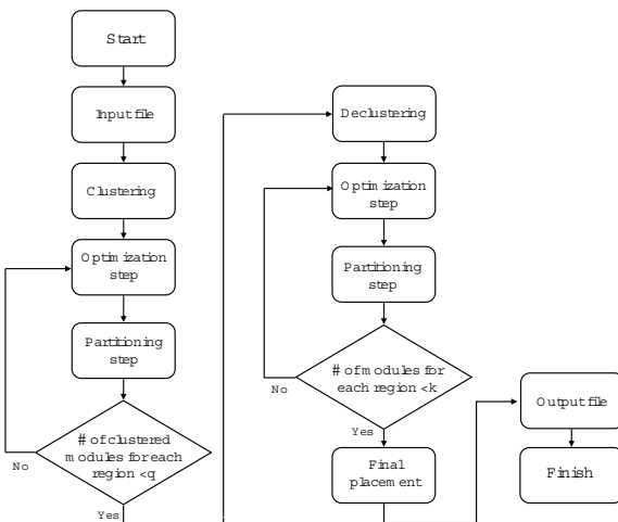
Fig. 12. The flow chart of our floorplanning method.
