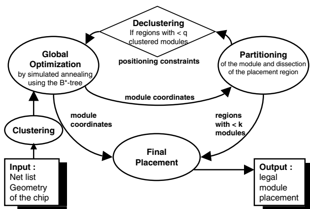
Fig. 5. Our algorithm.
