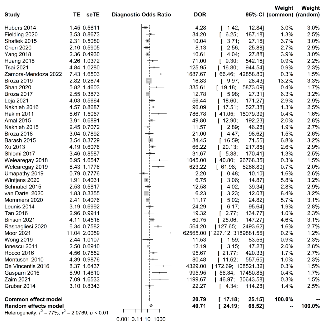
Figure 3. Forest plot and pooled diagnostic odds ratio analysis. Vertical dashed lines indicate 95% CI for the pooled effect. The size of the data markers reflects the weight. Error bars indicate 95% CI.
