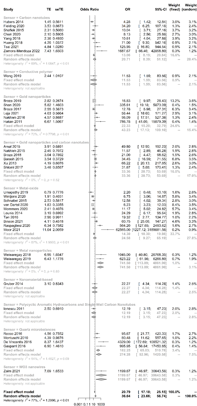
Figure 6. Subgroup analysis for pooled diagnostic odds ratio based on the type of sensor. The type of sensor is based on the classification provided in the literature.
