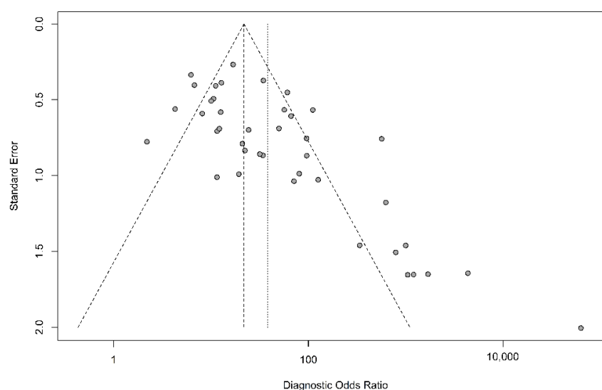
Figure 4. Funnel plot of the diagnostic odds ratio. A skewed asymmetrical funnel plot shows that there is publication bias. In the right lower corner, the small sample size studies (therefore large standard error) are more prone to publication bias than large studies.
