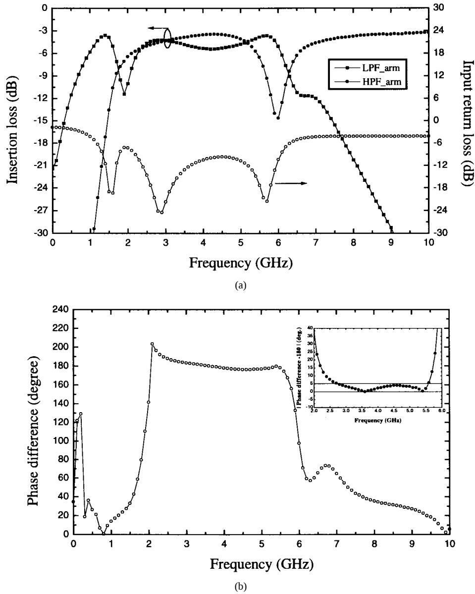
Fig. 2. The measurements of compensated high/low-pass balun: (a) amplitude balances and (b) phase balances.
