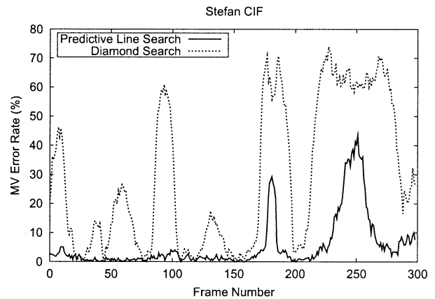
Fig. 8. Motion-vector error rate comparison between the PLS and the DS algorithms. The input sequence is the Stefan sequence in CIF format.
