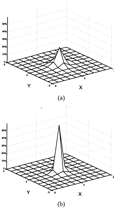
Fig. 2. Motion-vector distribution for the Foreman sequence. (a) Distribution of the motion vector. (b) Distribution of the motion-vector residue after prediction.
