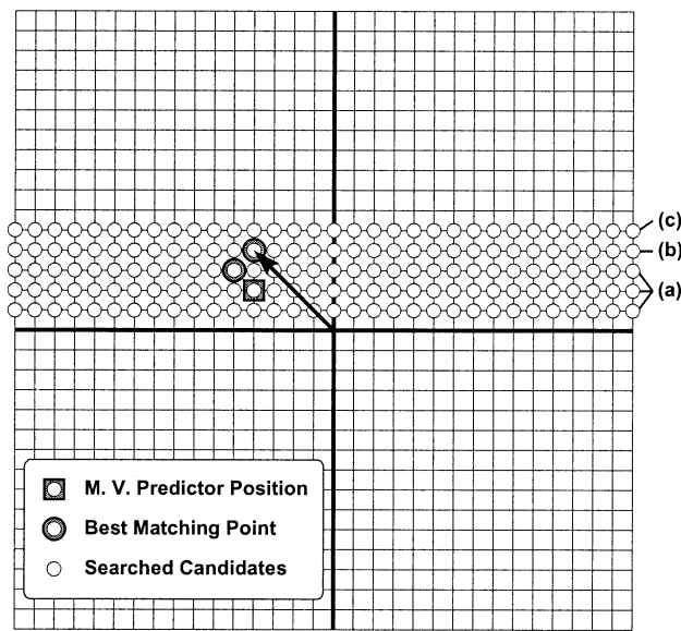
Fig. 4. PLS procedure. The search range is (-16, 15) , the motion-vector predictor is (-4, -2) , and the best-matching point is (-4, -4) in this example.
