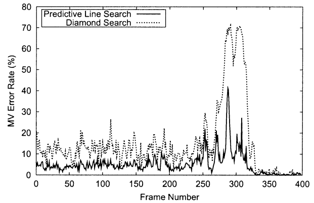
Fig. 7. Motion-vector error rate comparison between the PLS and the DS algorithms. The input sequence is the Foreman sequence in CIF format.
