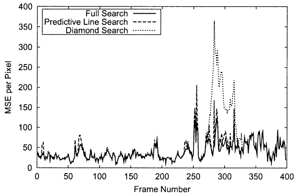
Fig. 5. MSE comparison between the PLS, the DS, and the FS algorithms. The input sequence is the Foreman sequence in CIF format
