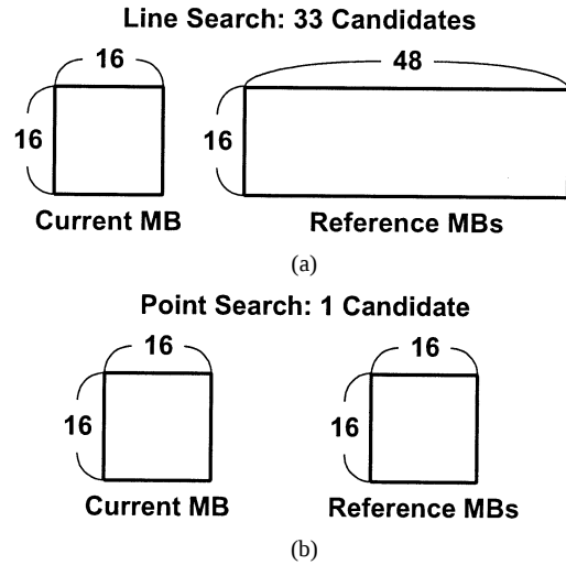
Fig. 3. Memory access comparison: (a) one-line search for PLS versus (b) one-point search for DS.
