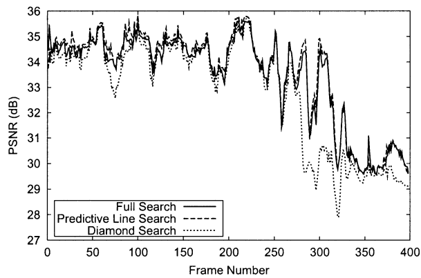
Fig. 9. PSNR comparison for the MPEG-4 encoder using three different motion-estimation algorithms: the FS, the PLS, and the DS algorithms. The input sequence is the Foreman sequence in CIF format and the target bit rate is 384 Kbits/s.
