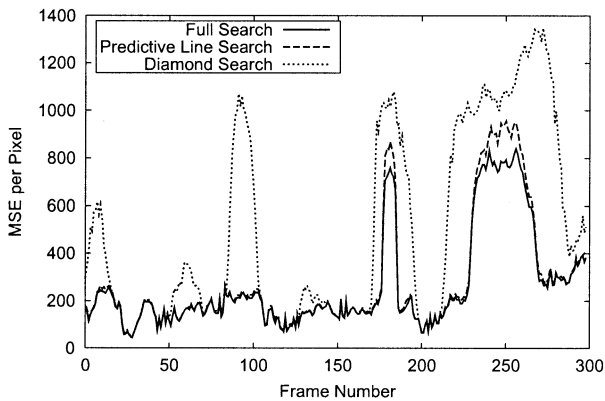
Fig. 6. MSE comparison between the PLS, the DS, and the FS algorithms. The input sequence is the Stefan sequence in CIF format.
