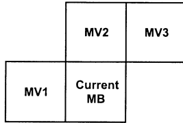
Fig. 1. Motion-vector prediction: the predictor for the current macroblock is the medium of MV1, MV2, and MV3.
