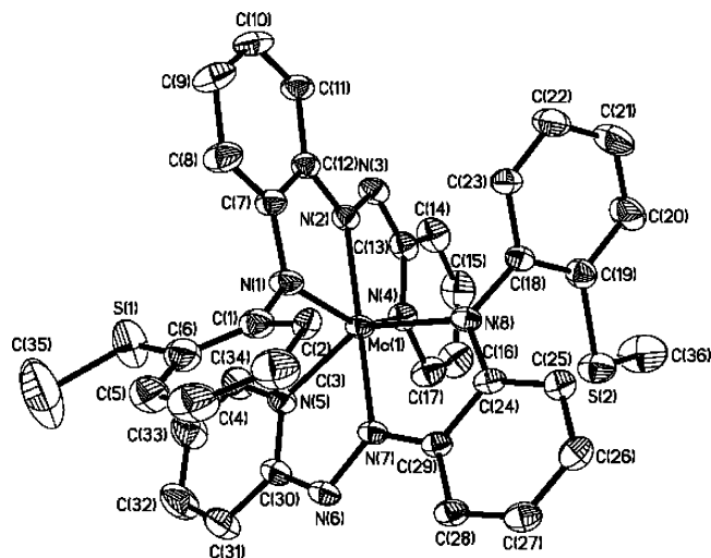
Figure 2. Molecular structure and atom numbering scheme for Mo[L e ] 2 .
