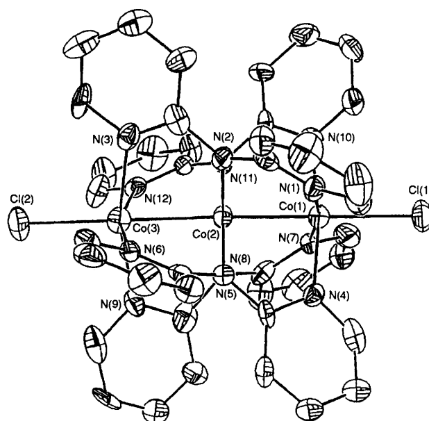
Fig. 1 ORTEP view of the Co 3 (dpa) 4 Cl 2 (along the Cl–Co–Co–Co–Cl axis) Pertinent bond lengths (Å) and angles (°): Co(1)–Cl(1), 2.432(4); Co(1)–N, 1.944(9)–1.983(9), av. 1.964; Co(2)–Co(3), 2.472(3); Co(2)–N, 1.893(9)–1.913(9), av. 1.900; Co(3)–Cl(2) 2.361(4); Co(3)–N, 2.108(9)–2.145(9), av. 2.121. N(1)–Co(1)–Co(2)–N(2), 26.1; N(4)–Co(1)–Co(2)–N(5), 25.1; N(7)–Co(1)–Co(2)–N(8), 26.8; N(10)–Co(1)–Co(2)–N(11), 26.7; N(2)–Co(2)–Co(3)–N(3), 20.3; N(5)–Co(2)–Co(3)–N(6), 24.3; N(8)–Co(2)–Co(3)–N(9), 24.1; N(11)–Co(2)–Co(3)–N(12), 21.2.
