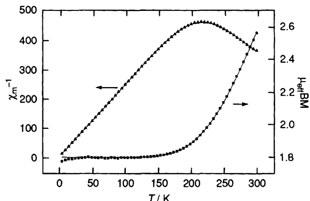
Fig. 2 Magnetic data for Co 3 (dpa) 4 Cl 2 powder sample at 1 T: observed values of χ m −1 (▲) and μ eff (■); Curves are calculated based on the equation μ eff 2 = [150γx C μ E 2 + 25{γx(5 − γ) 2 − 20(2 − γ) 2 } exp{ − (E/ζ + 5γ/6)x} + 2{5γx(11 + 2γ) 2 + 88(2 − γ) 2 } exp{ − (E/ζ + γ/3)x} + 9{35γx(3 + γ) 2 + 36(2 − γ) 2 } exp{ − (E/ζ − γ/2)x}] × (72γx[2C + exp{ − (E/ζ + 5γ/6)x} + 2exp{ − (E/ζ + γ/3)x} + 3 exp{ − (E/ζ − γ/2)x}]) −1 where μ E = 1.757 BM, γ = −1.5, ζ = 540 cm −1 , x = ζ/kT, E = 1638 cm −1 , C = 0.0405.
