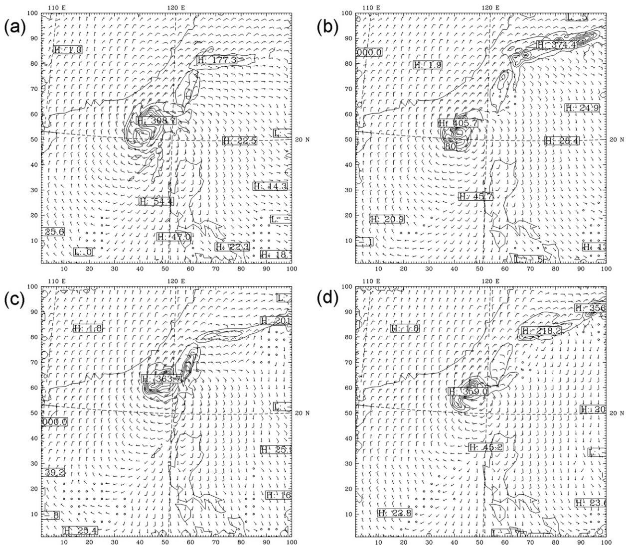
FIG. 9. Simulated 1000-hPa wind field (one full wind barb = 10 \text{ m s}^{-1} ) and 12-h accumulated rainfall (contour interval of 50 mm) in experiment (a) E20_KF and (b) E20_small valid at 1200 UTC 25 Oct 1998. (c),(d) As in (a),(b) but valid at 0000 UTC 26 Oct 1998.
