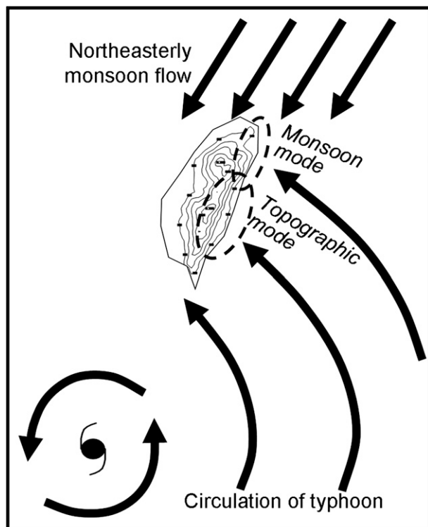
FIG. 13. Schematic diagram of the rainfall mechanisms associated with the monsoon mode and the topographic mode, as a response to the interaction among the typhoon circulation, northeasterly monsoon flow, and terrain of Taiwan (contour interval of 500 m).
