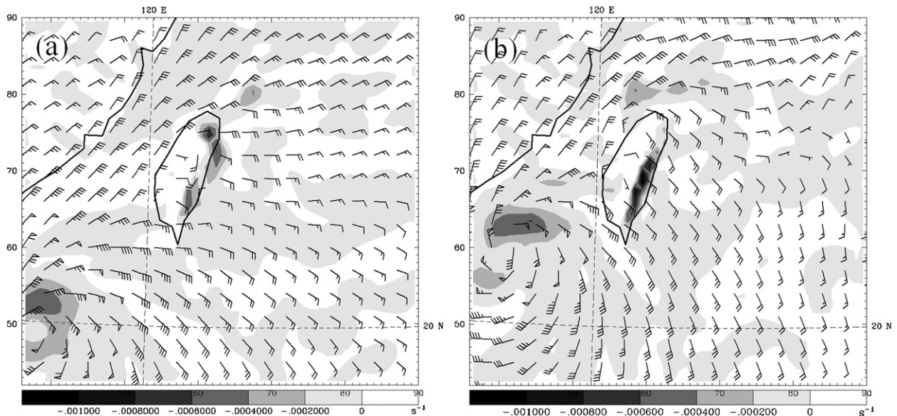
FIG. 4. Simulated 1000-hPa wind field (one full wind barb = 5 \text{ m s}^{-1} ) and divergence (shaded, contour interval is 2 \times 10^{-4} \text{ s}^{-1} ) in experiment E20_KF at (a) 0000 UTC 25 and (b) 0000 UTC 26 Oct 1998.
