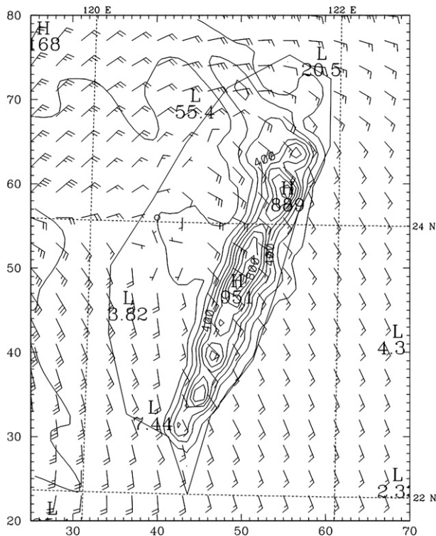
FIG. 5. As in Figs. 3b, but for experiment E6.67_KF and with contour interval of 100 mm.
