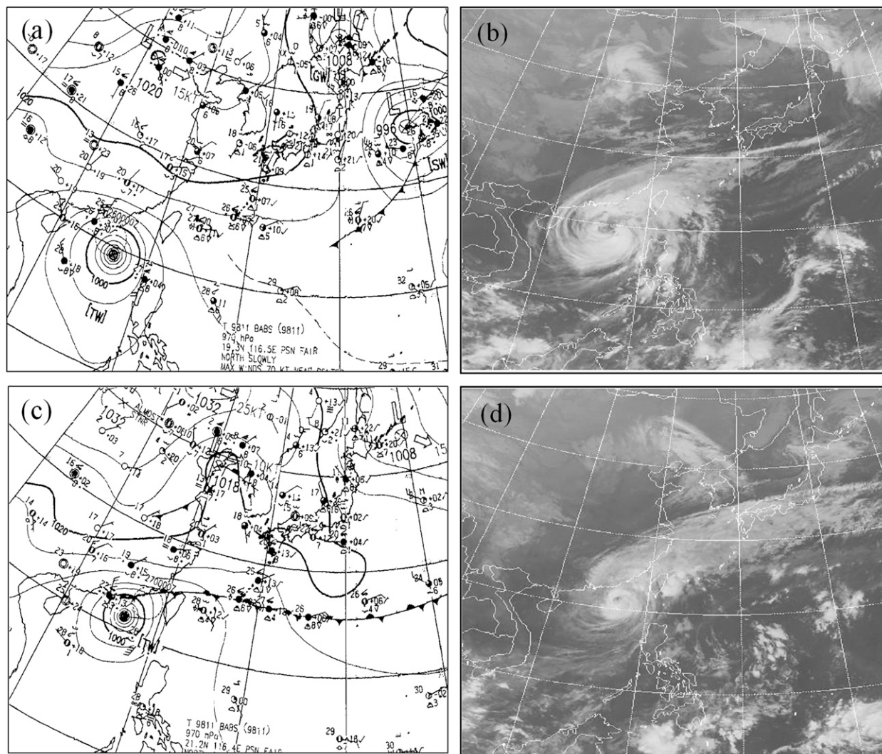
FIG. 1. (a) Surface weather map [Japan Meteorological Agency (JMA)] and (b) geostationary meteorological satellite (GMS-5) infrared satellite imagery at 0000 UTC 25 Oct 1998. (c), (d) As in (a) and (b) but at 0000 UTC 26 Oct 1998.
