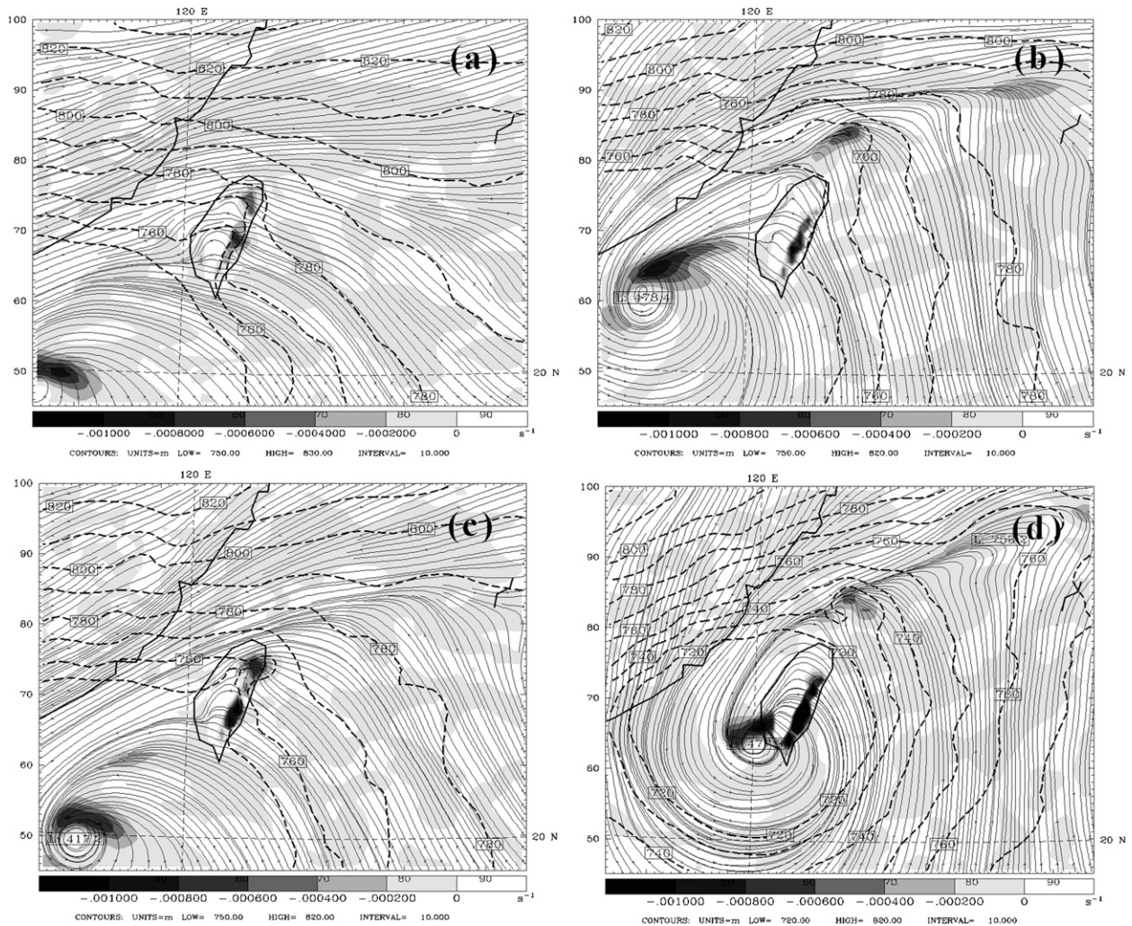
FIG. 12. Simulated 925-hPa streamline, geopotential height (dashed line, m) and divergence (shaded, contour interval is 2 \times 10^{-4} \text{ s}^{-1} ) in experiment E20_M1 at (a) 1800 UTC 24 and (b) 0000 UTC 26 Oct. (c),(d) As in (a),(b) but for experiment E20_M2.
