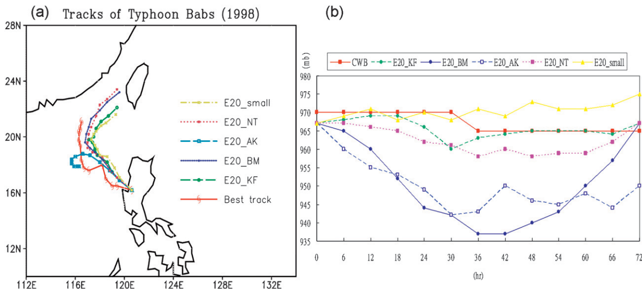
FIG. 2. (a) CWB best track and simulated tracks with six-hourly positions and (b) simulated minimum sea level pressure (hPa) of Typhoon Babs from 0000 UTC 23 to 0000 UTC 26 Oct 1998 for five of the experiments in this study.
