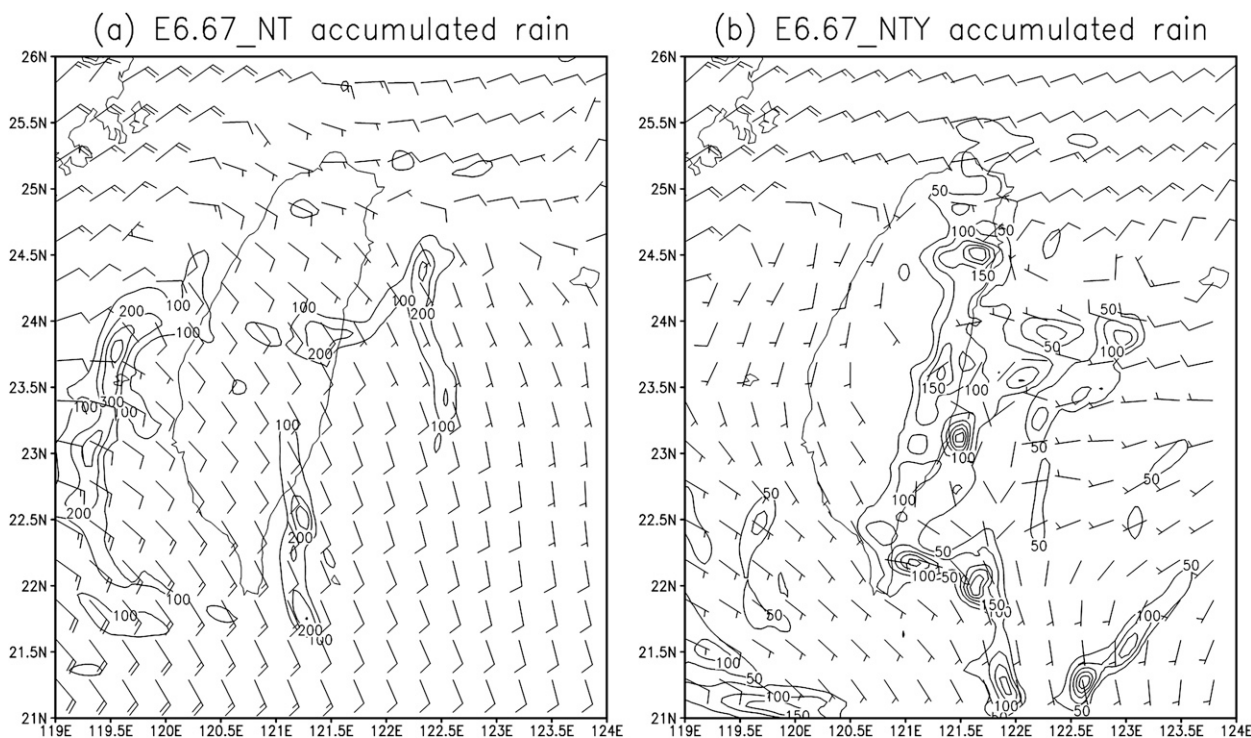
FIG. A1. As in Fig. 3b, but for the (a) no-terrain (NT) and (b) no-typhoon (NTY) simulations with 6.67-km resolution.
