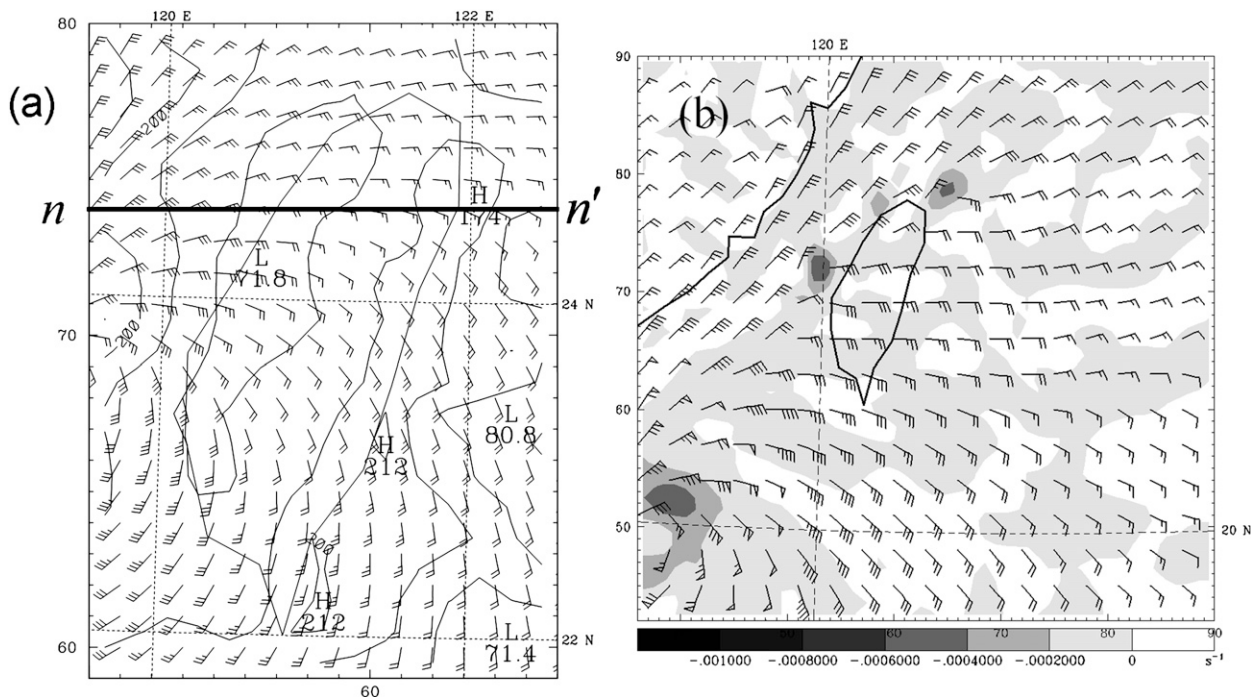
FIG. 6. (a) As in Figs. 3b, and (b) as in Fig. 4a but for experiment E20_NT.
