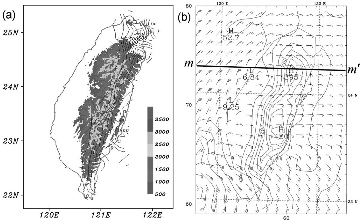
FIG. 3. (a) Observed and (b) simulated accumulated rainfall (contour interval of 50 mm) in experiment E20_KF from 0000 UTC 23 to 0000 UTC 26 Oct 1998. Also shown in (b) is 900-hPa simulated wind field at 0000 UTC 26 Oct (one full wind barb = 10 m s -1 ).
