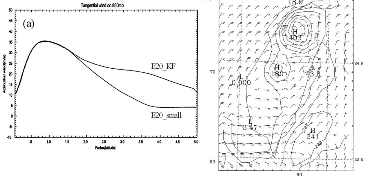
FIG. 8. (a) Azimuthally average tangential wind profiles ( \text{m s}^{-1} ) from center of bogus vortex in experiments E20_KF and E20_small, and (b) as in Figs. 3b, but for experiment E20_small.
