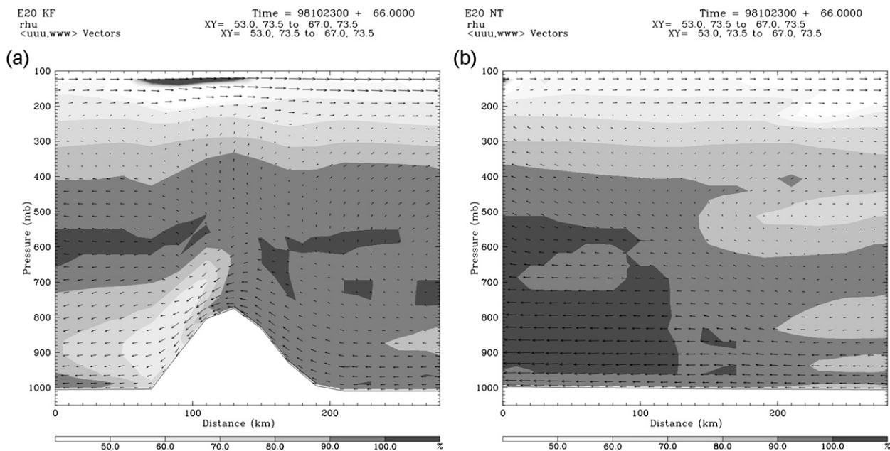
FIG. 7. East-west-oriented cross section of relative humidity (%), and zonal and vertical wind (vector) for experiment (a) E20_KF along line mm' in Fig. 3b and (b) E20_NT along line nn' in Fig. 7a at 1800 UTC 25 Oct 1998.
