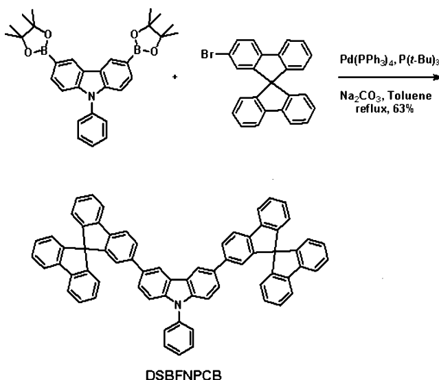
Scheme 1 Synthesis of DSBFNPCB
