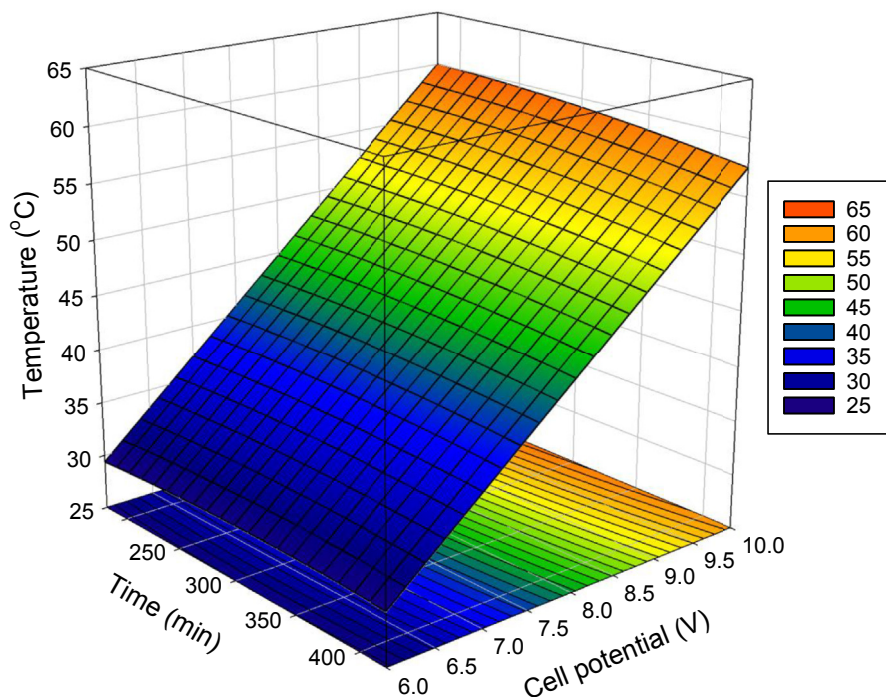
Figure 2 – Response surface and contour plots of electrolyte temperature with respect to electrolysis time and electric potential in electrolysis of deep ocean water.
