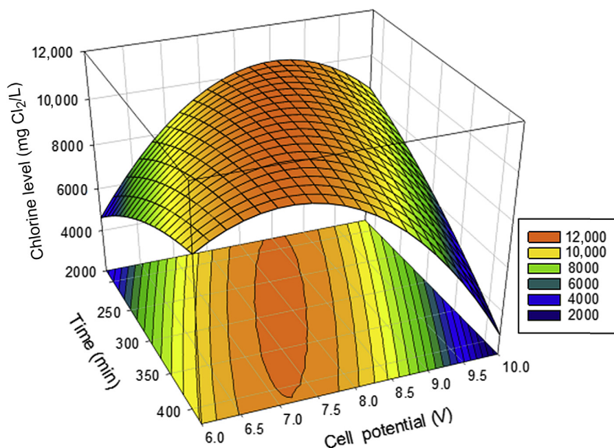
Figure 3 – Response surface and contour plots of chlorine concentration with respect to electrolysis time and electric potential in electrolysis of deep ocean water.
