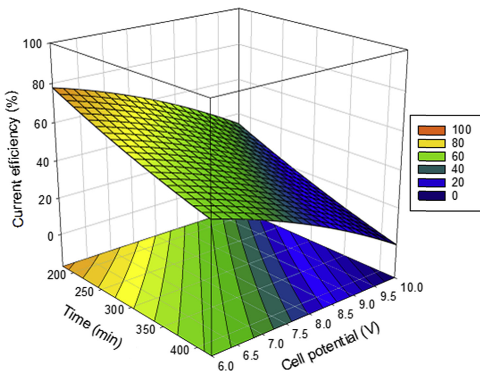
Figure 5 – Response surface and contour plots of current efficiency with respect to electrolysis time and electric potential in electrolysis of deep ocean water.
