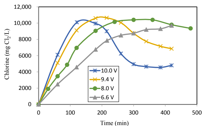
Figure 4 – Chlorine concentration of deep ocean water in electrolysis at different electric potential.
