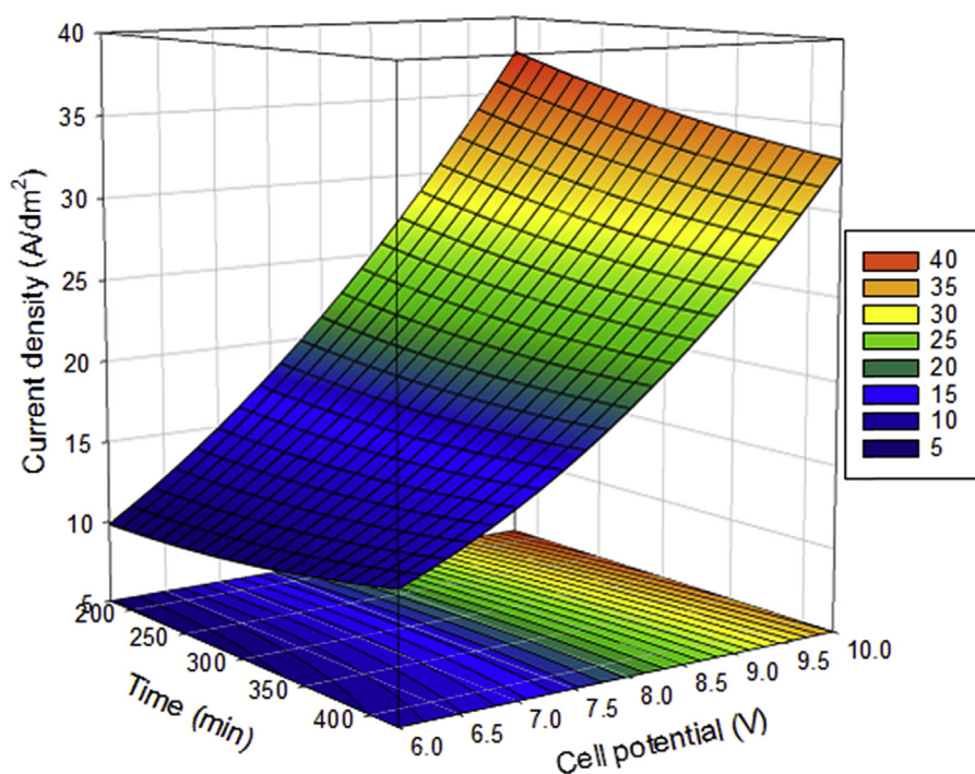
Figure 1 – Response surface and contour plots of current density with respect to electrolysis time and electric potential in electrolysis of deep ocean water.
