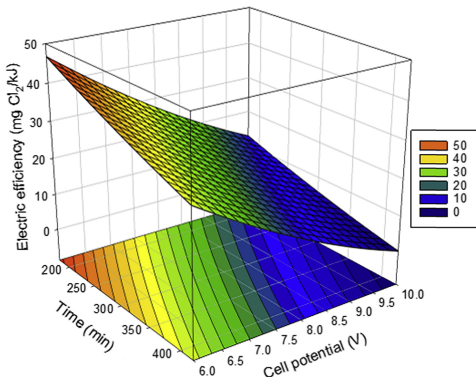
Figure 6 – Response surface and contour plots of electric efficiency with respect to electrolysis time and electric potential in electrolysis of deep ocean water.
