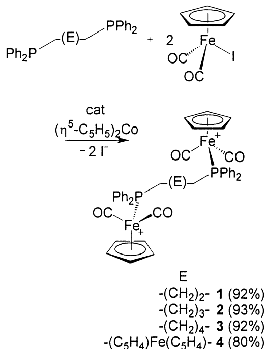
Fig. 2. Preparation of compounds 1–4 .
