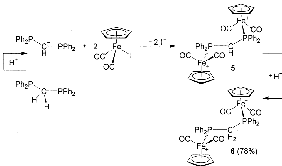
Fig. 4. Preparation of compounds 5 and 6 .
