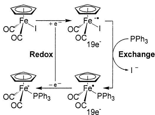
Fig. 3. Reaction of 1:1 (\eta^5\text{-C}_5\text{H}_5)\text{Fe}(\text{CO})_2\text{I}/\text{PPh}_3 in THF at -78^\circ\text{C} , after reductive initialization with a dilute lithiated reagent or (\eta^5\text{-C}_5\text{H}_5)_2\text{Co} , following the 17e–19e pathway and giving instantaneously precipitates of [(\eta^5\text{-C}_5\text{H}_5)\text{Fe}(\text{CO})_2(\text{PPh}_3)^+][\text{I}^-] , iodide being selectively replaced by \text{PPh}_3 .
