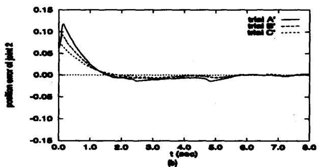
Fig. 7. Tracking error of (a) joint 1, and (b) joint 2 with admissible initial state error and measurement noise.
