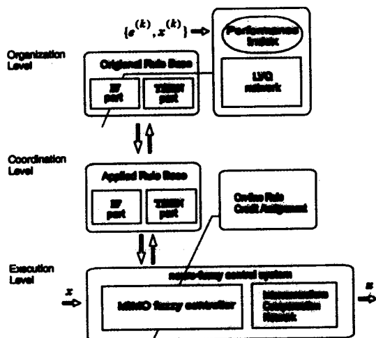
Fig. 2. Diagrammatic representation of the hierarchical SOFC.
