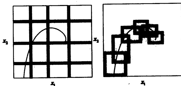
Fig. 3. (a) Regular rule partition, (b) Rule partitions depend on the trial trajectory.
