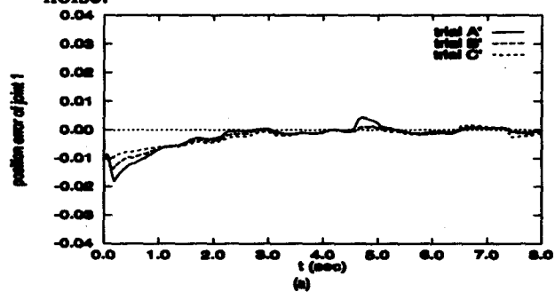
Fig. 6. Tracking error of (a) joint 1, and (b) joint 2 without initial state error and measurement noise.
