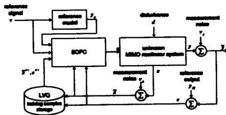
Fig. 1. A robust multi-variable tracking control system using the SOFC.
