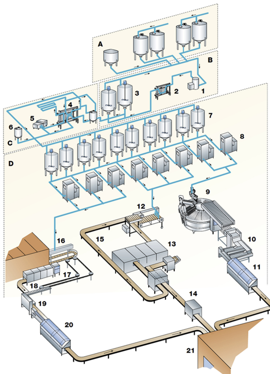
Fig. 1 – Large ice cream plant for production of 5000–10,000 L/h of various types of ice cream. Reproduced with permission from Reference [18], ©Tetra Pak.
