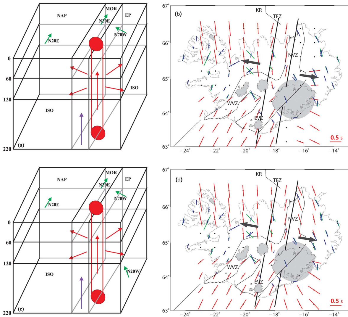
Figure 7. Same as Figure 6 but for two 3-layer models (SM4 and SM5) including a layer with radially oriented fast axes to simulate radial flow away from the plume center.
