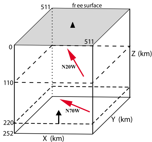
Figure 2. The geometry of the model space for the two-layer anisotropic models (bases outlined by dashed lines). Solid triangles indicate the receiver located at the free surface. The black arrow indicates the incident wave at 220 km. The red arrows show the fast directions in the top and bottom layer, respectively.
