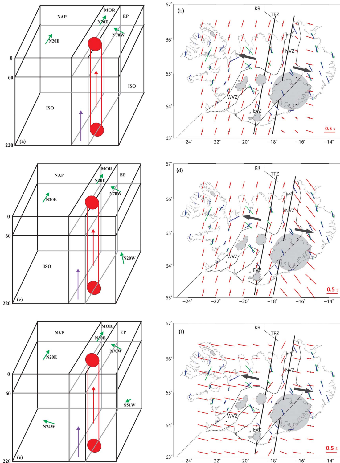
Figure 6. (a, c, and e) 3-D view of simple two-layer models (SM1, SM2 and SM3) which consider two or more basic anisotropic components and (b, d, and f) comparison of shear wave splitting results between predicted splitting parameters from the models (red bars oriented with fast direction and having length proportional to split time) and the real observations from Bjarnason et al. [2002] and Li and Detrick [2003] (blue bars) and Xue and Allen [2005] (green bars). The red cylinder represents the plume. The arrows show the assumed fast directions. The black arrows in Figures 6b, 6d, and 6f indicate the plate spreading direction. NAP, North American plate; MOR, Middle Ocean ridge; EP, Eurasian plate; ISO, isotropic.
