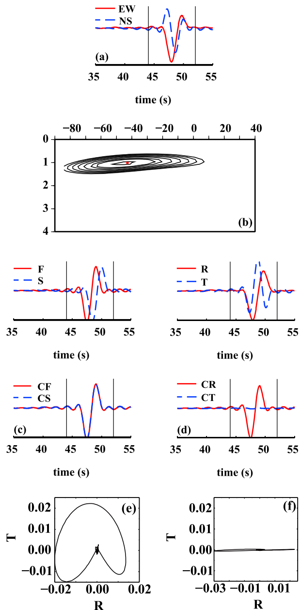
Figure 3. Splitting analysis of synthetic waveforms with a dominant period of 4 s and initial polarization of E-W from the two-layer anisotropic model shown in Figure 2. (a) Original waveforms of N-S and E-W components. (b) Contours of residual tangential energy are used to identify the optimum splitting parameters (red dot) in the fast direction and delay time space. The smallest contour indicates the 95% confidence level. (c) (top) Original and (bottom) corrected fast and slow components of motion. (d) (top) Original and (bottom) corrected radial and transverse components. (e) Original horizontal particle motion. (f) Corrected horizontal particle motion.
