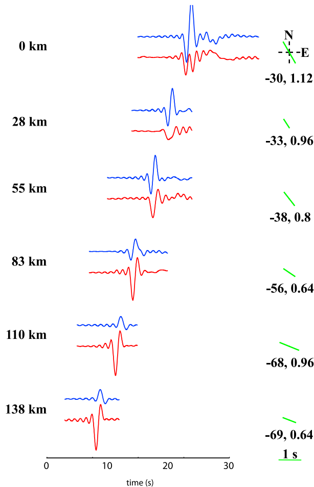
Figure 4. Synthetic waveforms on radial (red) and transverse (blue) components at a variety of depths and correspondent shear wave splitting results (green bars) from the two-layer anisotropic model. Fast direction is the first number on right in degrees and delay time is the second number in s. The orientation and length of the green bar indicate the fast direction and delay time, respectively.
