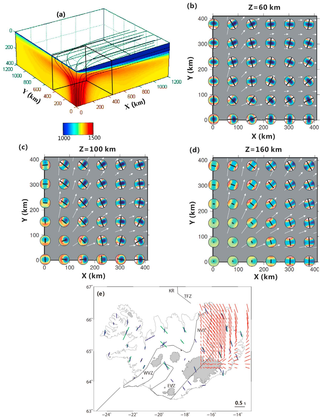
Figure 9. (a–d) The same as Figure 8 but for more realistic plume flow beneath a plate spreading at a half rate of 10 km/Myr (GM2). (e) SWS predicted at the surface (red) compared to those observed (as in Figure 8).
