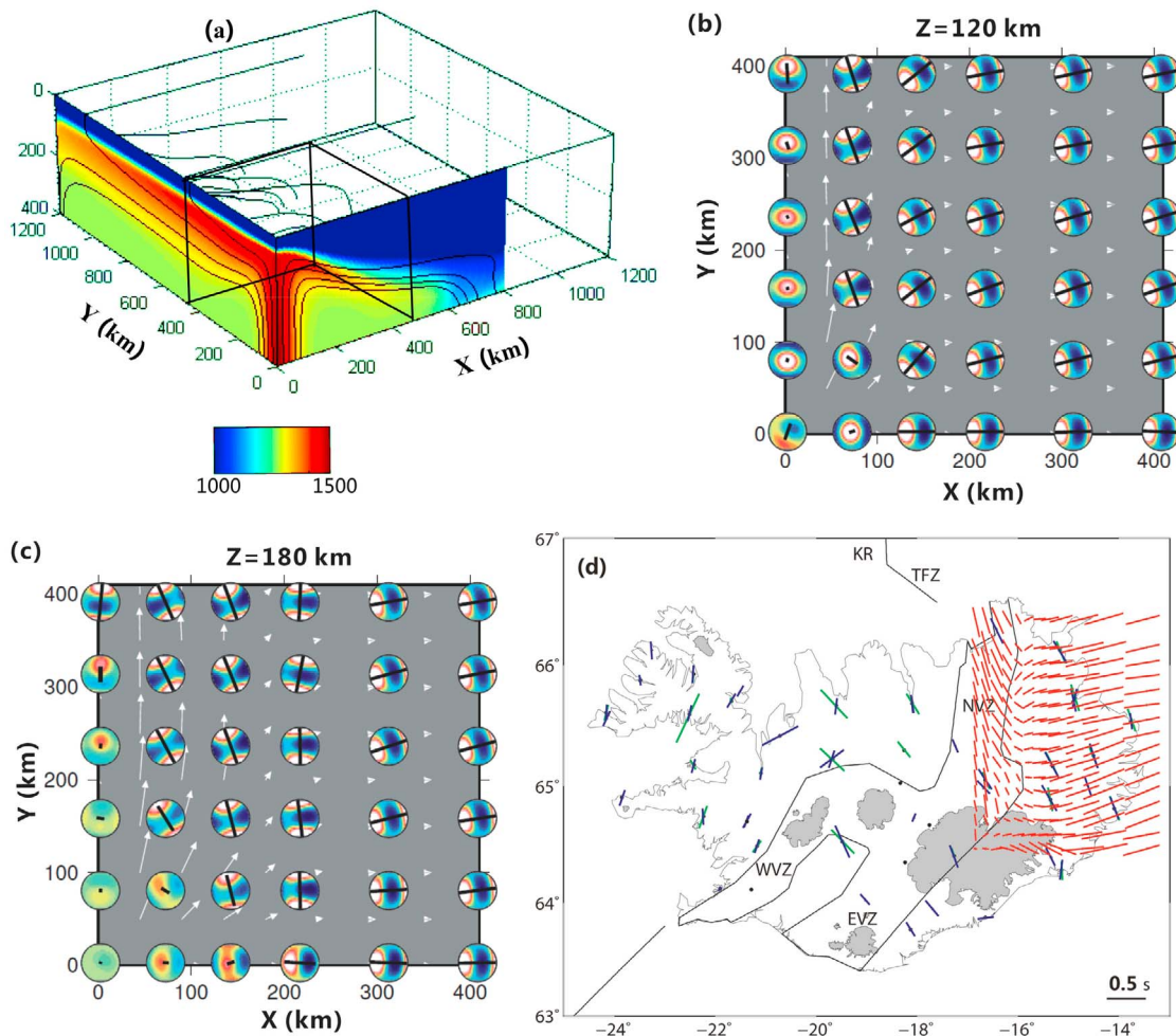
Figure 10. Same as Figure 9 but for channel flow model with unrealistic spreading rate of 1 km/Myr (GM3) and predicted anisotropy shown at two depths.
