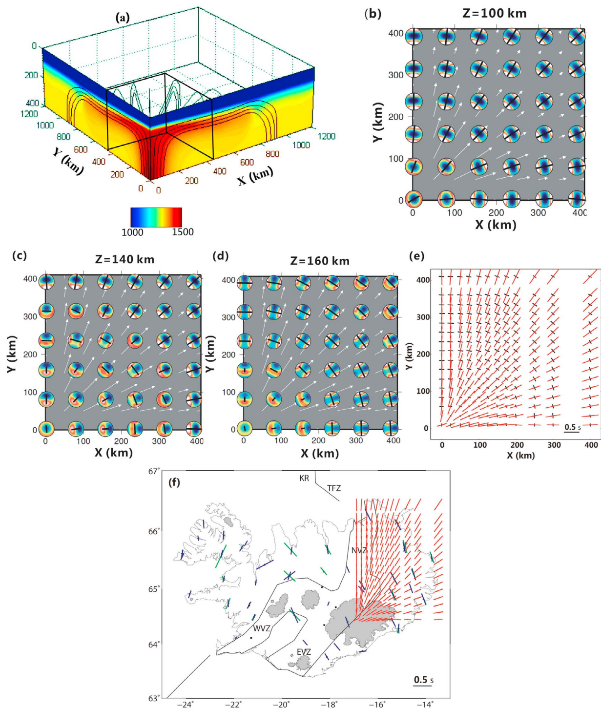
Figure 8. Perspective view of geodynamic models that simulate purely axis symmetric flow away from the plume beneath a stationary plate (GM1). (a) Model geometry. Potential temperature in °C is colored and mantle flow trajectories are shown with black lines. (b–d) Predictions of seismic anisotropy at three depths. Arrows show horizontal components of flow with length proportional to flow speed. Circles are outer hemisphere plots of the directional dependence of V_p (colors: white is fast, blue is slow). Bold bar shows the direction of the fastest V_p , which corresponds to the preferential alignment of the olivine \alpha -axes. (e) SWS parameters obtained from the wave propagating from a depth 200 km to a depth of 140 km (black) and to the surface (red). (f) Comparison between the predicted shear wave splitting parameters at the surface (red bars) and real observations from Bjarnason et al. [2002] and Li and Detrick [2003] (blue bars) and Xue and Allen [2005] (green bars) in eastern Iceland.
