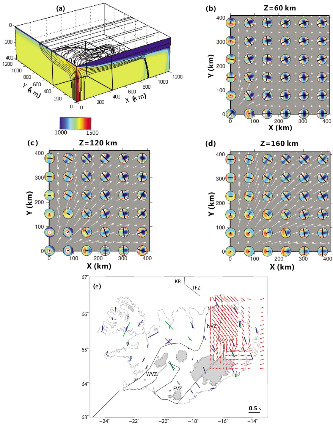
Figure 11. Same as Figure 9 but for channel flow model with realistic spreading rate of 10 km/Myr (GM4).
