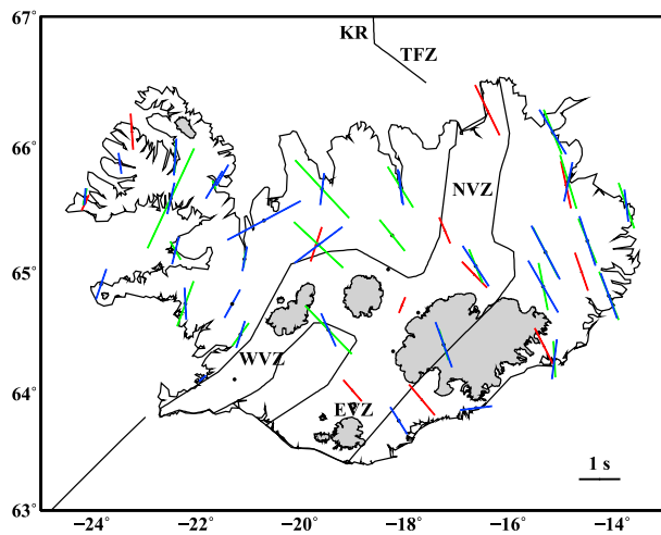
Figure 1. Tectonic map of Iceland. Thick black lines outline the volcanic zones in Iceland and ridge segments in the Atlantic. Shaded areas mark the locations of major icecaps. The Iceland hot spot is currently centered beneath the largest icecap in southeast. Splitting parameters are shown as blue bars at the ICEMELT stations from Bjarnason et al. [2002], red bars at the HOT SPOT stations from Li and Detrick [2003], and green bars at the HOT SPOT and SIL stations from Xue and Allen [2005]. WVZ, Western Volcanic Zone; EVZ, Eastern Volcanic Zone; NVZ, Northern Volcanic Zone; RR, Reykjanes Ridge; KR, Kolbeinsey Ridge; TFZ, Tjornes Fracture Zone.
