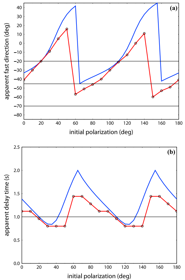
Figure 5. Predicted apparent (a) fast direction and (b) delay time as a function of incoming polarization direction. Black lines are the fast directions of the top ( -20^\circ ) and bottom ( -70^\circ ) layer and the delay time for each layer (both 1 s). Red lines are the splitting parameters from the full waveform method; blue lines are from the analytic solution.
