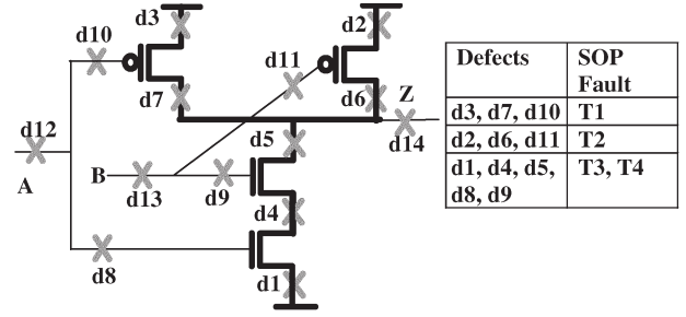
Fig. 3. Fourteen open-defect locations (d1–d14) of NAND.
