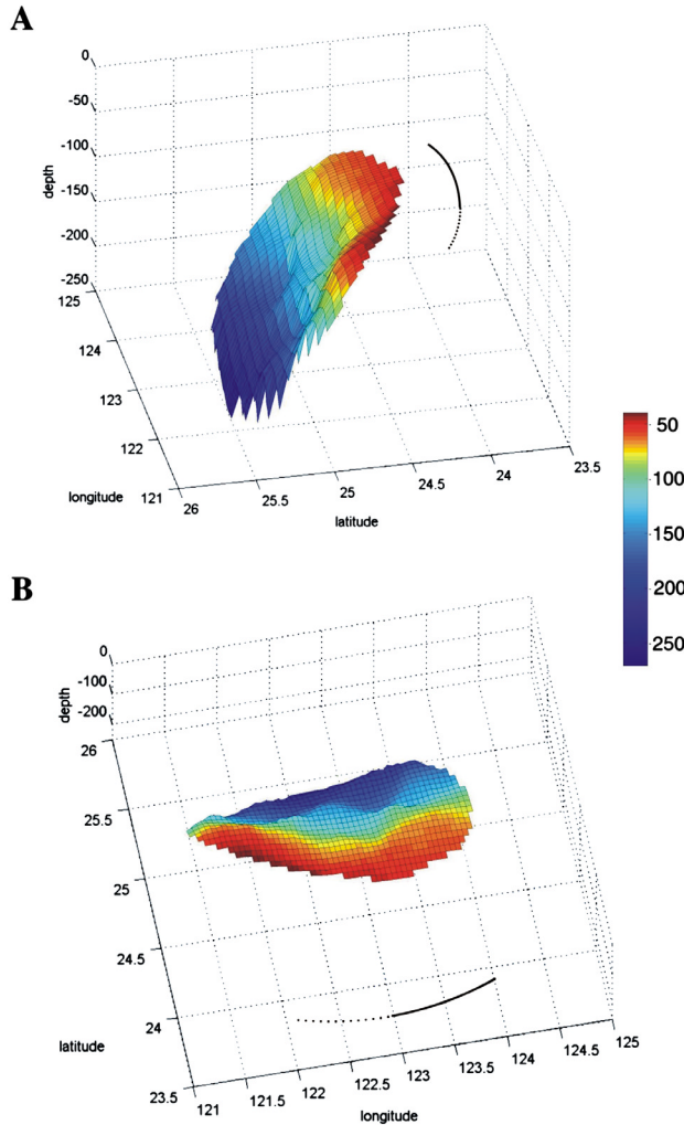
Figure 4. The 3-D slab surface model fit using GOCAD software, shown in two different perspectives. (a) From northwest to see the face of the slab. The folding over the western section creates a bulge at intermediate depths that leads to a greater dip angle of the slab below. (b) A look that grazes along the surface of the slab from south to north subparallel to the slab dip. In both Figures 4a and 4b, folding near the western boundary is evident in comparison with the trace of the trench (solid and dotted lines in Figures 4a and 4b).
