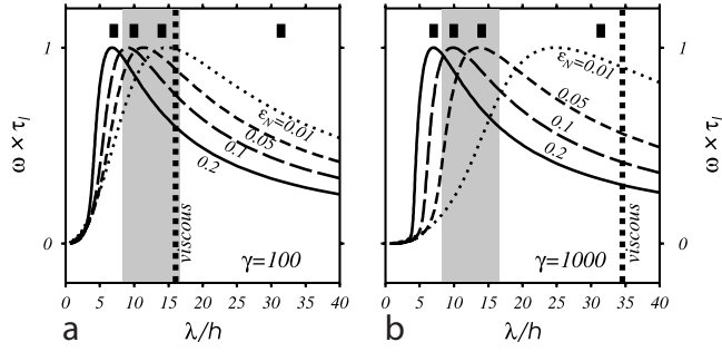
Figure 6. Predicted nondimensionalized amplification \omega_1 \times \tau_I as a function of wavelength for (a) \gamma = 100 and (b) \gamma = 1000 and for the elastic strain \varepsilon_N = 0.01 (dotted lines), 0.05 (short dashed lines), 0.1 (long dashed lines), and 0.2 (solid lines). The amplification functions are normalized to 1. The dominant wavelength for a viscous layer (vertical dotted line) is a function of \gamma only, and is approximated by the viscoelastic layer at small \varepsilon_N . The dominant wavelength of an elastic buckling is a function of \varepsilon_N , indicated by the short vertical bars near the top of Figures 6a and 6b for \varepsilon_N = 0.2, 0.1, 0.05 , and 0.01 from left to right. Pure viscous folding barely explains the observation (shaded region) with \gamma = 100 (or smaller), and a pure elastic slab requires strain >0.04 . Both are inadequate in explaining the status of stress of the slab.
