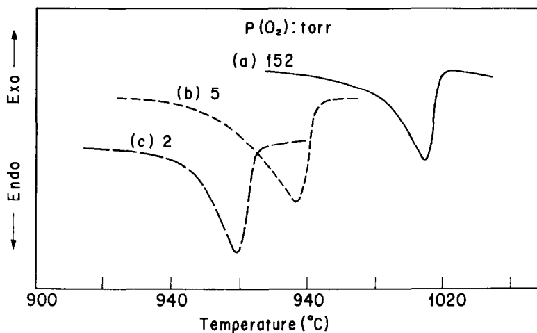
Fig. 2. Effect of oxygen pressure on the melting of 123 oxide. DTA curves of 123 samples at a heating rate of 1^\circ\text{C min}^{-1} under an oxygen pressure, P(\text{O}_2) , of: (a), 152 Torr; (b), 5 Torr; and (c), 2 Torr.
