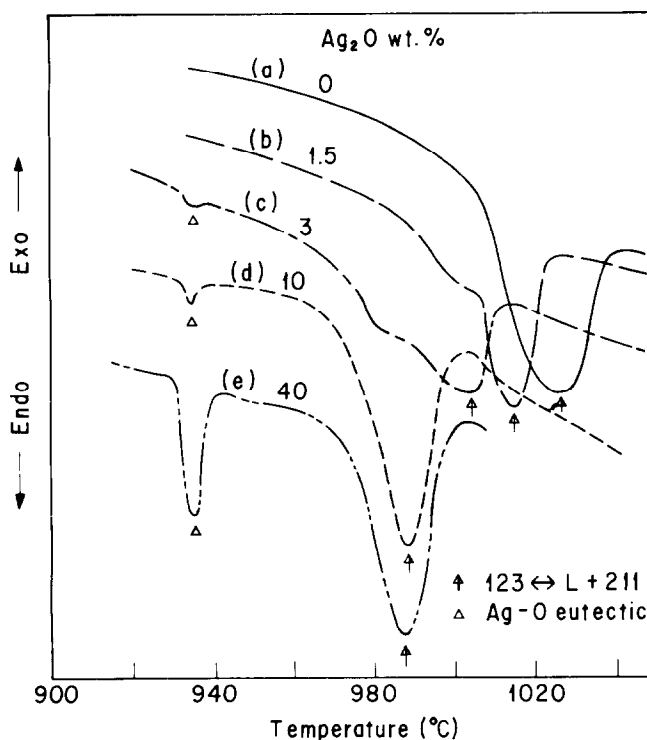
Fig. 1. Effect of Ag on the melting of 123 oxide. DTA curves of 123/Ag samples containing: (a), 0; (b), 1.5; (c), 3.0; (d), 10.0; and (e) 40.0 wt% \text{Ag}_2\text{O} , at a heating rate of 10^\circ\text{C min}^{-1} in air.
