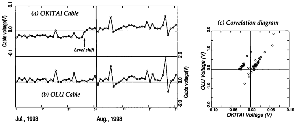
Fig.6 Abrupt voltage change in the cable data. (a) An abrupt voltage change in OKITAI cable data, marked by 'level shift', in July 1998. (b) OLU cable data with no abrupt voltage change. (c) Correlation diagram between OKITAI and OLU voltages using daily mean voltages in two months around the abrupt voltage change.
