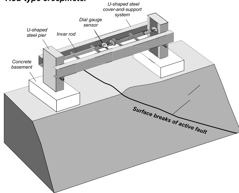
Figure 5. Schematic representation of the rod-type creep meter across an active fault, rupturing the concrete wall on the surface. For a description of the instrumentation, see the text.
