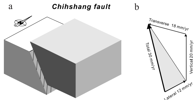
Figure 3. 3-D schematic reconstruction of the Longitudinal Valley Fault. (a) Illustration of oblique slip, showing the reverse and left-lateral components of motion. (b) Quantification of present-day fault slip components, based on fault geometry (strike and dip) and results of geodetic surveys near Chihshang.
