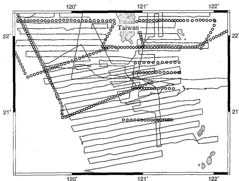
Fig. 3. Tracks of 1990 6-channel seismic data (solid lines) (after Reed et al. , 1992) and 120-channel seismic data associated with TAICRUST (dotted lines).
