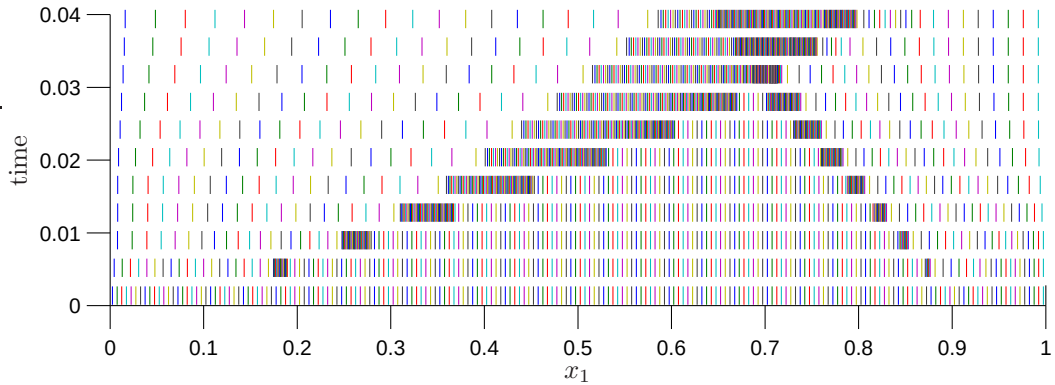
Figure 7: Physical grid coordinates for the generalized Lagrangian run shown in Fig. 6 at eleven different times t = i \times 0.0038 , for i = 0, 1, \dots, 10 . Here the grid system is displayed in the same manner as in Fig. 5.
