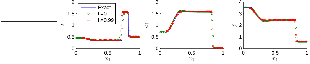
Figure 4: Numerical results for a two-component Lax Riemann problem at time t = 0.14 . The solid line is the exact solution, and the dotted and triangular points are the computed solutions obtained using two different grid-movement parameters h = 0 and h = 0.99 , respectively, with a 100 mesh points.
