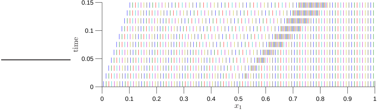
Figure 5: Physical grid coordinates for the generalized Lagrangian run shown in Fig. 4 at eleven different times t = i \times 0.014 , for i = 0, 1, \dots, 10 . Each little dashed line displayed in the graph gives a cell-center location of the grid system at a specific output time.
