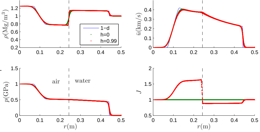
Figure 11: Scatter plots of the results for the run shown in Fig. 10. The solid line is the “true” solution obtained from solving the one-dimensional model with appropriate source terms for the radial symmetry using the high-resolution method and 1200 mesh points. The dotted and triangular points are the two-dimensional results obtained using h = 0 and 0.99 , respectively. The dashed line is the approximate location of the air-water interface.
