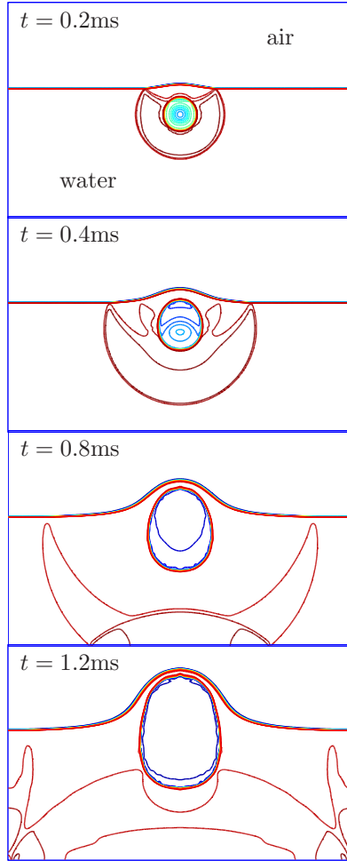
Figure 12: Numerical results for the simulation of a model underwater explosion problem. Contour plots are shown for (a) the density (30 lines range from 18.6 to 1137.2 kg/m 3 ), and (b) the pressure (30 lines range from 6.43 to 392.18MPa) at four different times t = 0.2, 0.4, 0.8 , and 1.2ms obtained using both h = 0 and 0.95 with a 400 \times 250 grid.
