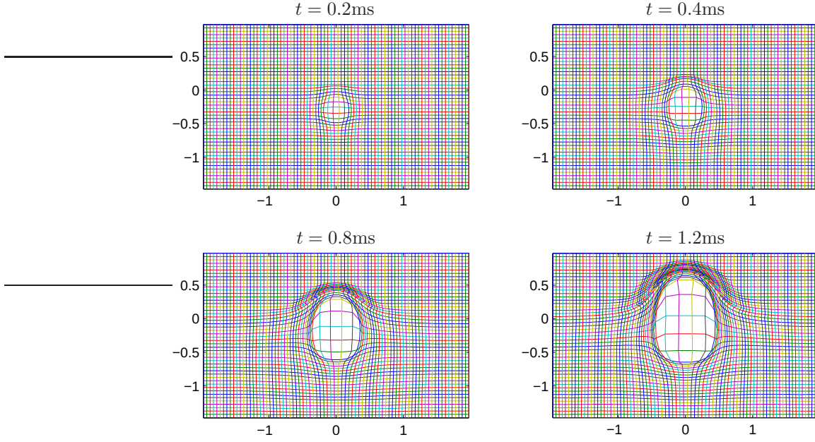
Figure 13: Physical grid system for the generalized Lagrangian run with h = 0.95 shown in Fig. 12. For clarity, a grid coarsening factor of 5 in each x_1 - and x_2 -direction is used to make each of the graphs.
