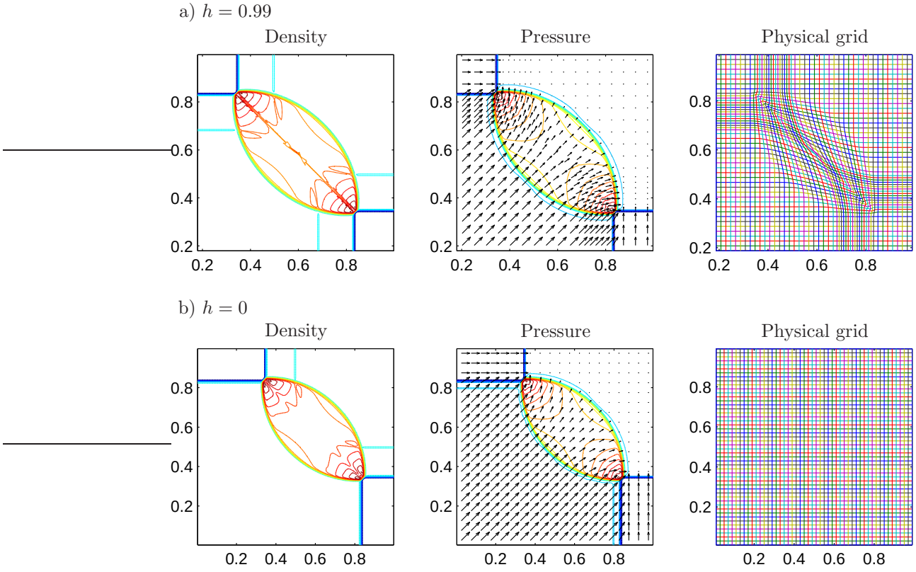
Figure 8: Numerical results for a two-dimensional Riemann problem, a 4-shocks initial condition case. Contour plots of the density and pressure (30 lines range from 0.033 to 1.998 and 0.044 to 2.685, respectively), and the physical grid coordinates are shown at time t = 0.2 obtained using both h = 0 and 0.99 with a 200 \times 200 grid. Note that the computed velocity field is superimposed into the pressure contours. For clarity, solution coarsening factors of 10 and 4 in each x_1 - and x_2 -direction are used to graph the velocity vectors and the physical grid system, respectively.
