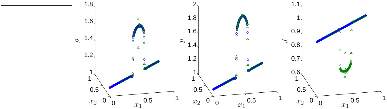
Figure 9: Cross-sectional plots of the results for the shown shown in Fig. 8 along the diagonal axis of the computational grid. The dotted and triangular points are the numerical solutions obtained using h = 0 and 0.99, respectively.
