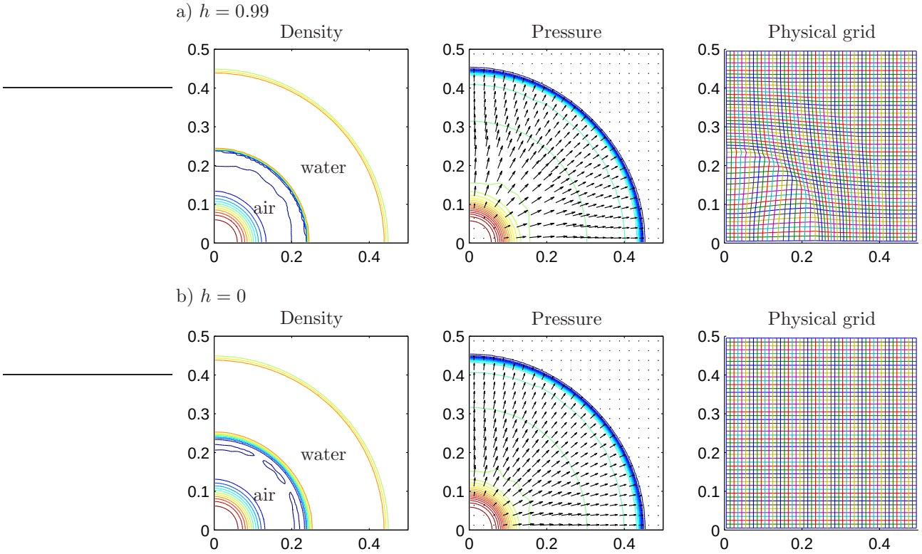
Figure 10: Numerical results for a two-component radially symmetric problem at time t = 120\mu\text{s} with a 100 \times 100 grid. Here the solutions are plotted in the same manner as in Fig. 8 with the contours ranging from 20.8 to 1270.8 \text{kg/m}^3 and 16.7 to 1016MPa, for the density and pressure, respectively.
